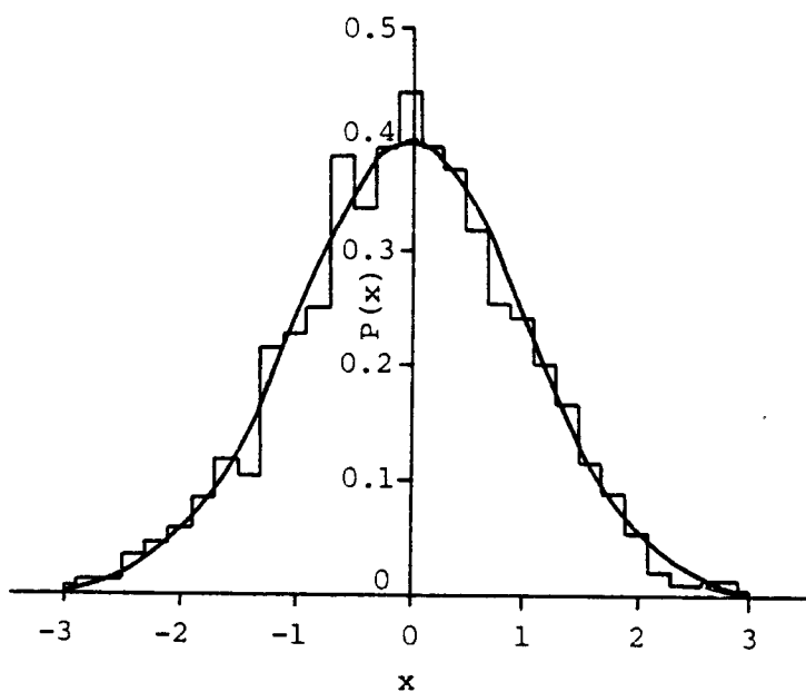
Figure 4-3. Probability density function of the data set used in Figure 4-2, computed with \Delta x = 0.2 .
