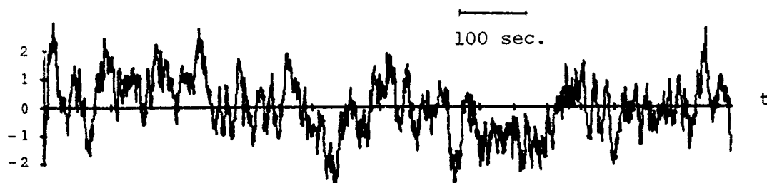
(b) Lateral component of Dryden spectrum model
