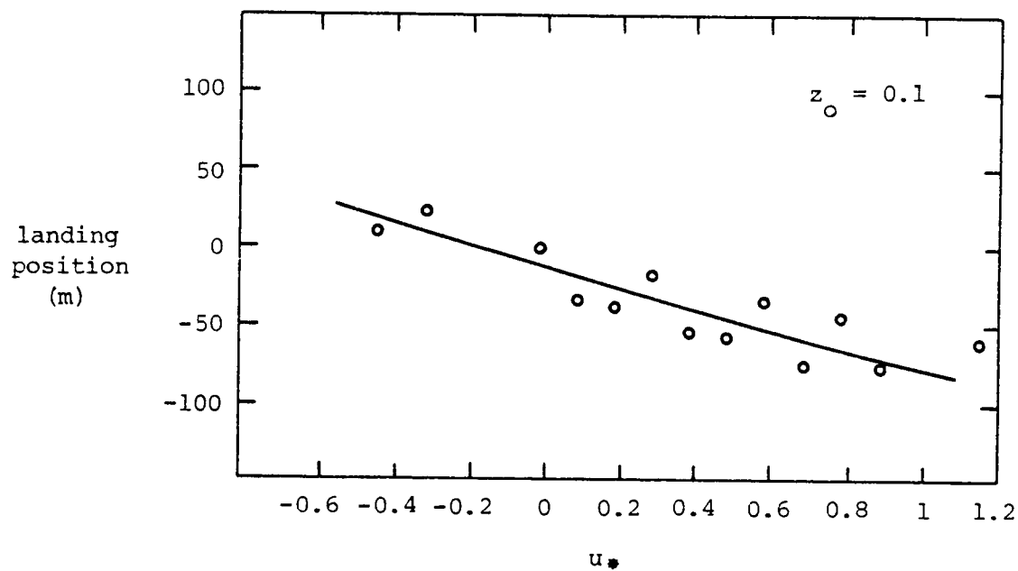
Figure 5-3. The landing position for different values of u_* with no turbulence.
