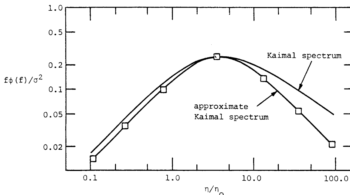
Figure 2-6. The Kaimal spectrum, Equation (2-12), compared with the approximation form, Equation (2-20).
