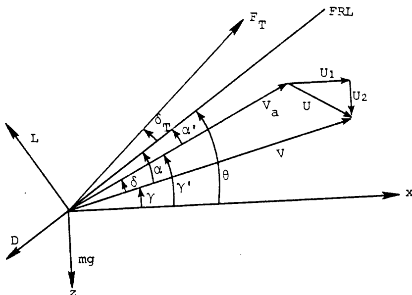
Figure C-1. The forces acting on the aircraft.
