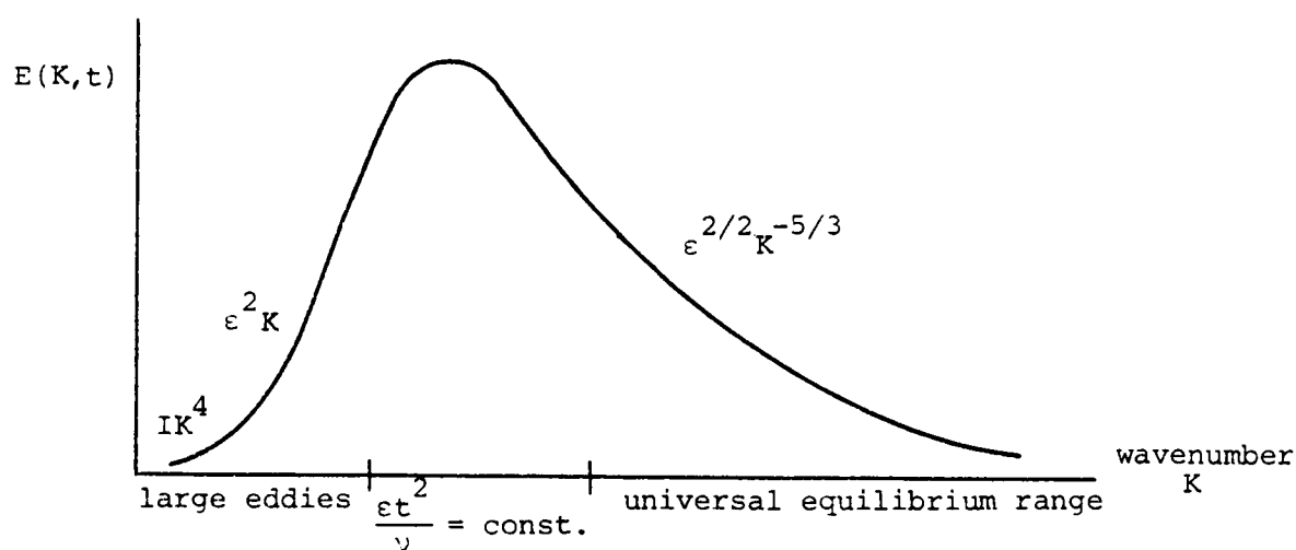
Figure 2-1. Typical three-dimensional energy spectrum function [4].
