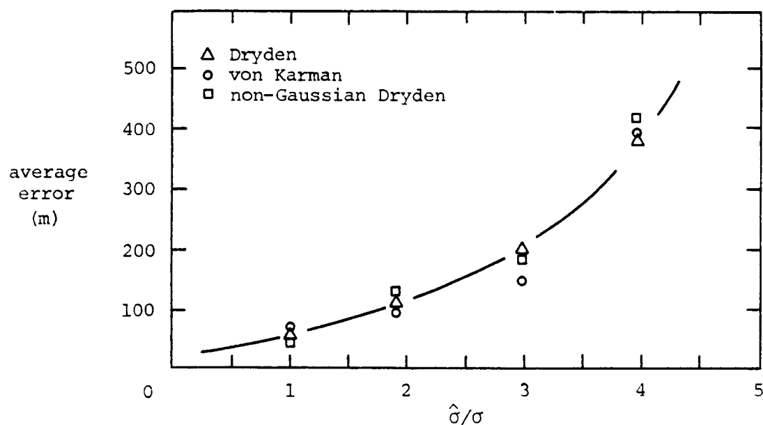
Figure 5-5. The average landing error for different turbulence models ( u_* = 0.5 , z_0 = 0.1 ).
