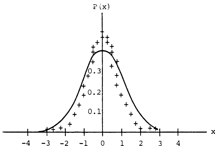
Figure 2-9. Comparison of the Gaussian distribution with measured gust velocity distribution [10].
