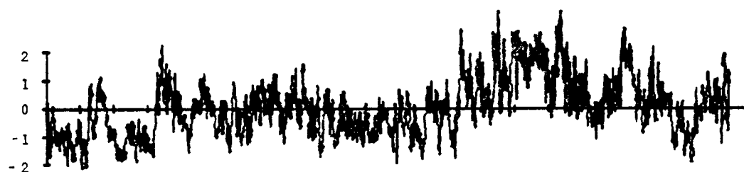
(a) Measured atmospheric turbulence ( z = 24 m)
