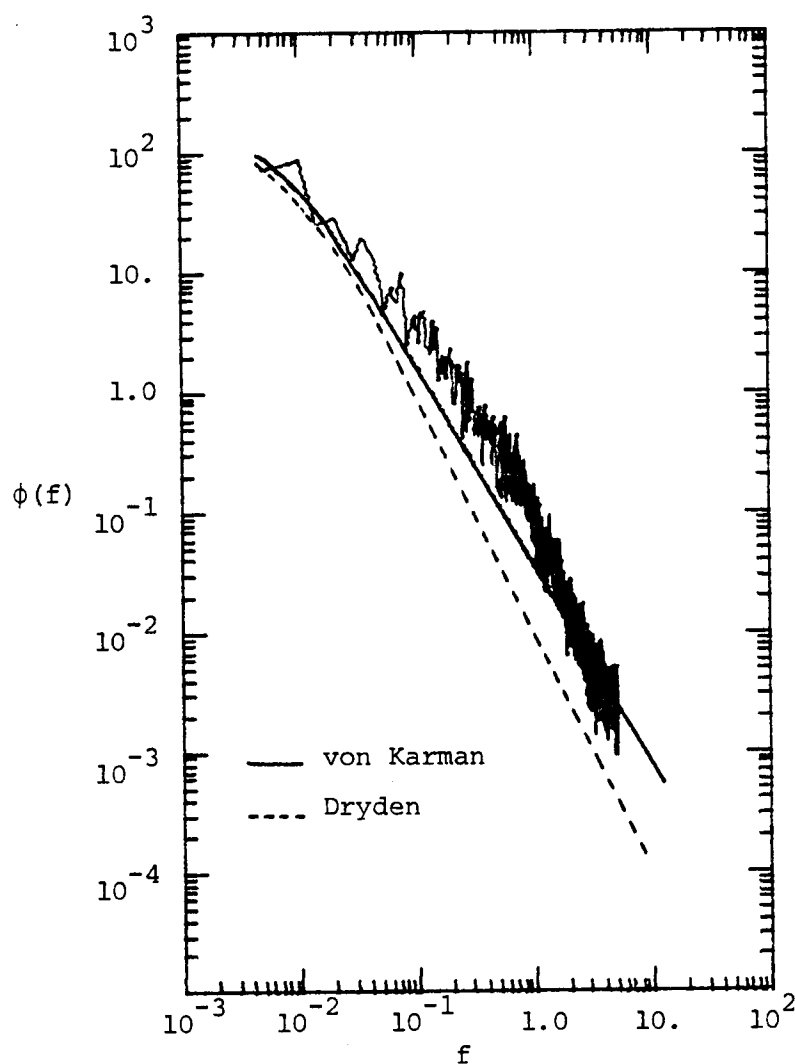
Figure 4-16. Comparison of two theoretical curves with the calculated spectrum of measured atmospheric turbulence ( z = 24 m, \Delta t = 0.5 , N = 2048 ).
