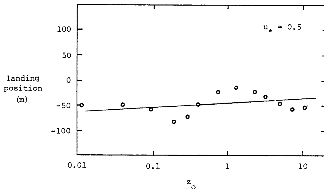
Figure 5-4. The landing position for different values of z_0 .
