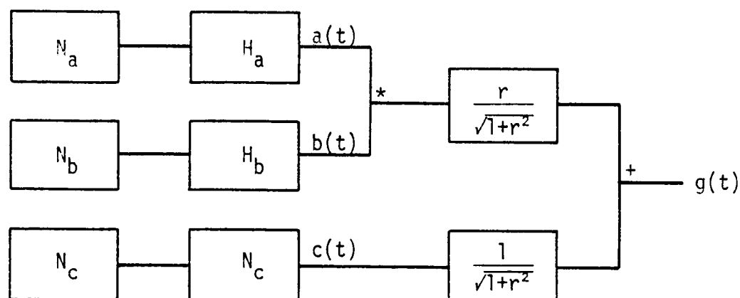
Figure 2-8. The non-Gaussian multi-filter system.
