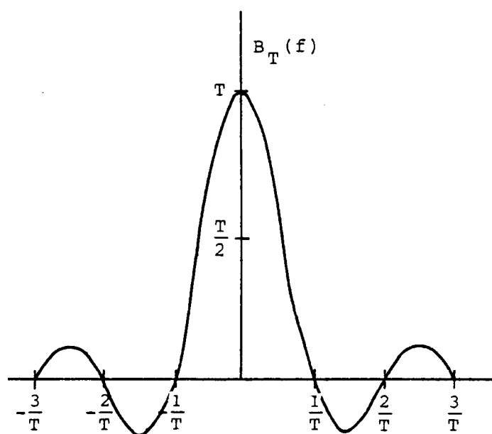
Figure 3-4. The spectral window for boxcar weighting function.
