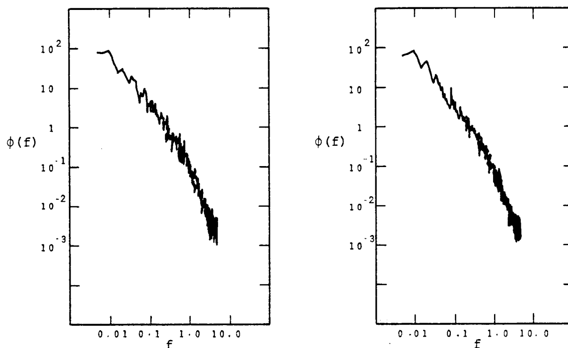
(b) Measured atmospheric turbulence at z equal to 24 m and 12 m, respectively ( \Delta t = 0.5 )
