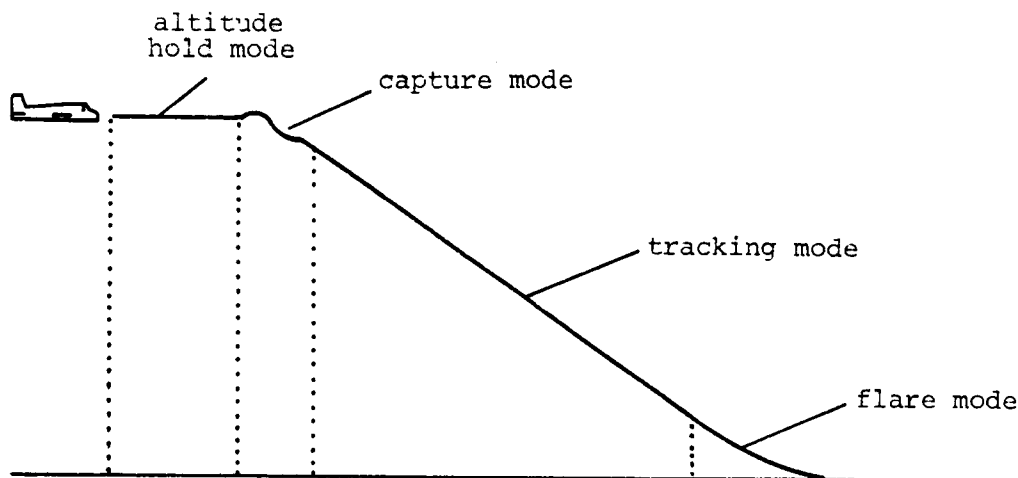
Figure 5-1. Automatic landing control modes.
