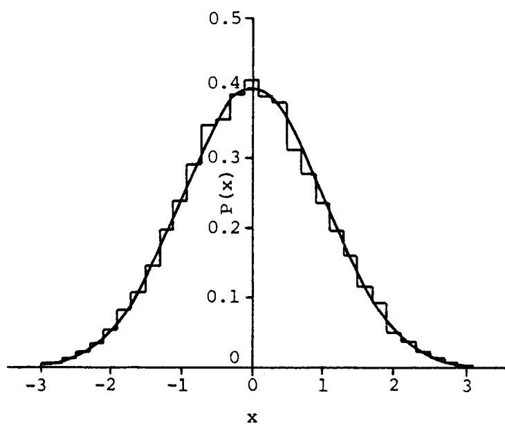
Figure 4-4. Probability density function computed with total 20480 datum points ( \Delta x = 0.2 ).
