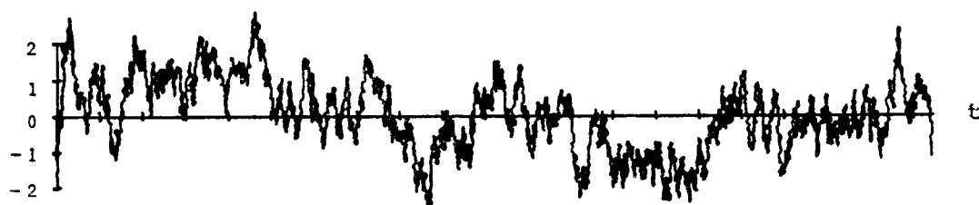
(a) Longitudinal component of Dryden spectrum model
