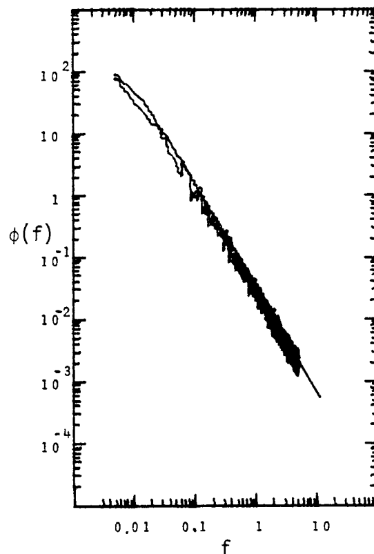
(b) Kaimal spectral model
