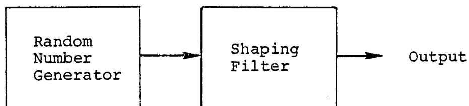
Figure 1-1. Turbulence simulation system.
