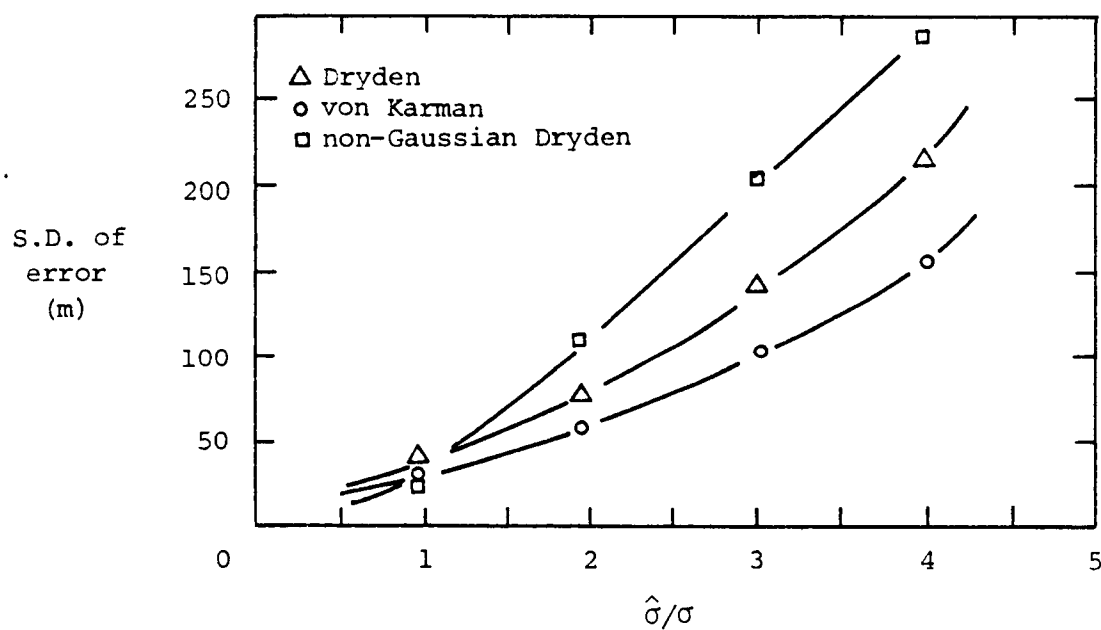
Figure 5-6. The standard deviation of error for different turbulence models ( u_* = 0.5 , z_0 = 0.1 ).
