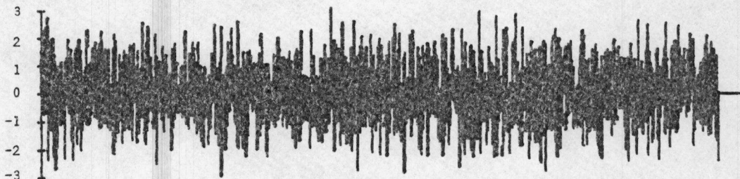
Figure 4-1. Gaussian distributed random signals with zero mean and unity standard deviation (2048 data).
