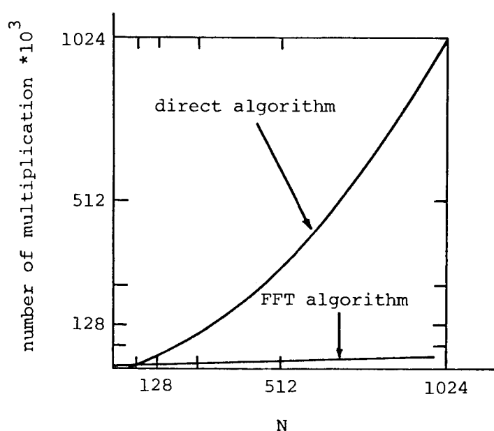
Figure 3-3. Comparison of the number of multiplications required for a Fourier transform by the direct algorithm and the FFT algorithm.
