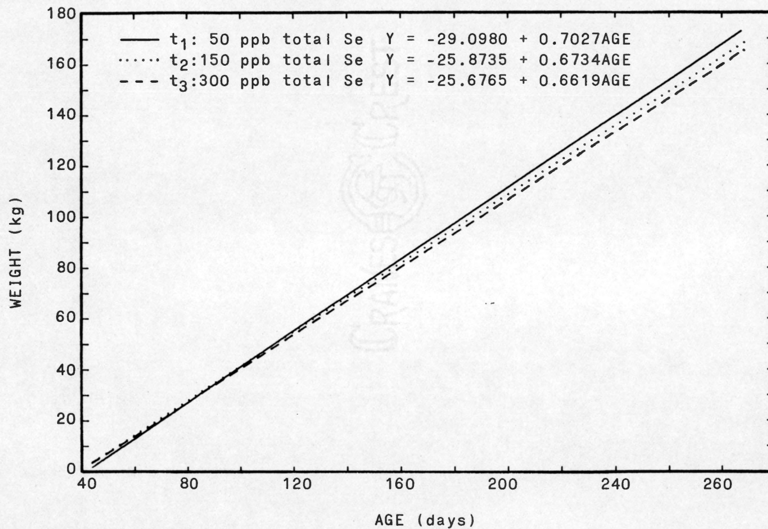
Figure 1. Relationship between the linear regressions of the weight (kg) of boars receiving three levels of dietary selenium (Se) over age (days). Treatments 1, 2 and 3 received 50, 150 and 300 ppb selenium (from sodium selenite), respectively.
