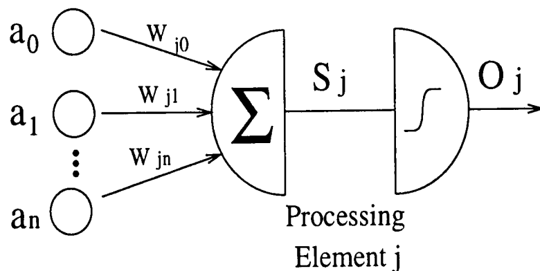
Figure 2.1: Basic Components of a PDP System
