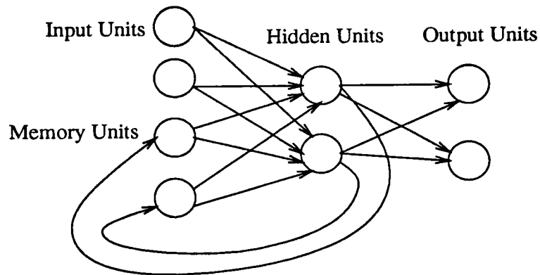
Figure 2.3: A Sequential Recurrent Network
