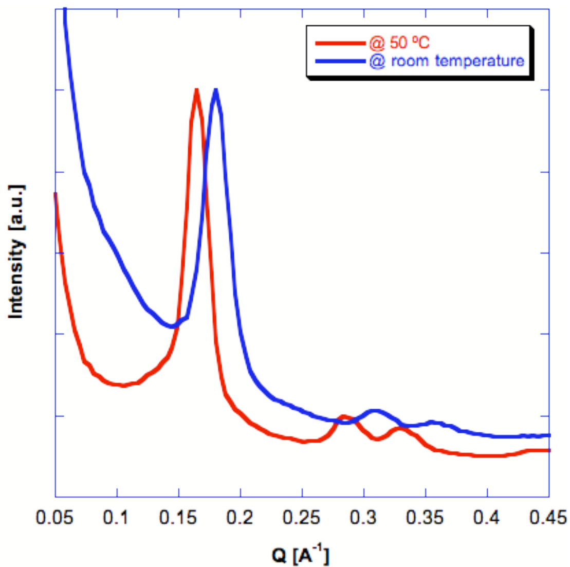
Figure 5-13 SAXS patterns of of mesoporous silica particle synthesized at different temperatures. Using the 6:1 TEOS:CTAB, red line synthesized at 50 °C and blue line at room temperature.
