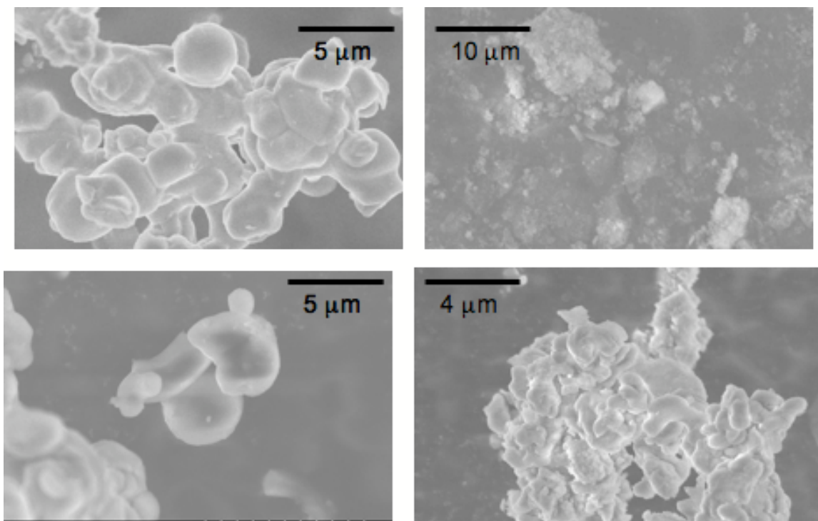
Figure 5-6 SEM images of silica particles synthesized at pH > 12.5.
