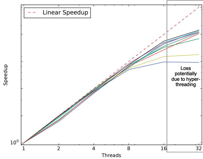
Figure 2.4: Scaling on various problems
