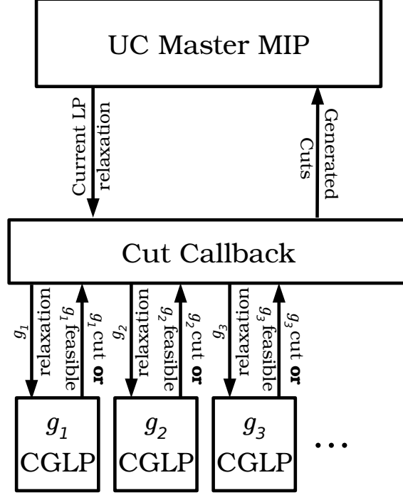
Figure 3.1: Visualization of the cut-generation procedure
