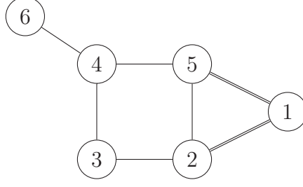
Figure 2.2: FIXEDDEGELIM example: Edges (1,2) and (1,5) are fixed
