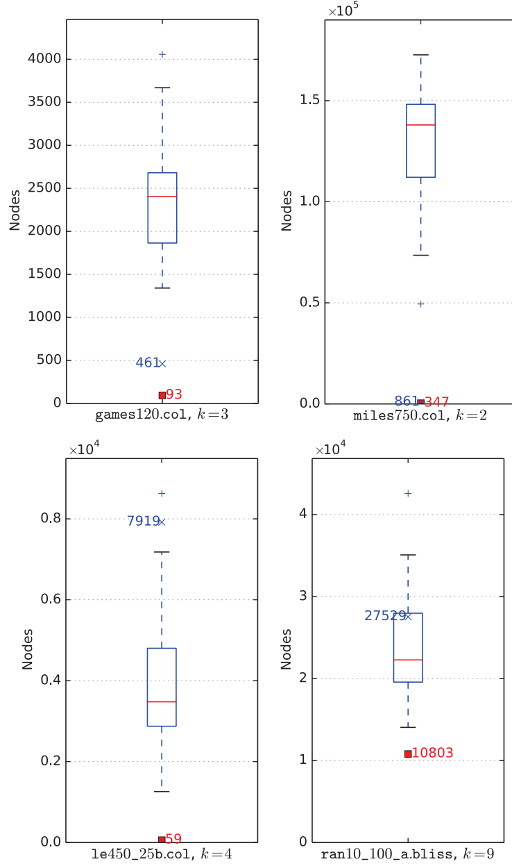
Figure 2.5: Random branching (box plot) vs. edgeUse branching (■, number of nodes on right) vs. local branching (×, number of nodes on left), selected instances
