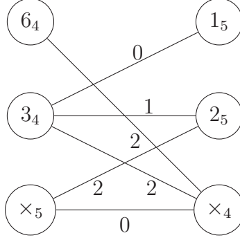
Figure 2.3: REFINEBYMATCHING example: Edges with weight +\infty have been excluded for clarity.
