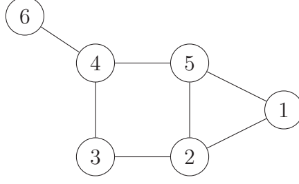
Figure 2.1: A graph with almost symmetry
