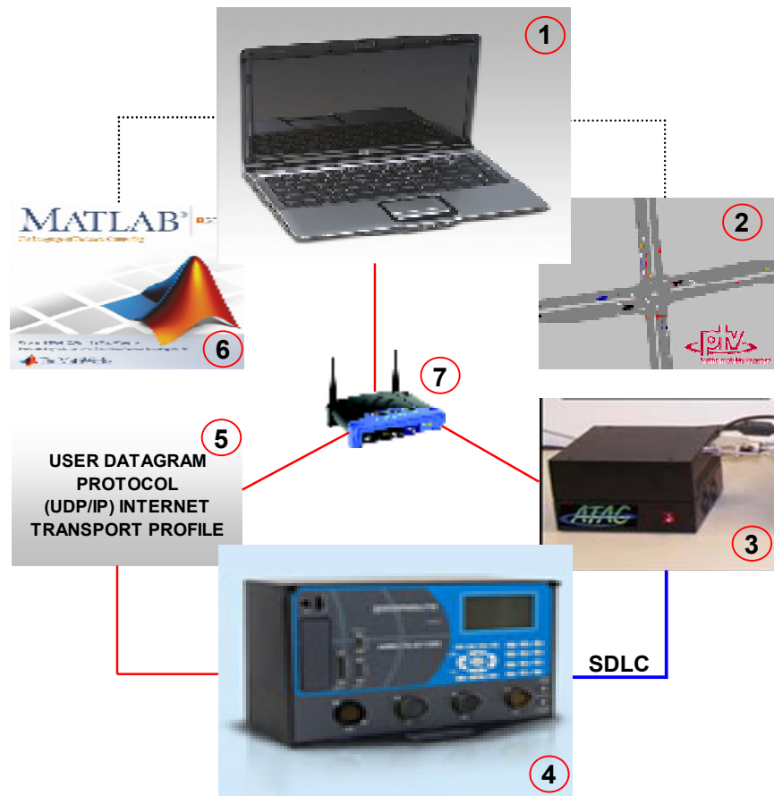
Figure 1 - System architecture for a hardware-in-the-loop simulation (1-Computer, 2-Traffic Simulator, 3-Controller Interface Device, 4-Traffic Signal Controller, 5-Communication Protocol, 6-Algorithm Software, 7-Ethernet Connection Provider)
