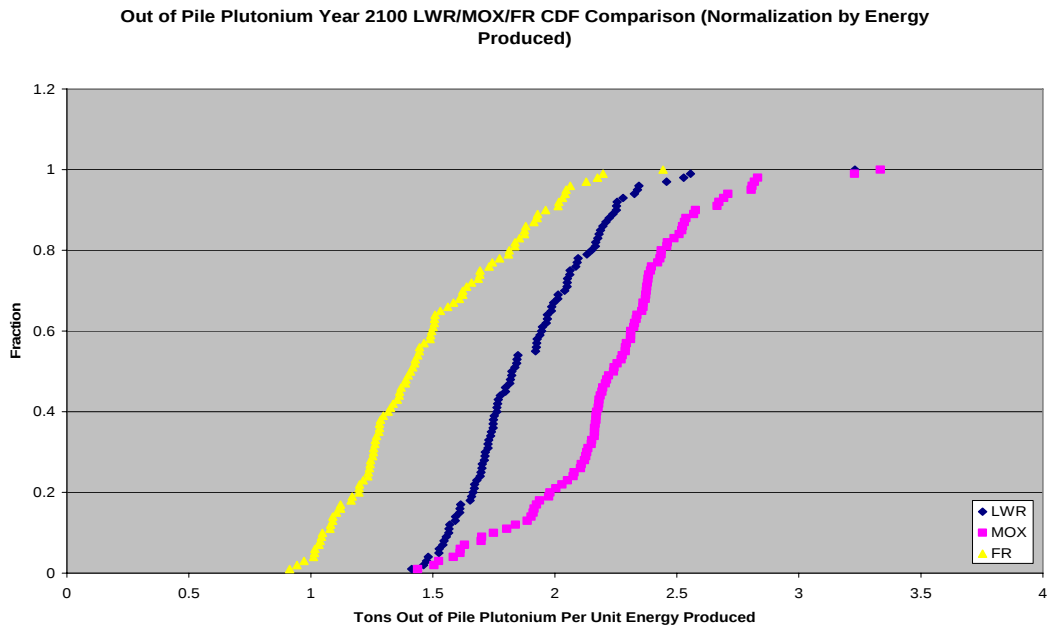
Figure 3.32 Sample Comparison CDF of Results Normalized Over Energy Produced. Pu Out-of-Pile year 2100
