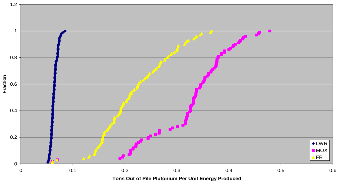
In Pile Plutonium Year 2050 LWR/MOX/FR CDF Comparison (Normalization by Energy Produced)
