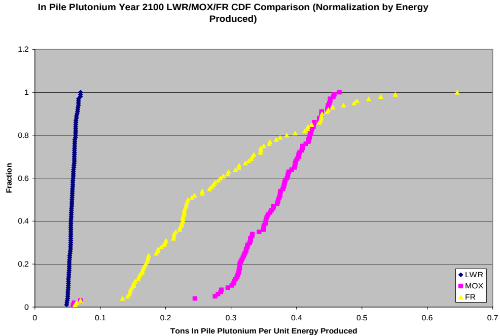
Figure 3.31 Sample Comparison CDF of Results Normalized Over Energy Produced. Pu In-Pile year 2100
