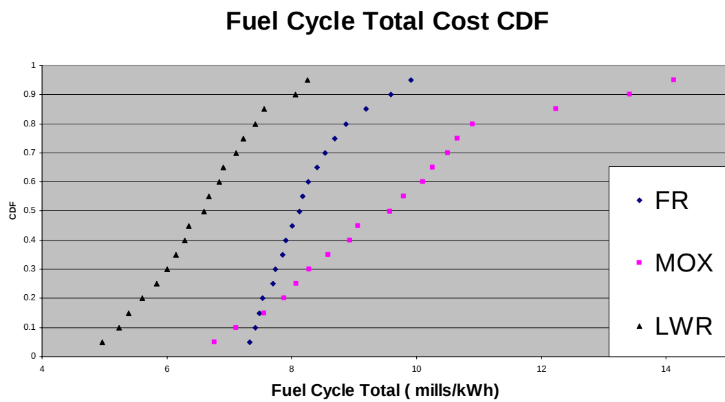
Figure 3.33 CDF of Fuel Cycle Total Cost in mills/kWh
