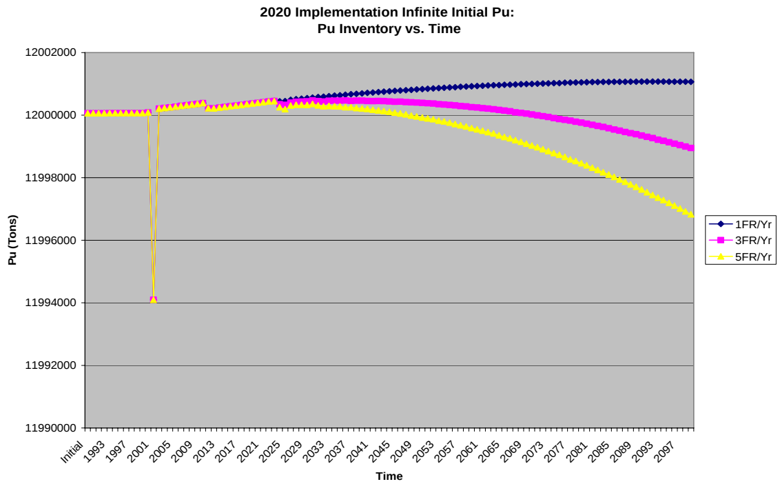
Figure 3.7 2020 Implementation Infinite Initial Pu: Pu Inventory vs. Time
