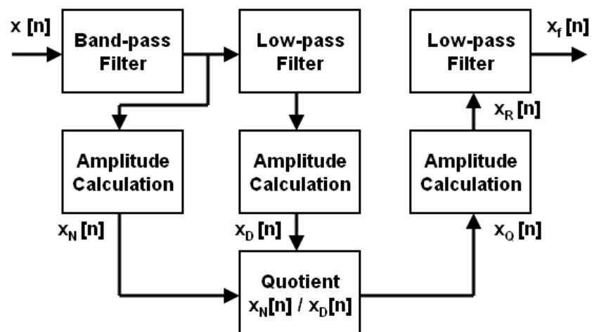
Figure 4.9. Sezi method frequency measurement algorithm [31]
