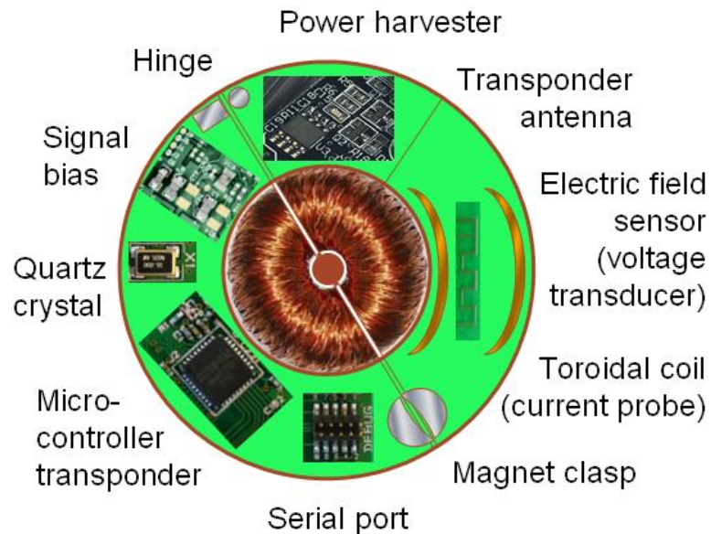
Figure 4.1. Author’s concept PMU (complete system is 1.3” diameter disk)
