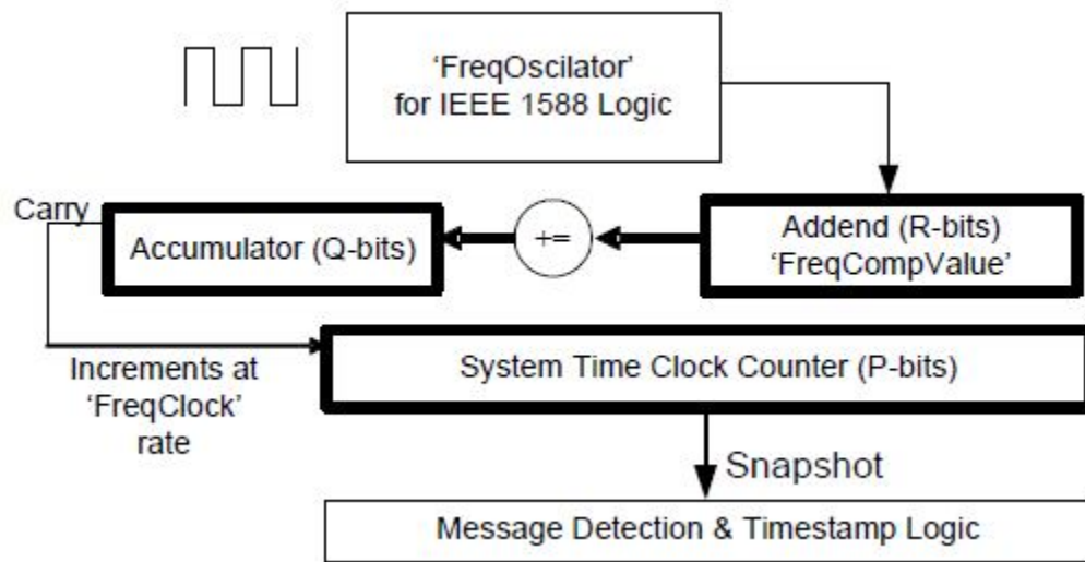
Figure 4.7. Frequency compensated clock logic [28]
