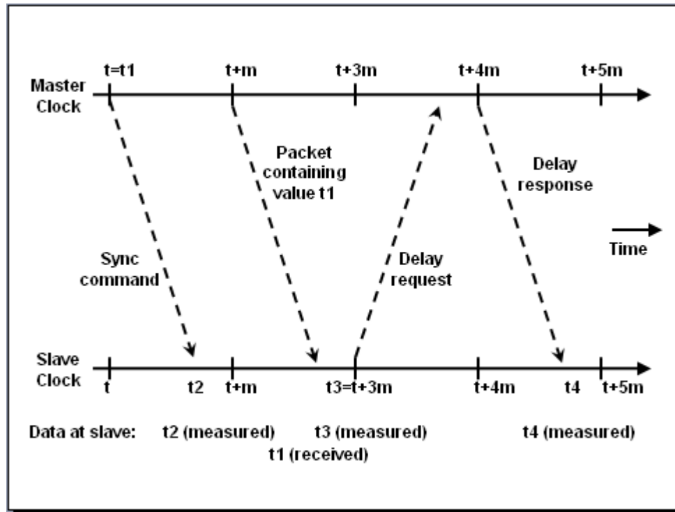
Figure 4.6. Synchronization of IEEE 1588 slave to master clock time [26]
