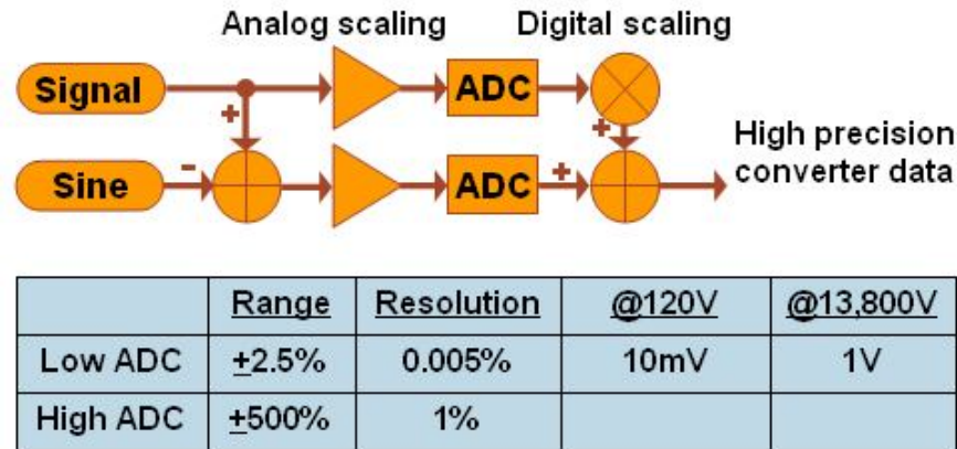
Figure 4.4. Author's proposed tracking ADC for high precision sampling
