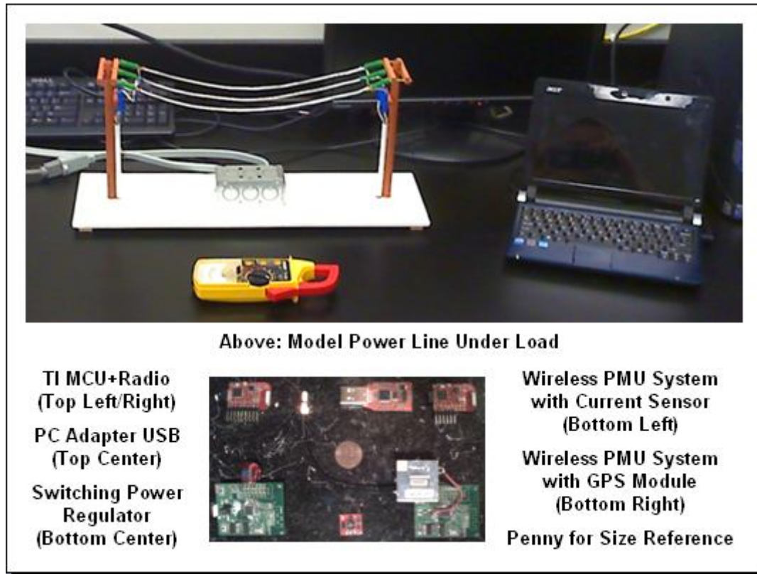
Figure 4.3. Author's hardware prototype and model power line
