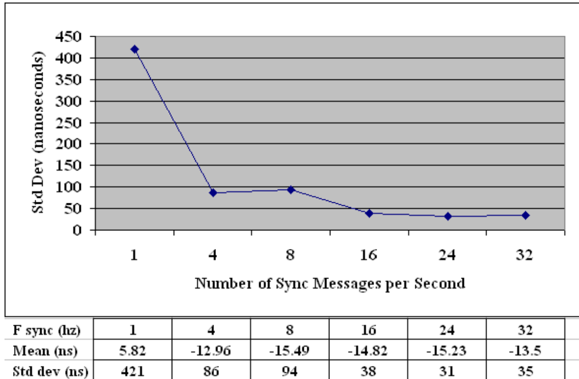
Figure 4.8. Time synchronization for various sync message rates [30]
