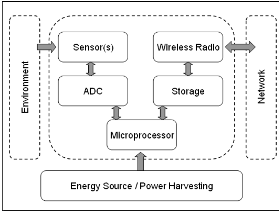
Figure 2.2. Typical architecture of a wireless sensor node [11]
