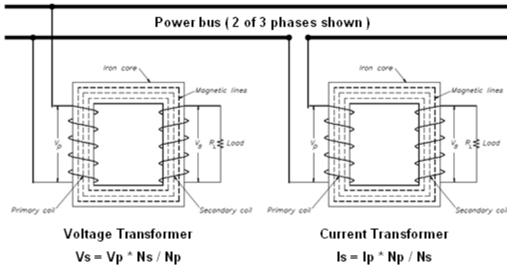
Figure 3.1. Illustration of existing instrument transducer technology
