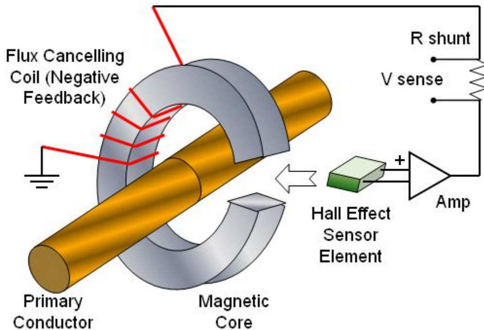
Figure 4.5. Basic topology of closed loop Hall Effect current sensor [22]
