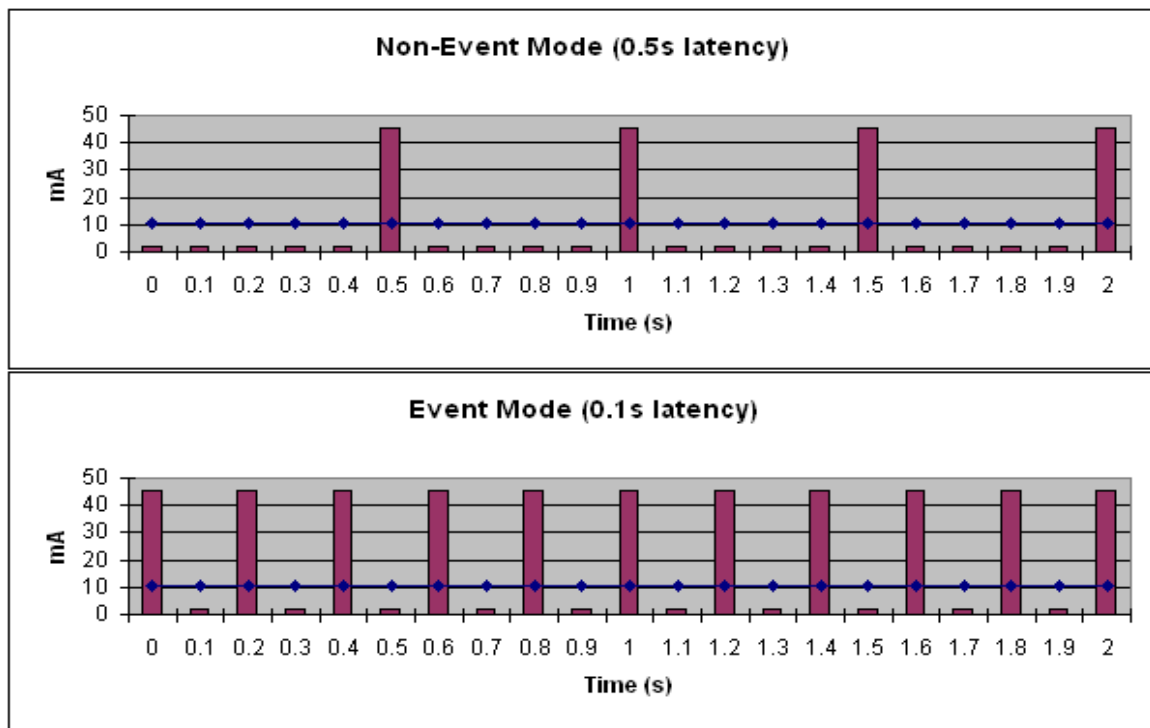
Figure 4.10. Power harvesting (lines) versus power consumption (bars)
