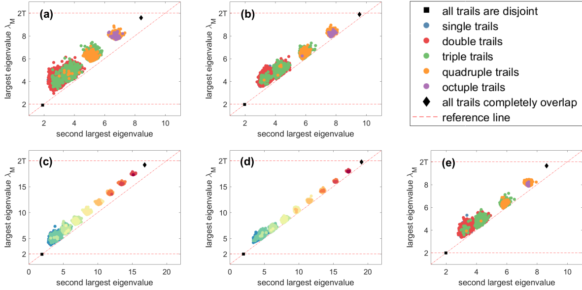
Figure 1.4: Plots of the largest and second largest eigenvalues for different Forest sizes and trails lengths.
