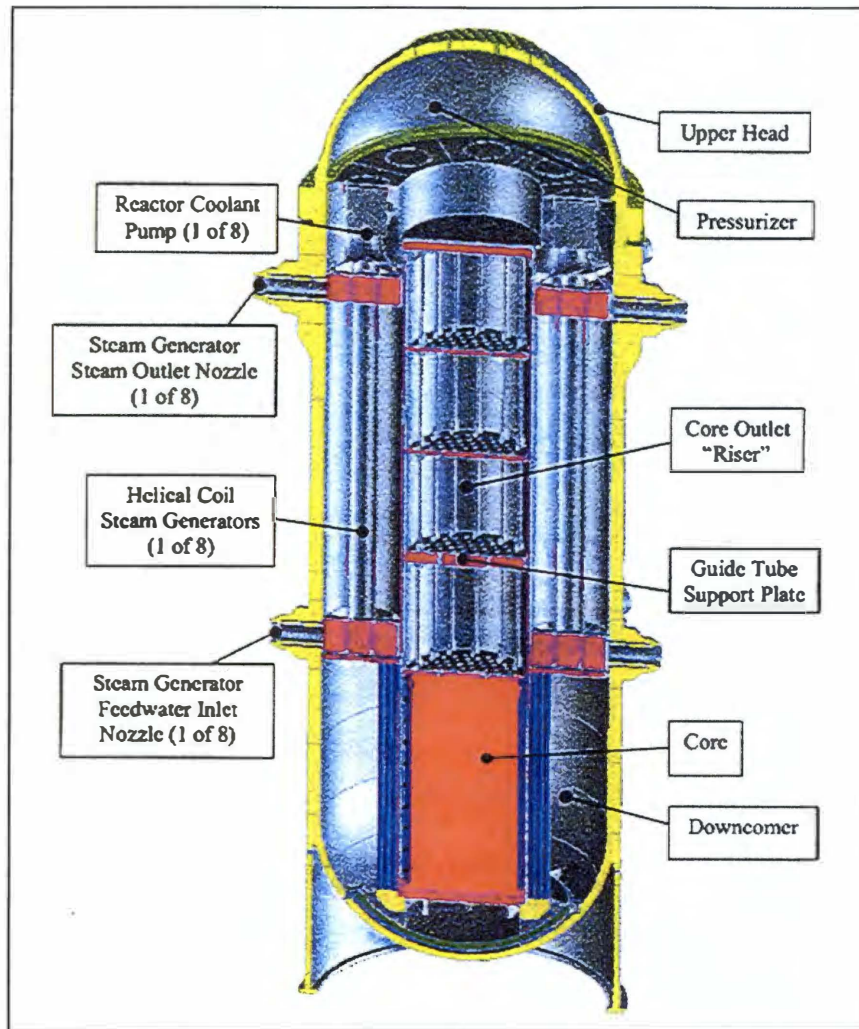
Figure 2-1. IRIS Reactor Vessel Internals [Source: Westinghouse, 2002]
