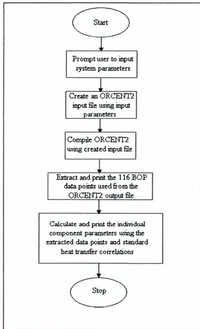
Figure 3-1. Flowchart for BOSCO
