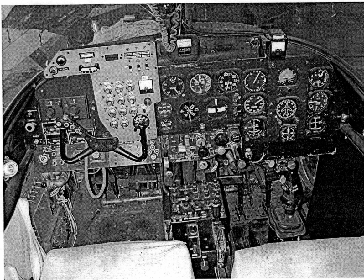
Figure 3-3 Navion Cockpit
