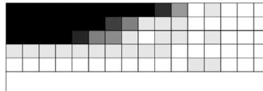
30% material fraction - fixed root cantilever
