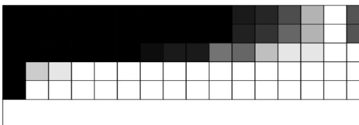
50% material fraction - fixed root cantilever
