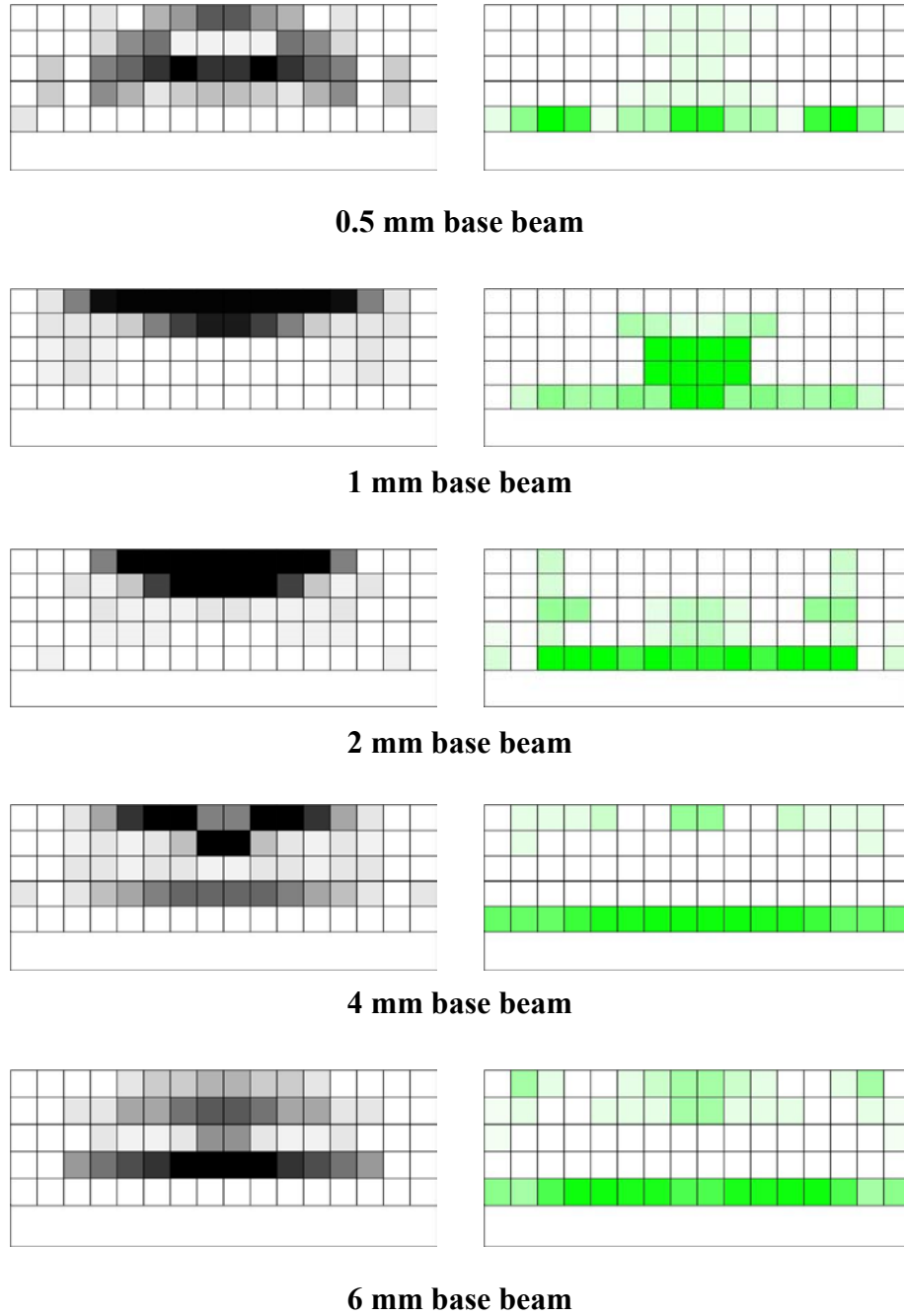
Figure 4.9 – Optimization Results - Base Beam Thickness Parameter Study
