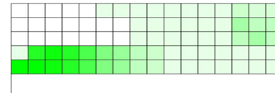
40% material fraction - fixed root cantilever
