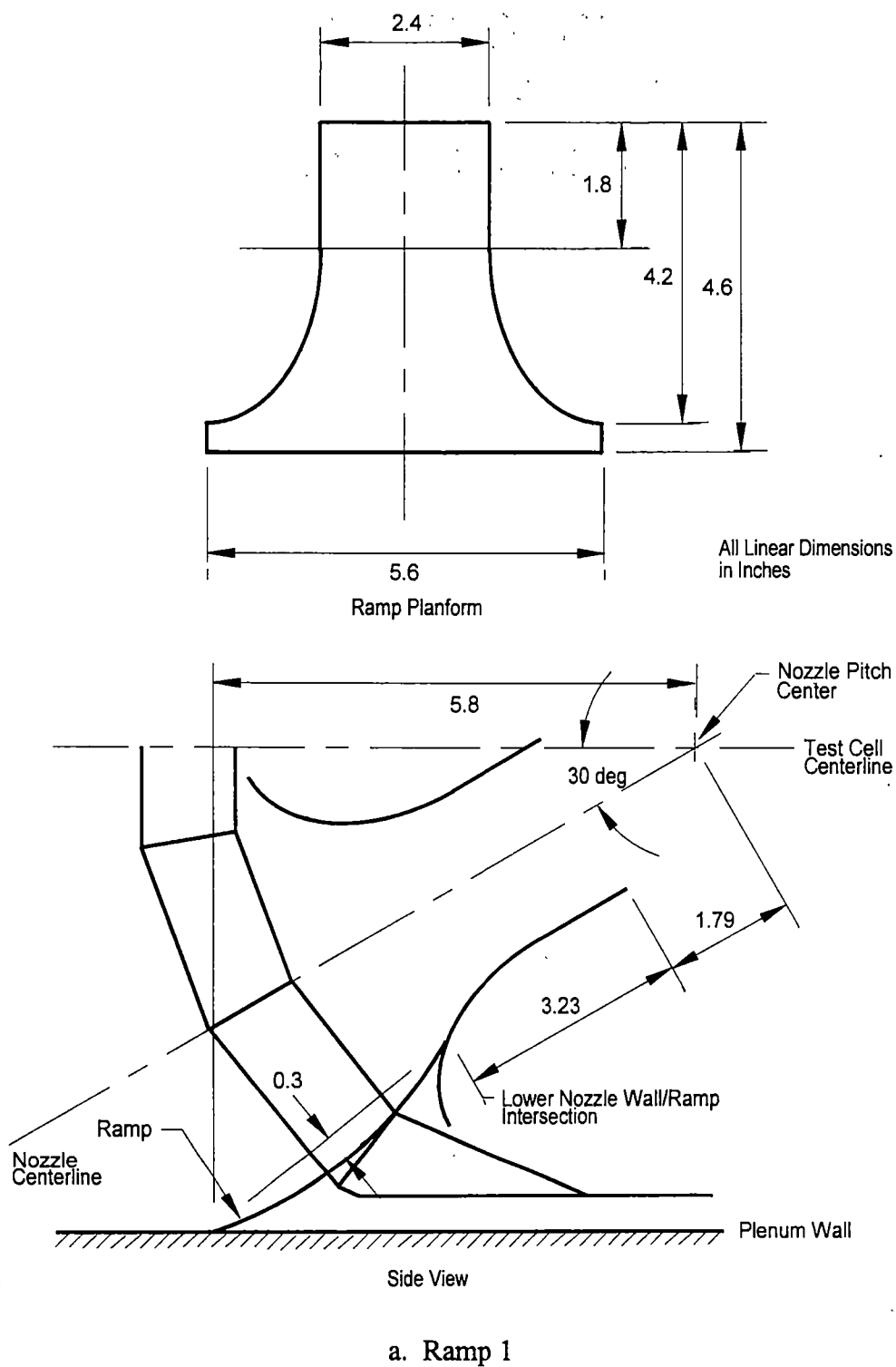
Figure 21. Variable-Area Nozzle Water Flow Model Ramp Configurations.
