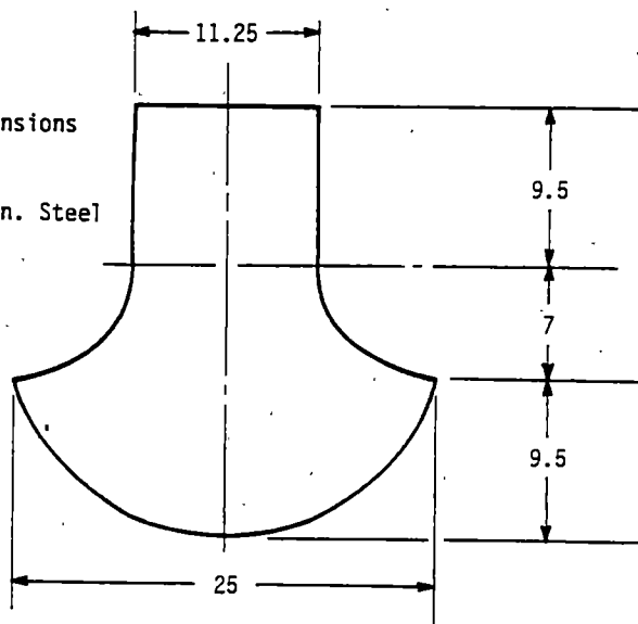
Ramp Planform
