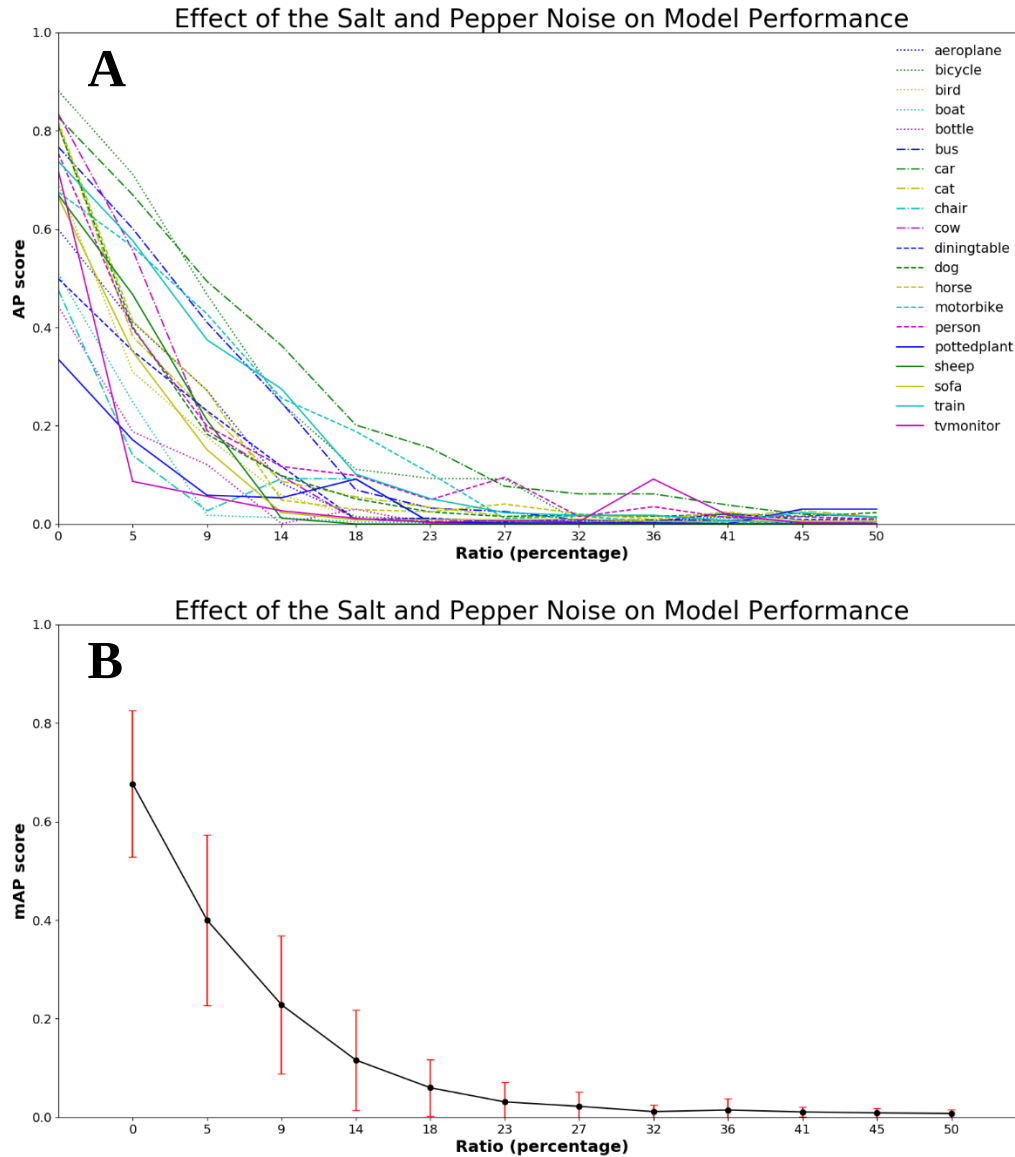
Figure 4.10 Effect of salt and pepper noise on model performance: (A) AP by VOC class and (B) mAP overall. Model performance was measured for images applied with salt and pepper noise ranging from 0% (untransformed) to 50% (extremely noisy). As the salt and pepper noise increases from 0% to 14%, performance decreases sharply due to low levels of noise distorting the object features quickly. Above 14%, model performance keeps decreasing steadily as features are almost unrecognizable by the model even though objects are distinguishable by a human viewer.
