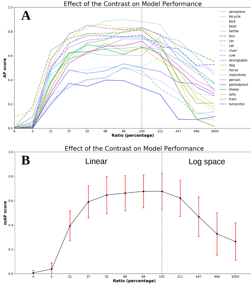
Figure 4.4 Effect of image contrast on model performance: (A) AP by VOC class and (B) mAP overall. Model performance was measured for images ranging in contrast from 0% (all gray) to 2000% (heavily contrasted), including 100% (untransformed, vertical dashed line). At 0% contrast, the class “cat” stands out as unusual having an AP score of 0.09, which is within the range of random guessing with 20 classes. As the contrast increases from 0% to 5%, performance only slightly increases since the model is not able to distinguish features from the low contrasted images. From 5% to 21%, performance sharply increases as the model is able to differentiate objects from one another. Above 21%, model performance behaves analogous to brightness (fig. 10), due to both being related to image intensity.
