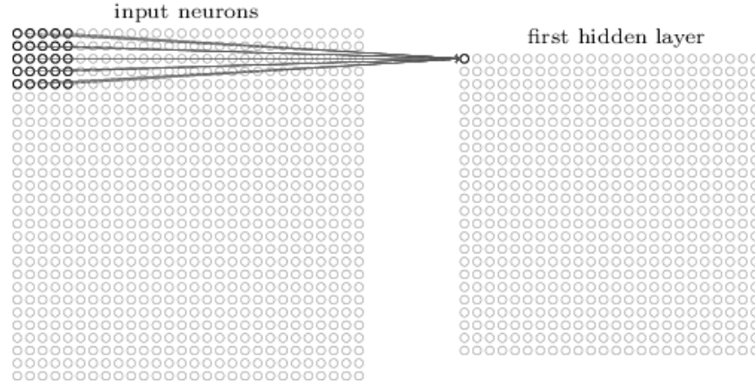
Figure 2.3 Example of a 5x5 convolutional kernel being applied to a 28x28x1 image, from [54]. The convolutional kernel is used in the sliding window technique (more precisely, convolving). It moves one pixel to the right each iteration, and once it reaches the end, it starts again on the left side and moves one pixel down. This results in going from 28x28 in the input to 24x24 in the first hidden layer.
