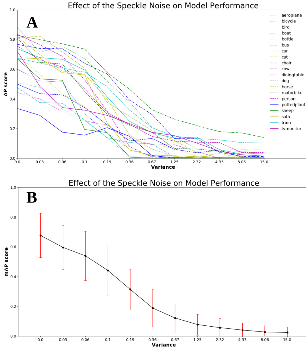
Figure 4.9 Effect of speckle noise on model performance: (A) AP by VOC class and (B) mAP overall. Model performance was measured for images applied with speckle noise with variance ranging from 0 (untransformed) to 15 (extremely noisy). As the speckle noise variance increases from 0 to 0.36, performance decreases gradually due to low levels of noise distorting the object features quickly. After 0.36 variance, model performance keeps decreasing steadily as features are almost unrecognizable by the model even though objects are distinguishable by a human viewer.
