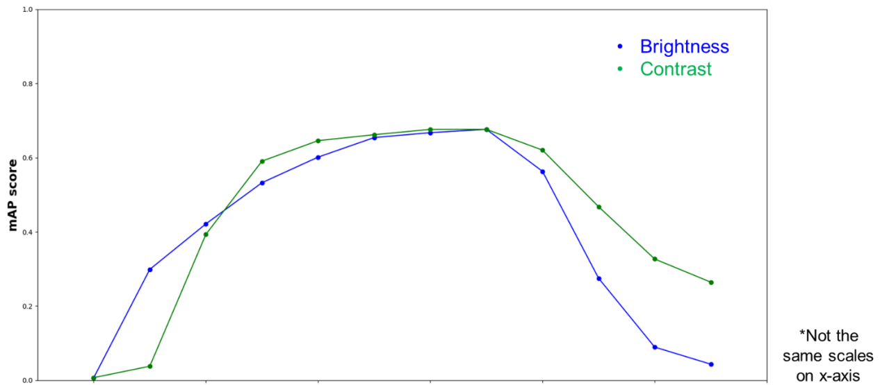
Figure 4.11 High impact degradation methods’ results displayed in one graph. Both the brightness and contrast results placed into one graph to allow a clearer depiction of why they are categorized as high impact. Both methods sharply decrease at the low and high ends of the range with a plateau in the middle.
