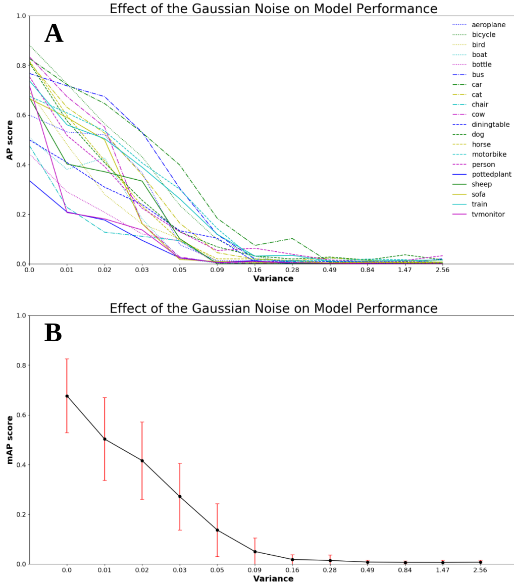
Figure 4.8 Effect of Gaussian noise on model performance: (A) AP by VOC class and (B) mAP overall. Model performance was measured for images applied with Gaussian noise with variance ranging from 0 (untransformed) to 2.56 (very noisy). As the Gaussian noise variance increases from 0 to 0.09, performance decreases sharply due to low levels of noise distorting the object features quickly. After 0.09 variance, model performance keeps decreasing steadily as features are almost unrecognizable by the model even though objects are distinguishable by a human viewer.
