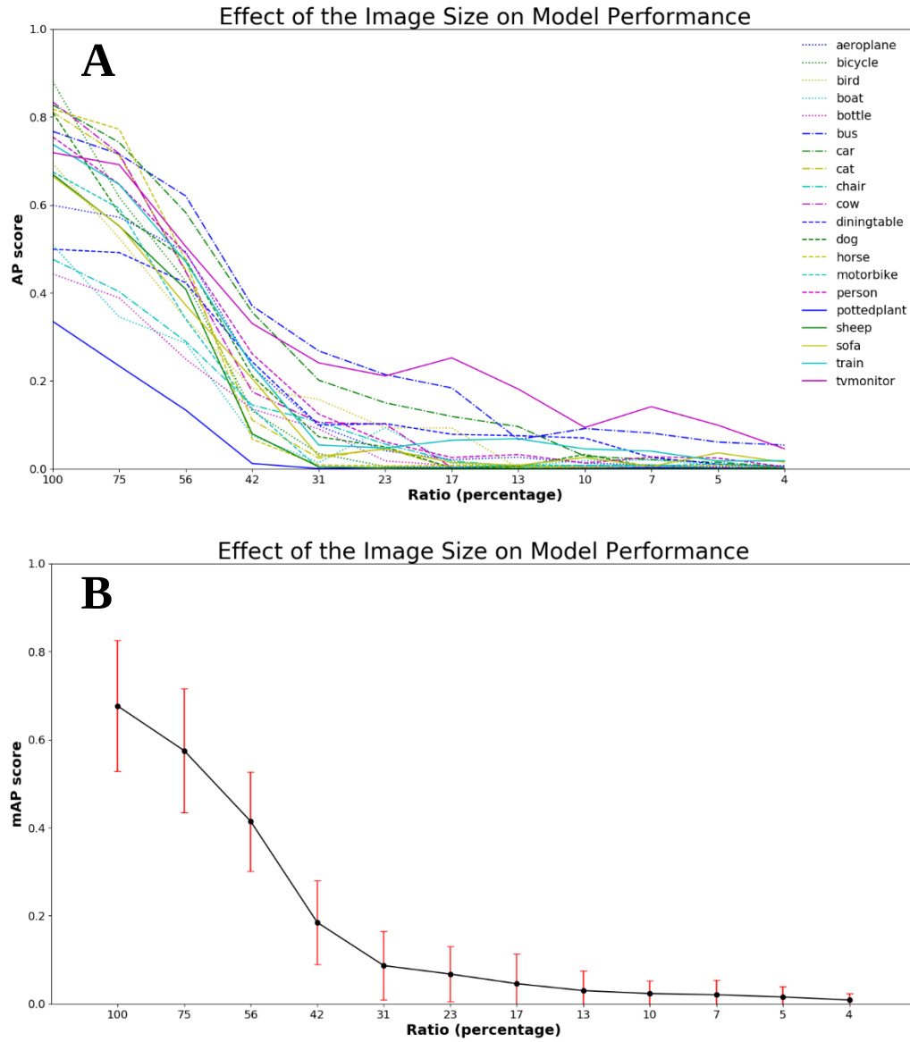
Figure 4.6 Effect of image size on model performance: (A) AP by VOC class and (B) mAP overall. Model performance was measured for images ranging in size from 100% (untransformed) to 4% (extremely pixelated), which were resized back to the original size to replicate pixelated images. As the image size decreases from 100% to 42%, performance decreases markedly due to the model not being able to distinguish features even though objects are still easily detectable by a human viewer. Below 42%, model performance decreases steadily as the images become more pixelated.
