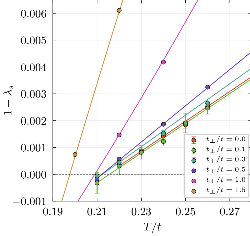
Figure 5.4: Temperature dependence of 1 - \lambda_s(T) for the composite bilayer system on a N_c = 36 site cluster for several different values of the interlayer hopping t_\perp . Error bars (s.d.) are shown for the smallest three values of t_\perp/t = 0.0, 0.1, 0.3 obtained by repeating the last DCA iteration using different random number seeds in the CTQMC cluster solver. The resulting T_c estimates for t_\perp/t = 0.0, 0.1 , and 0.3 fall within each other's range of uncertainty. Figure taken from our Ref. [4].
