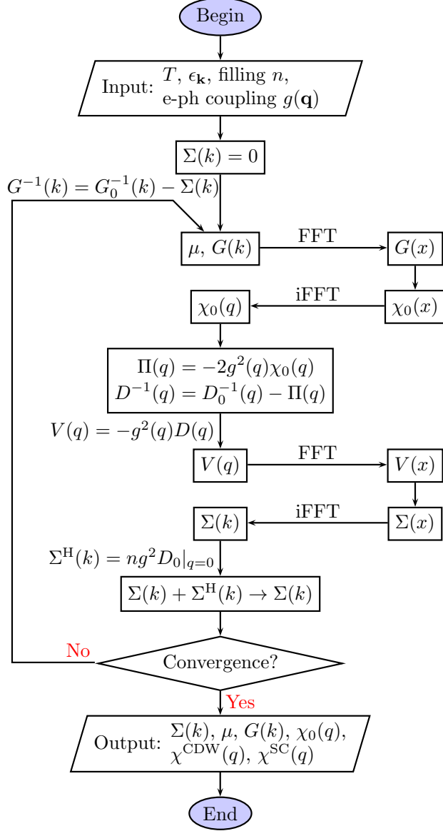
Figure 2.2: Algorithm for self-consistent iterations of Green's functions and self-energies with FFT. The Hartree self-energy \Sigma^H = n|g(\mathbf{q} = \mathbf{0})|^2 D_0(q = 0) = -2n|g(\mathbf{0})|^2/\Omega is a constant during iterations, and thus in practice the computation of \Sigma^H and the shift of electron self-energy \Sigma(k) \rightarrow \Sigma(k) + \Sigma^H can be moved outside the iteration loop and done after the convergence. Figure taken from our Ref. [1].
