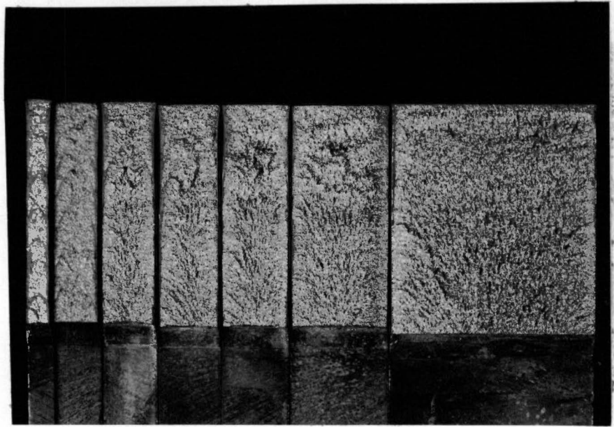
Figure 21. Fracture Surface Appearance as a Function of Specimen Thickness.
