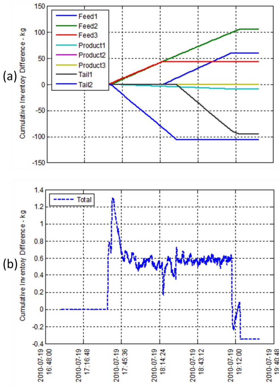
Figure 4-21. Cumulative inventory difference from July 19, 2010, after installation of the PI controller. Plot (a) is the CID for each station, and plot (b) is the total CID calculated by summing the data in plot (a).
