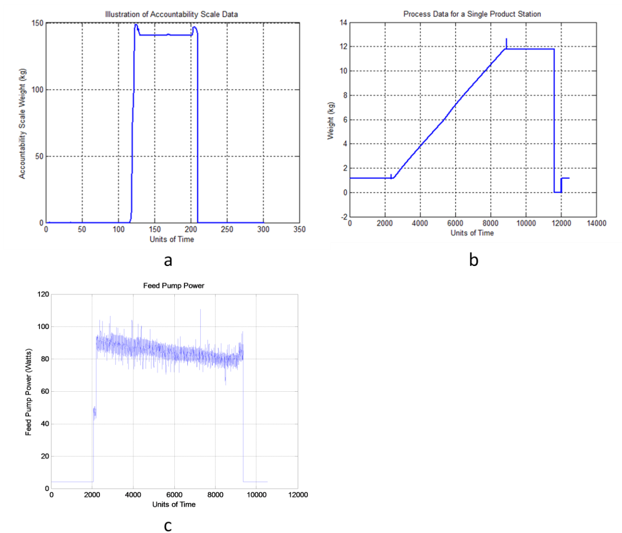
Figure 3-7. A sample of the different data types collected at the ORNL mock feed and withdrawal facility. The accountability scale data (a) is a step function of a tank's weight before and after processing. The process scale data (b) is continuous and shows the instantaneous weight of a tank on a station as material is being processed. The feed pump power (c) data is a type of facility control data and may either be a step function or continuous depending upon the instrumentation.
