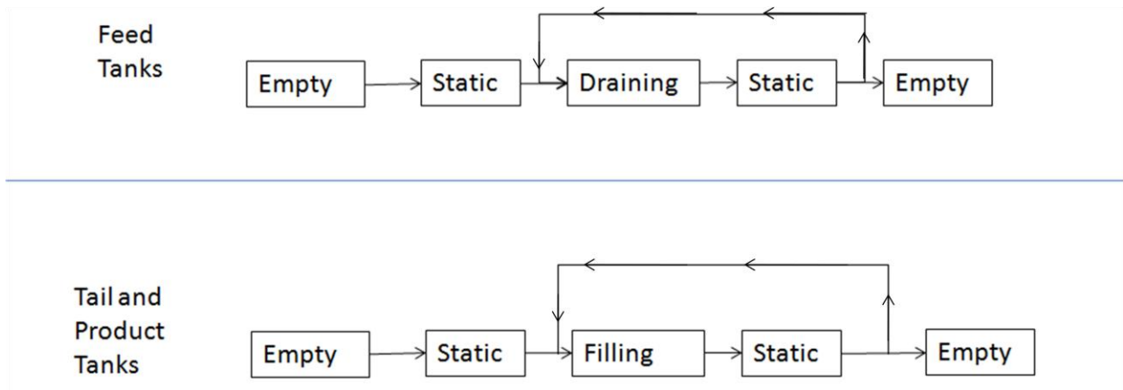
Figure 4-16. The life cycle of a process station with respect to 4 possible states.
