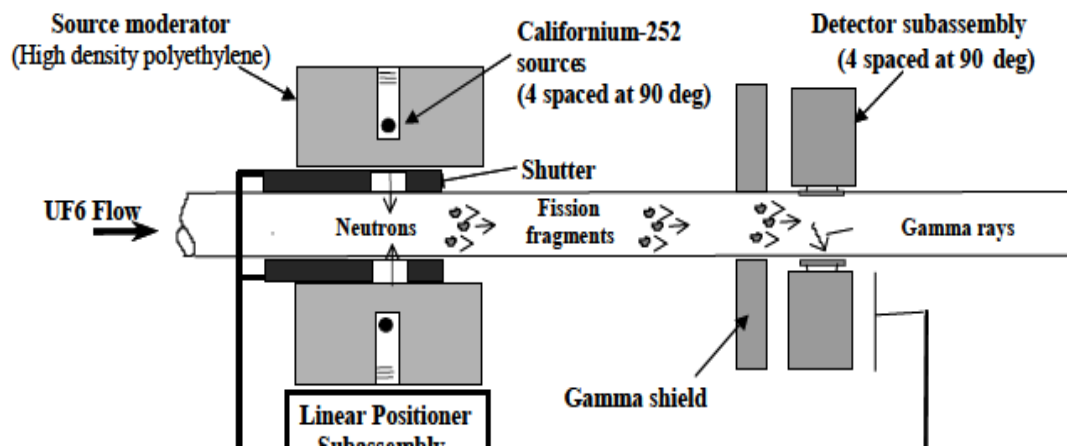
Figure 3-1. A schematic of the Fissile Mass Flow Meter (FMFM) used in the blend-down monitoring system. When the shutter is opened a Californium-252 neutron source induces fissions in a uranium hexafluoride stream. Downstream of the neutron source is a shielded detector array used to detect delayed gammas from Uranium-235 fission. The number of delayed gammas detected is proportional to the amount of Uranium-235 in the stream. The time delay between the source shutter opening and the initial detection of fission gammas can be used to calculate the flow velocity.
