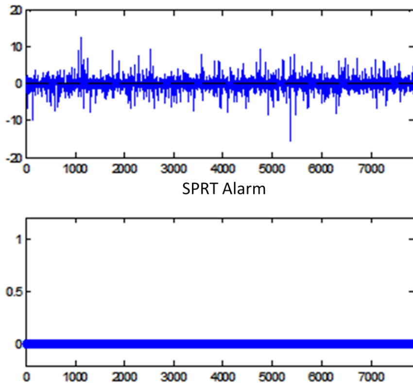
P-LEU Velocity Sensor Residuals for 10% Bleed-off Case (Model 2)
