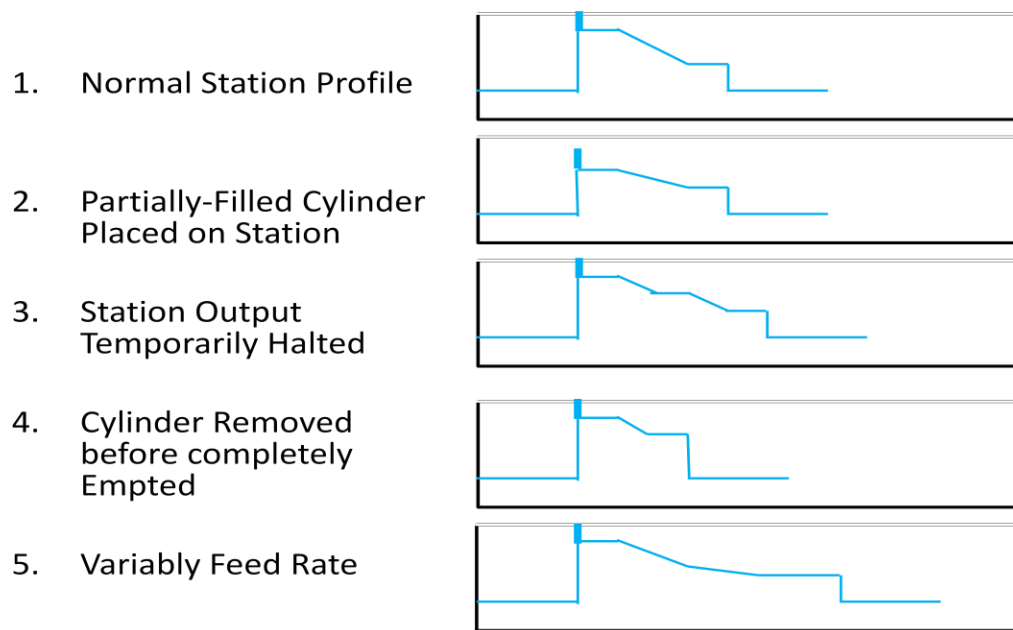
Figure 2-8. Changes in a GCEP feed station profile under different operating conditions. The spikes when a tank is added or removed from the scale represent expected fluctuations.
