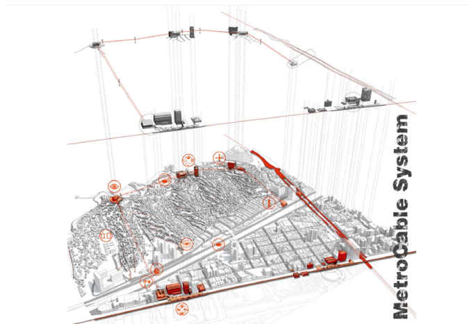
Figure 3.02 Exploded Axon of the Metro Cable System ( Urban Think Tank )
