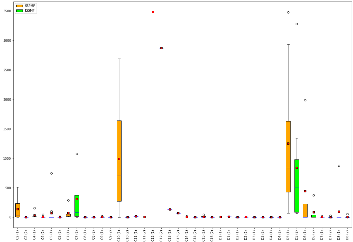
Figure 3.4: Comparison of the solution times for the instances in cluster C and D, that are solved with both methods.
