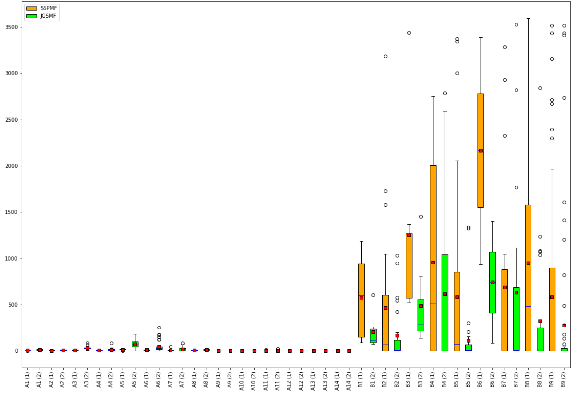
Figure 3.3: Comparison of the solution times for the instances in cluster A and B, that are solved with both methods.
