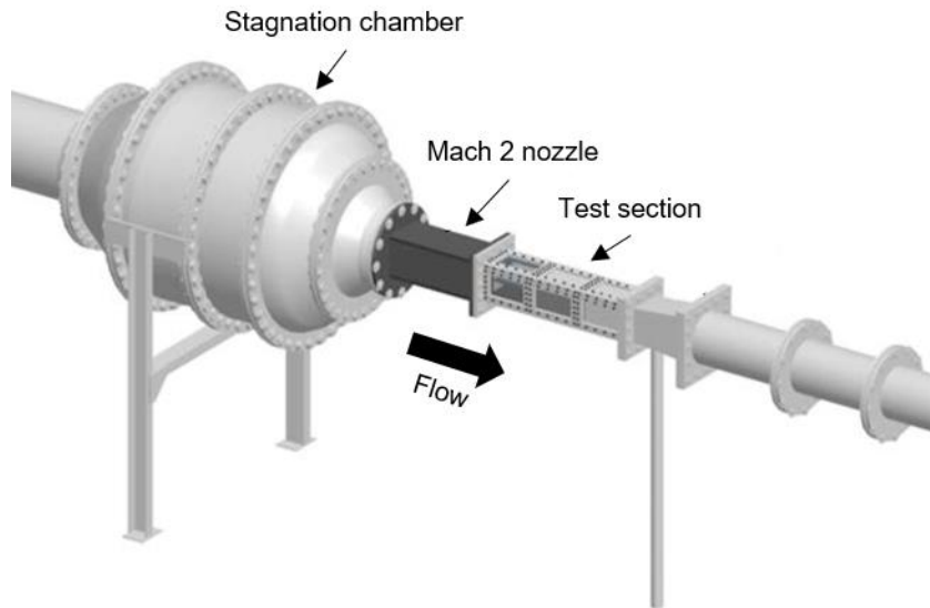
Figure 2.1. Schematic of the UTSI Mach 2 blowdown wind tunnel. Figure adapted from Kocher et al. [71].
