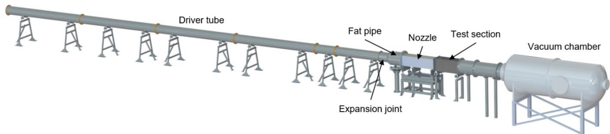
Figure A.1. Schematic of the Mach 4 Ludwig Tube at the UTSI TALon facility.
