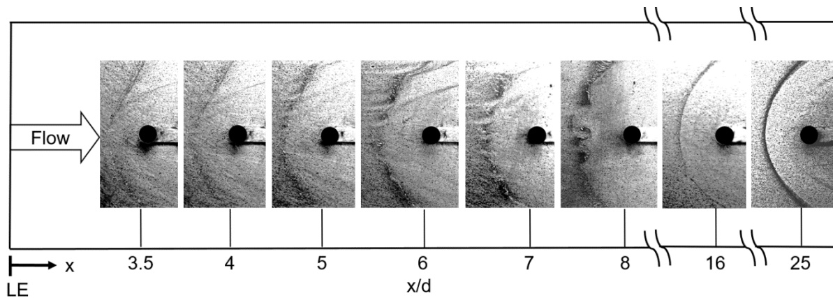
Figure 2.7. Surface oil flow visualization of the boundary layer separation as the cylinder moves downstream of the plate leading edge. Flow is from left to right.
