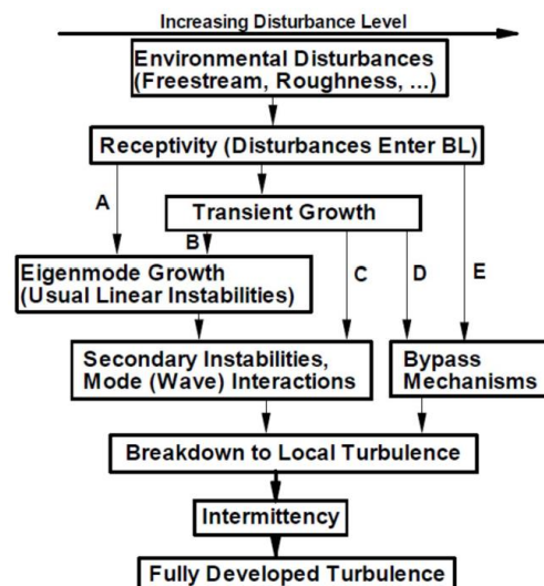
Figure 1.8. Waterfall plot describing the mechanisms that lead to boundary layer transition. Image adapted from [54], courtesy of J.D. Schmisseeur.
