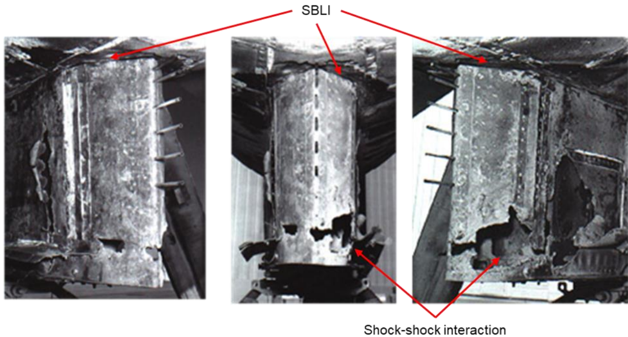
Figure 1.2. Images of the damage to the ventral fin on the underside of the X-15A-2 vehicle [18].
