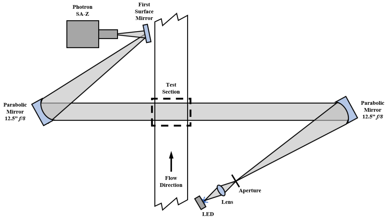
Figure A.3. Schematic of the schlieren setup for the Mach 4 Ludwig tube at the UTSI TALon Facility.
