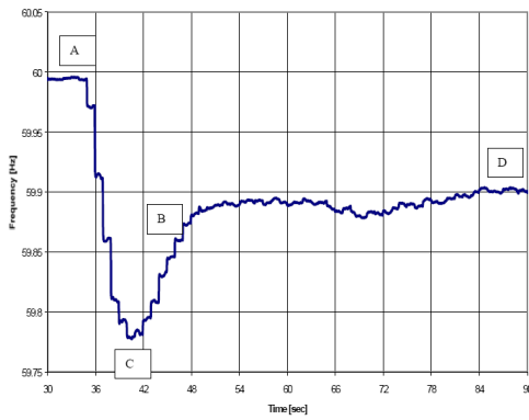
(c) NERC defined A, C, and B points
