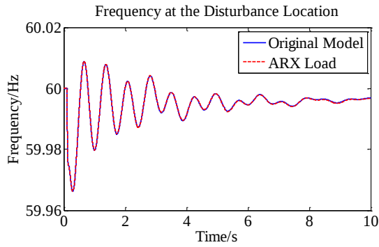
(a) Frequency at the Disturbance Location
