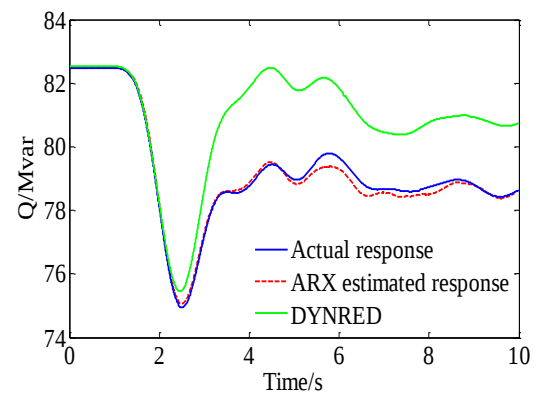
(b) Reactive power of tie line
