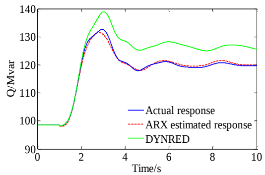
(b) Reactive power of tie line
