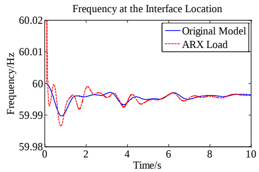
(b) Frequency at the Interface Location
