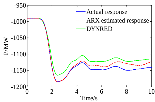
(a) Active power of tie line
