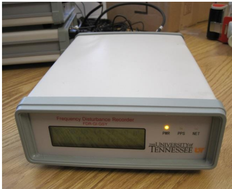
Figure 1-4 Second-generation FDR
