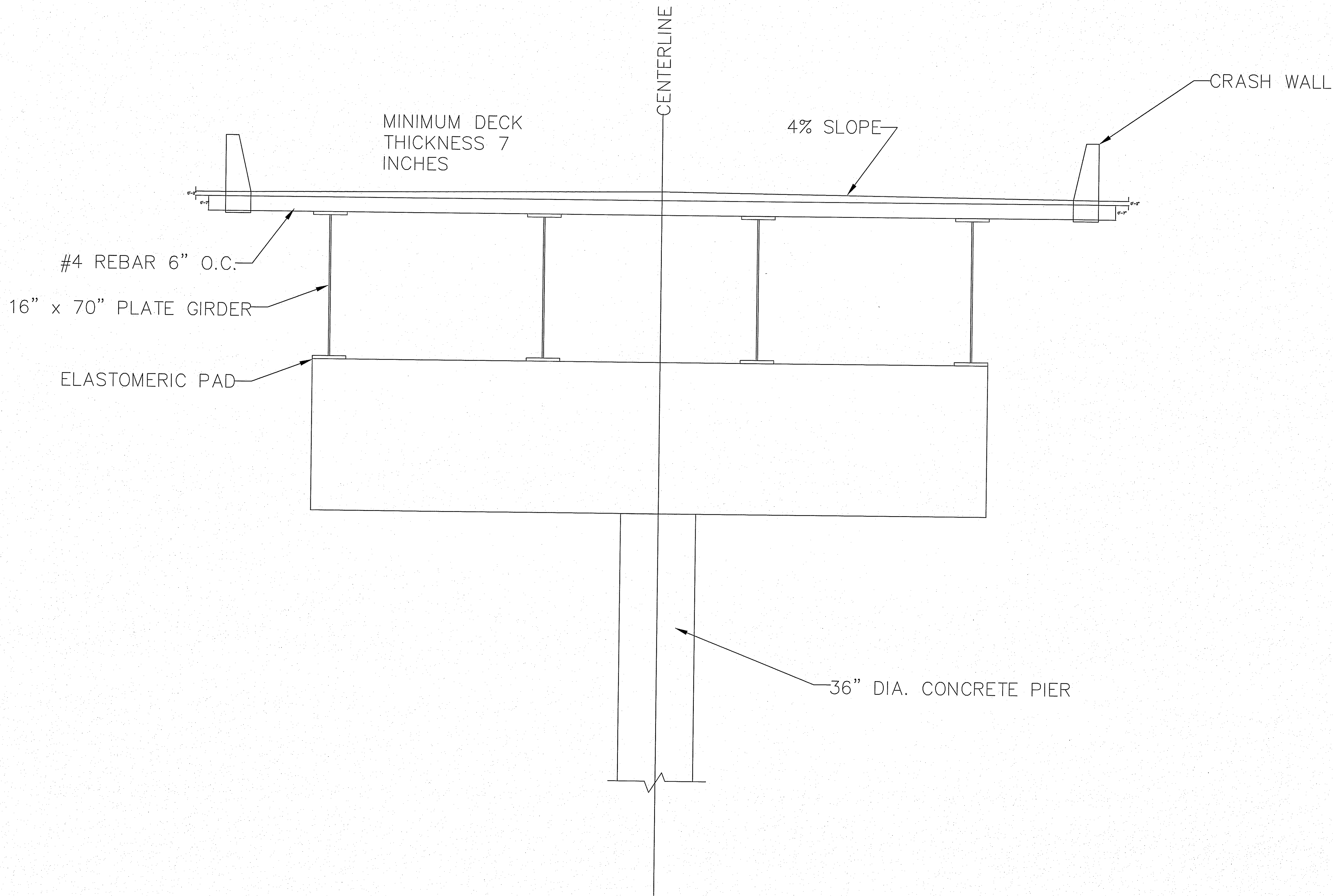
2 10F2 BRIDGE DECK CROSS SECTION SCALE: 1/2"=1'
