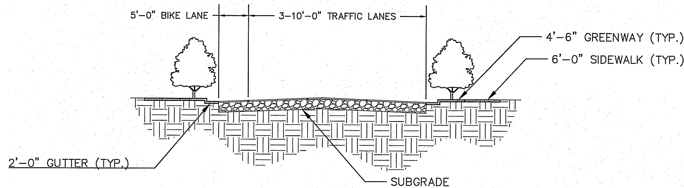
2 1 OF 6 TYPICAL ROAD PROFILE SCALE: 1" = 10'
