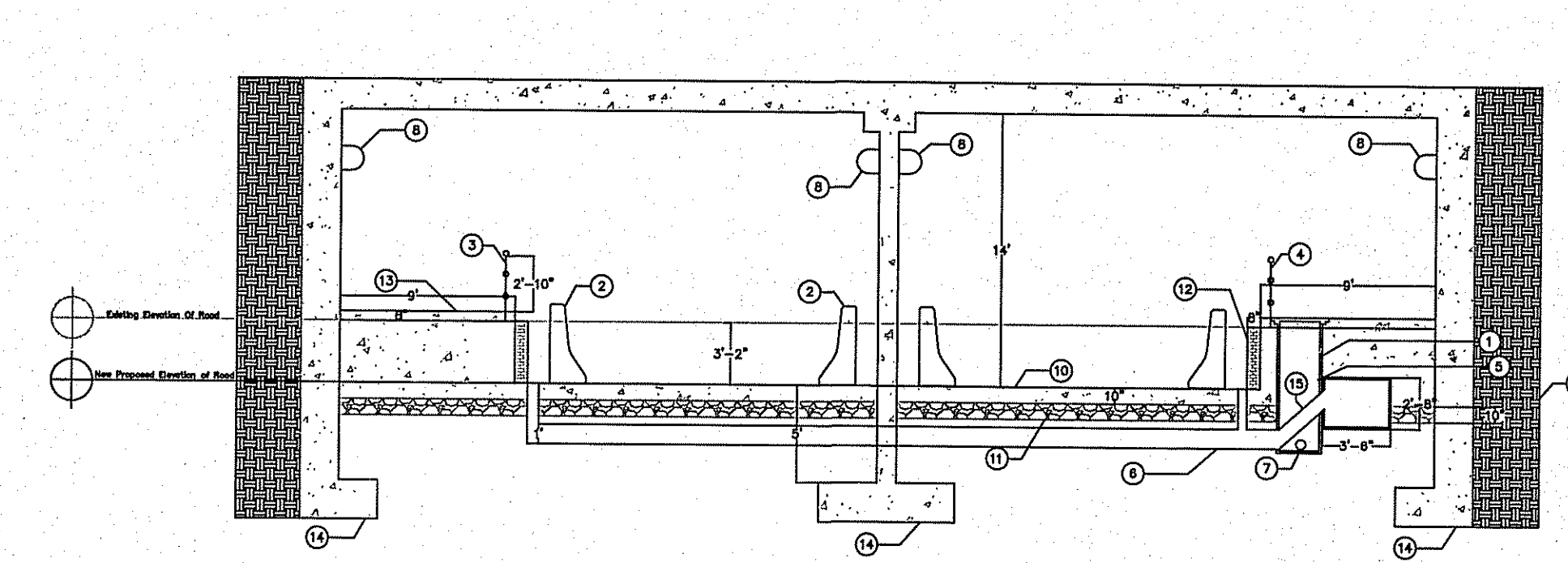
C-S 20F2 Proposed Underpass Cross-Section SCALE: 1/8" = 1'0"
