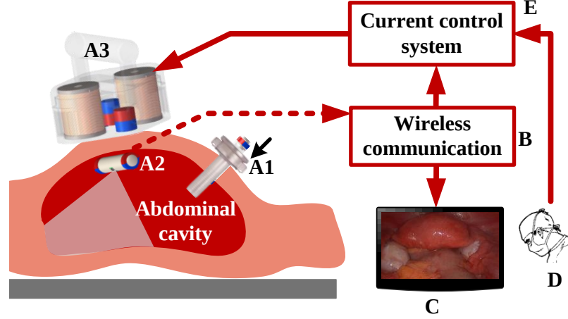
Figure 4.1: Conceptual illustration of the magnetic actuated camera robot. (A1) The process of inserting the camera robot into the patient’s abdominal cavity through a trocar. (A2) The initialized position after the camera inserted inside. (A3) The stator. (B) The visual information is transmitted through wireless communication from the camera to the display terminal (C) and current control system (E). (D) A surgeon can control the current input of the stator through current control system (E) for a desired robot pose.
