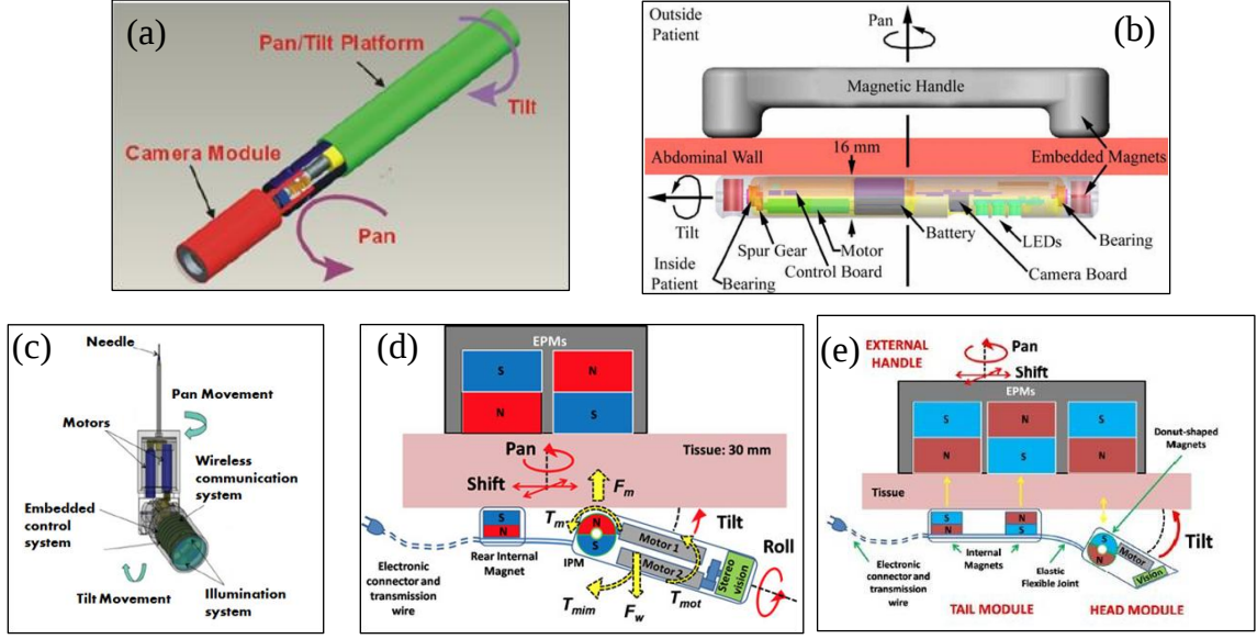
Figure 1.2: Laparoscopic cameras robots. (a) Hu et al. (2009); (b) Platt et al. (2009); (c) Castro et al. (2013); (d) Simi et al. (2013); (e) Simi et al. (2011).
