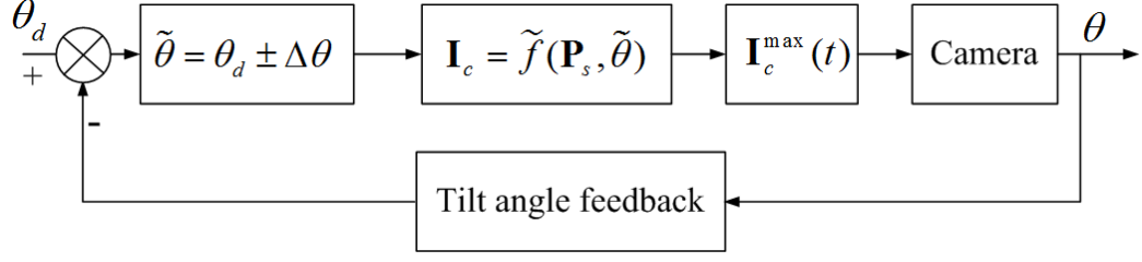
Figure 5.6: Block diagram of the camera tilt motion control.
