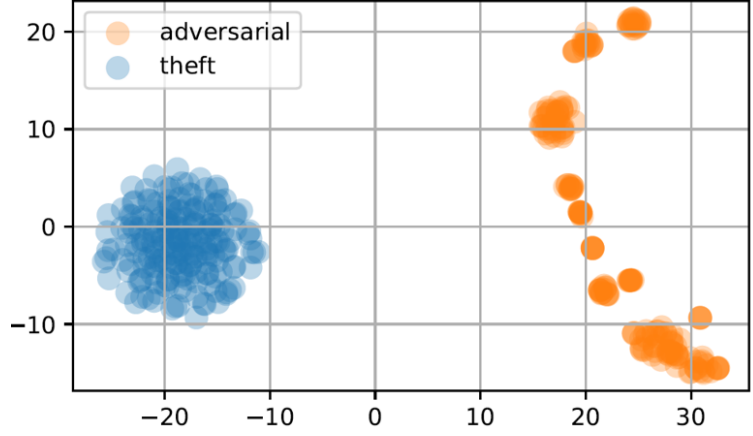
Figure 5.5: Energy theft/adversarial measurements visualization (t-SNE dimensionality reduction)
