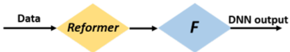
Figure 5.3: Input Reconstruction
