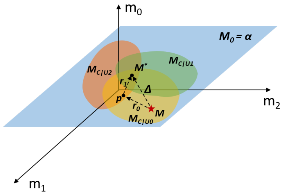
Figure 4.4: Iteration illustration.
