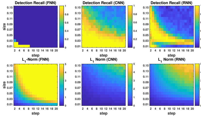
Figure 3.6: Black-box SearchFromFree.
