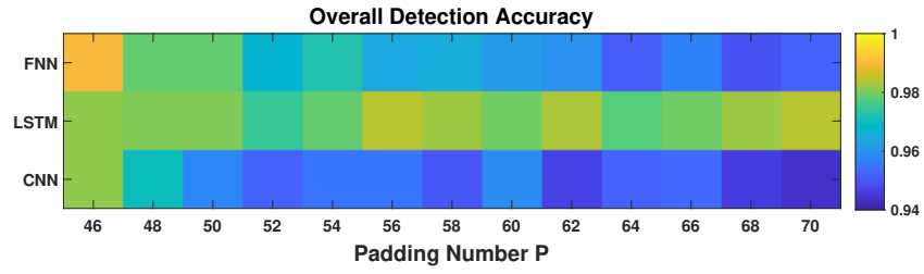
Figure 5.10: Detection accuracy of random inputs padding framework.
