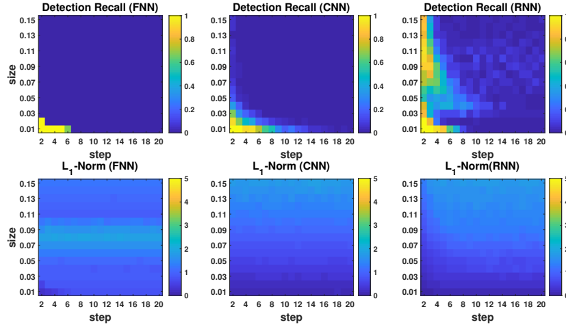
Figure 3.5: White-box SearchFromFree
