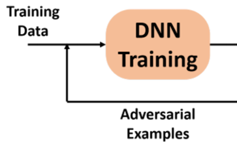
Figure 5.1: Adversarial Training
