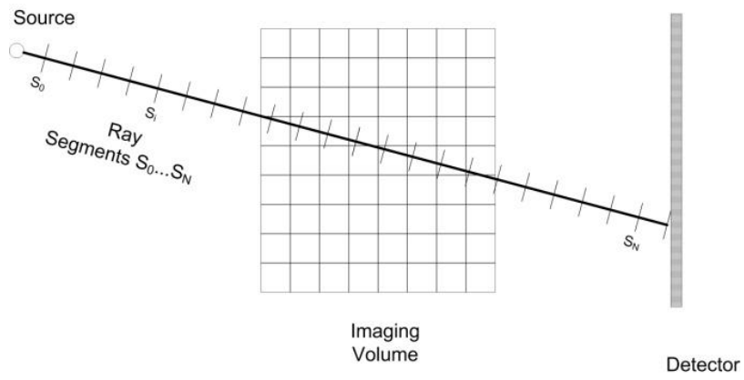
Figure 18. Division of ray into independent segments for the OVIA Method.
