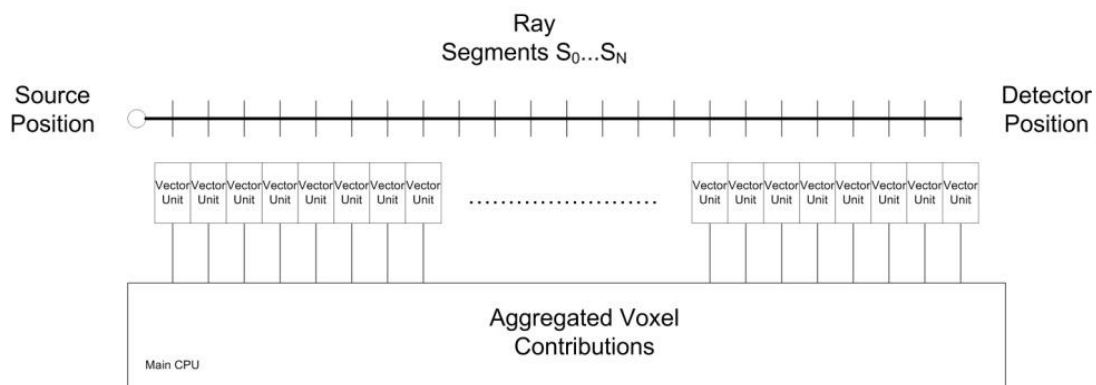
Figure 19. Vectorized OVIA Hardware Organization for many-core GPGPU.
