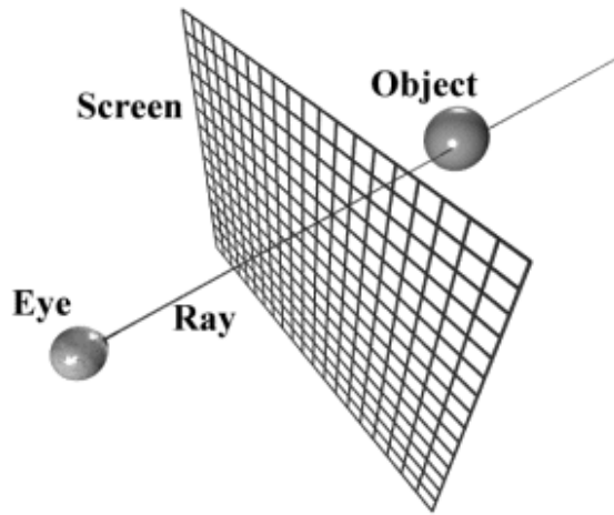
Figure 12. Ray tracing 2D solution [Buck, 1999].
