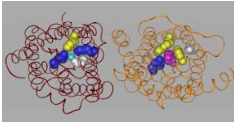
Figure 39. Ribbon diagram of AQP1 and GlpF showing bound substrates and key pore residues. Structures for AQP1 (left) and GlpF (right) were generated based on the published coordinates from the solved crystal structures of these proteins (Fu et al., 2000; Sui et al., 2001). A) Structures are viewed in the plane of the membrane, the four water molecules bound in the pore of AQP1 are shown in cyan, while NPA asparagines (bound to water 2 and 3) are shown in white. Basic residues of the aromatic/arginine region (ar/R) are shown in blue, hydrophobic side chains are yellow and hydrophilic side chains are in white. GlpF structure is labeled the same with two of the bound glycerols in the pore shown in magenta. B) Structures from the cytoplasmic face looking down through the pore. The four residues forming the narrow ar/R selectivity filter are shown bound to water (AQP1) or glycerol (GlpF).
