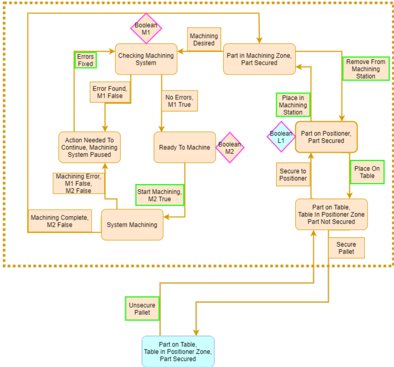
Figure 2.6: Machining and part positioner subsection of the state diagram
