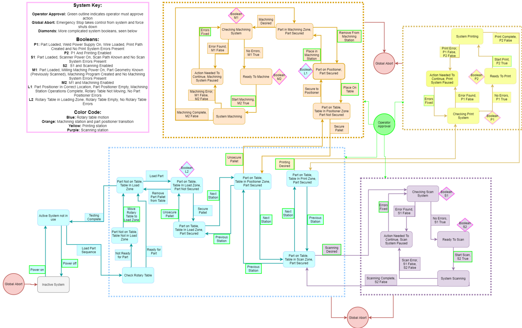
Figure 2.3: Hybrid manufacturing state diagram
