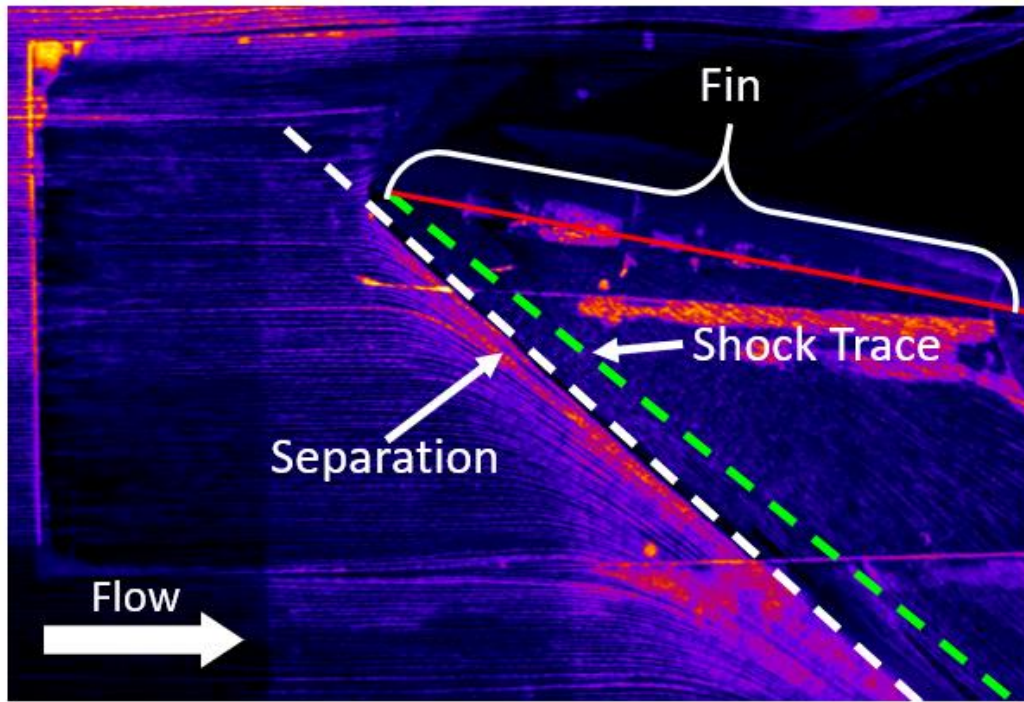
Figure 2.20. Oil flow of fin at 10^\circ angle of attack in the UTSI Mach 2 wind tunnel. Courtesy of Douthitt et al.
