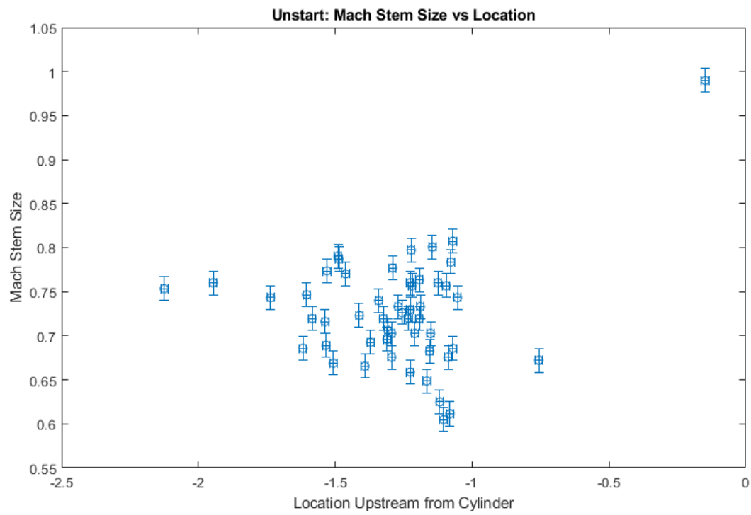
Figure 3.19. The Mach stem size versus location in the wind tunnel.
