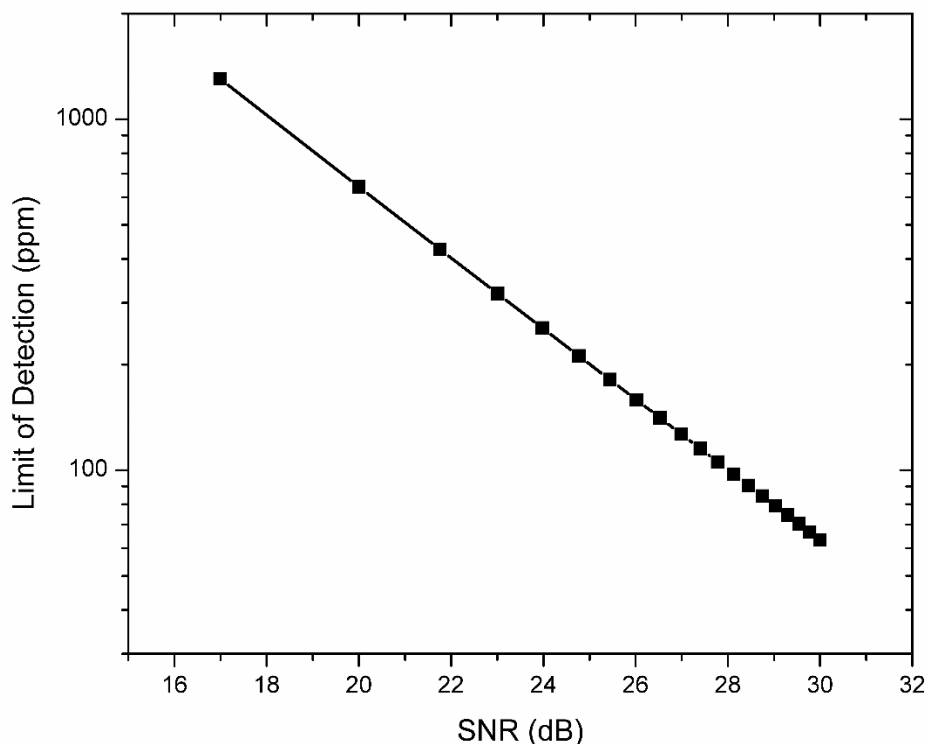
Figure 4.14. LoD respect to SNR
