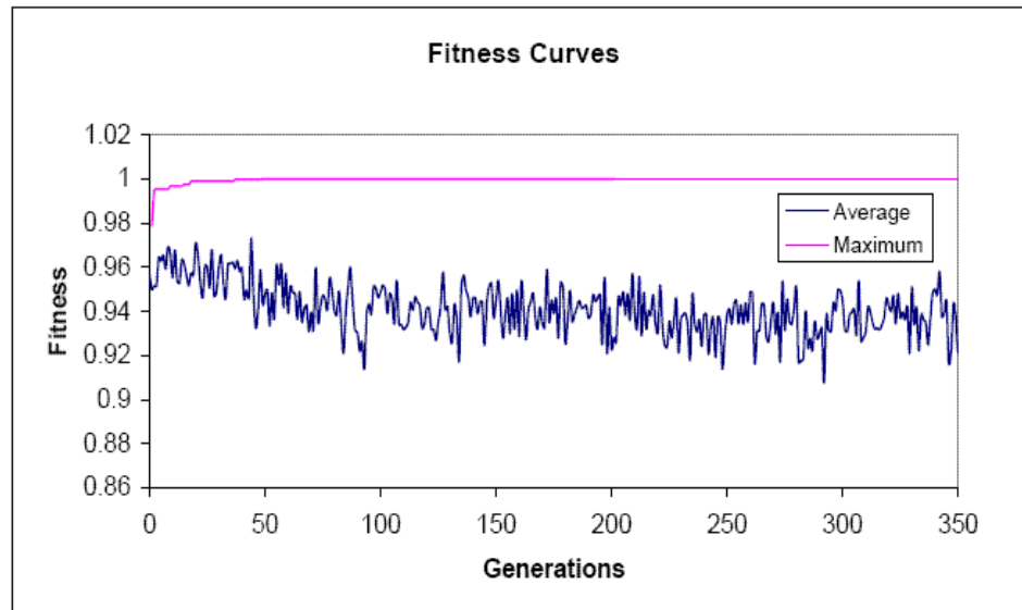
Figure 50 Average and maximum fitness trends for the first re-training cycle
