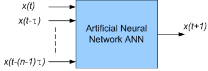
Figure 36 Time delayed neural network
