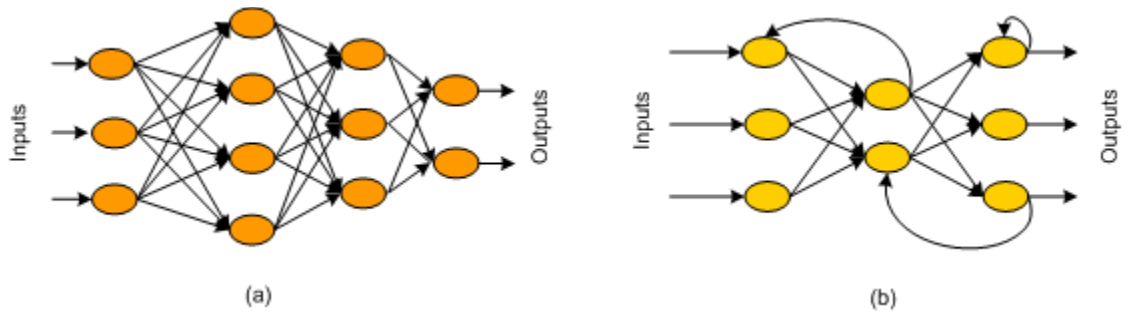
Figure 4 (a) Non-recurrent multilayer perceptron network (b) Recurrent artificial neural network
