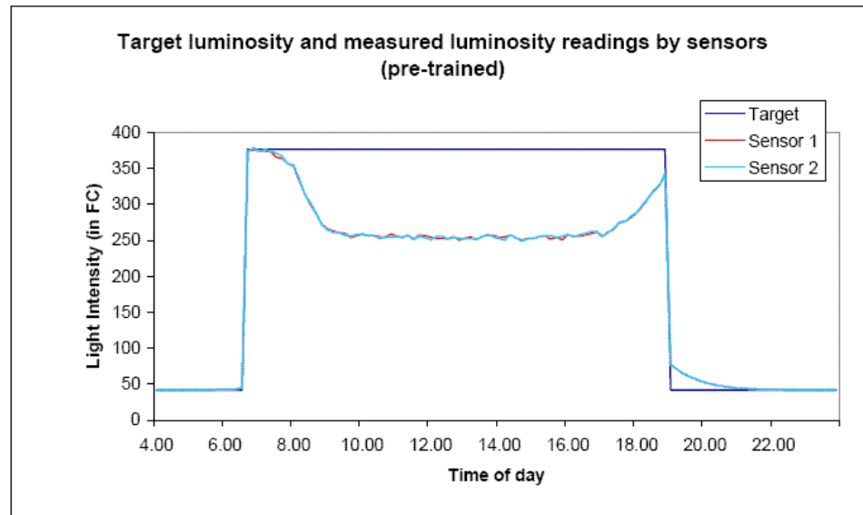
Figure 55 Target and measured luminosity levels as recorded by the light sensors. (pre-trained case)
