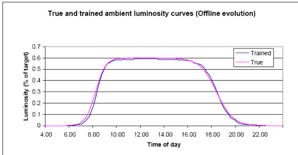
Figure 41 Results of the BbNN pre-training. Plot shows the actual and the predicted ambient luminosity values as learnt by BbNN
