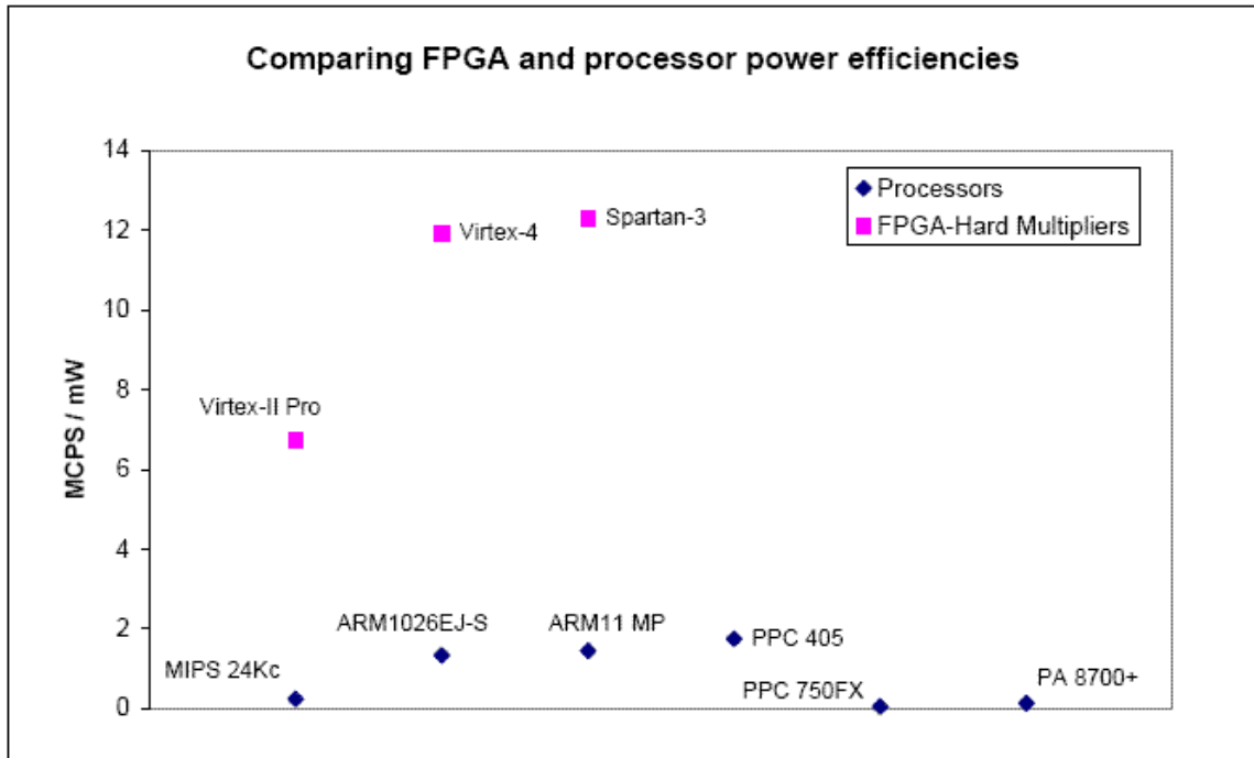
Figure 84 Comparing power efficiencies of processors and FPGAs (Hard Multiplier)
