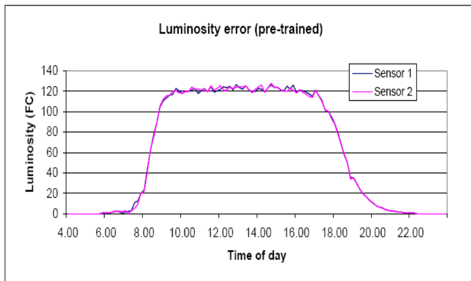
Figure 56 Error between target and measured luminosities (pre-trained case)
