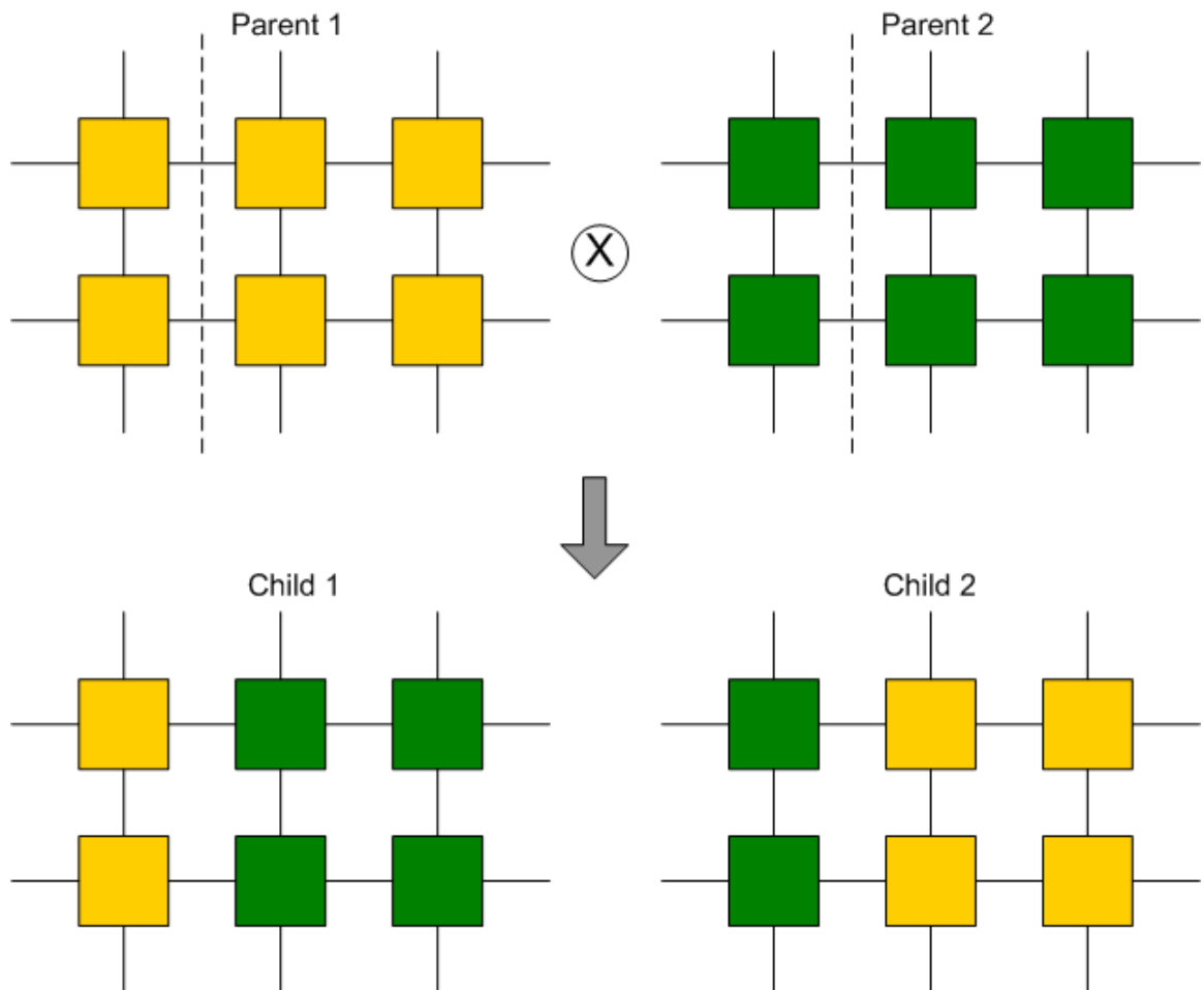
Figure 15 Structure crossover operation in BbNN
