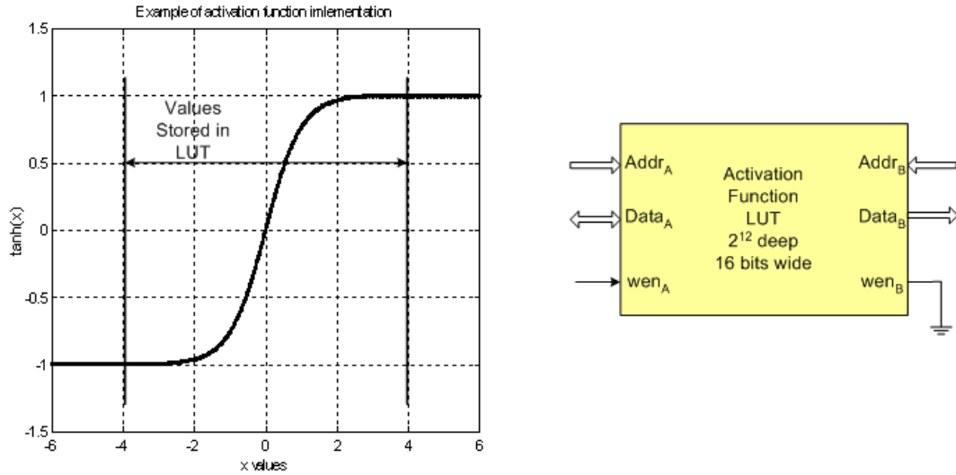
Figure 17 Activation function LUT illustration
