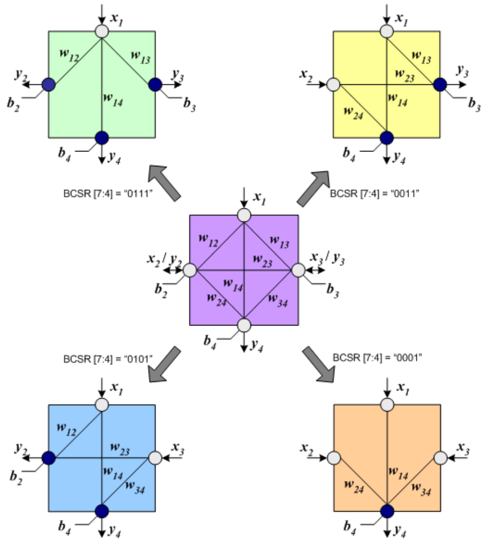
Figure 18 Smart Block-based Neuron to emulate all internal neuron block configurations
