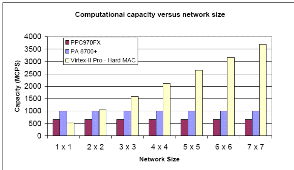
Figure 86 Computational capacities of FPGAs and processors as a function of network size
