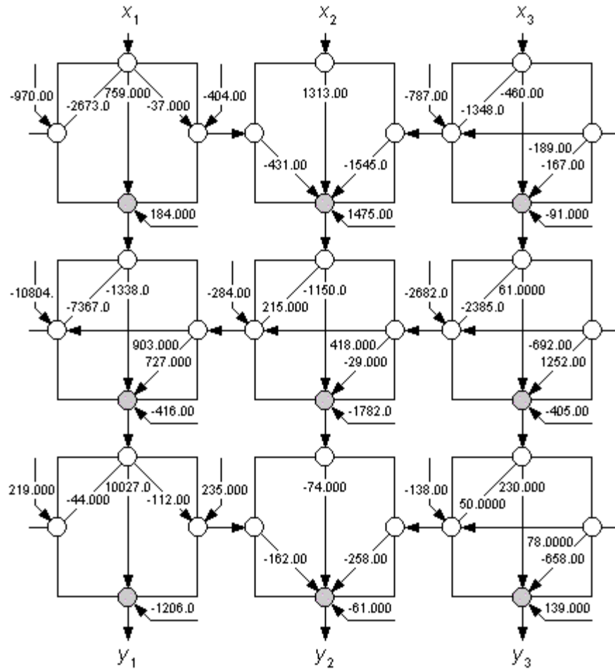
Figure 32 Evolved BbNN network for Iris plant classification database
