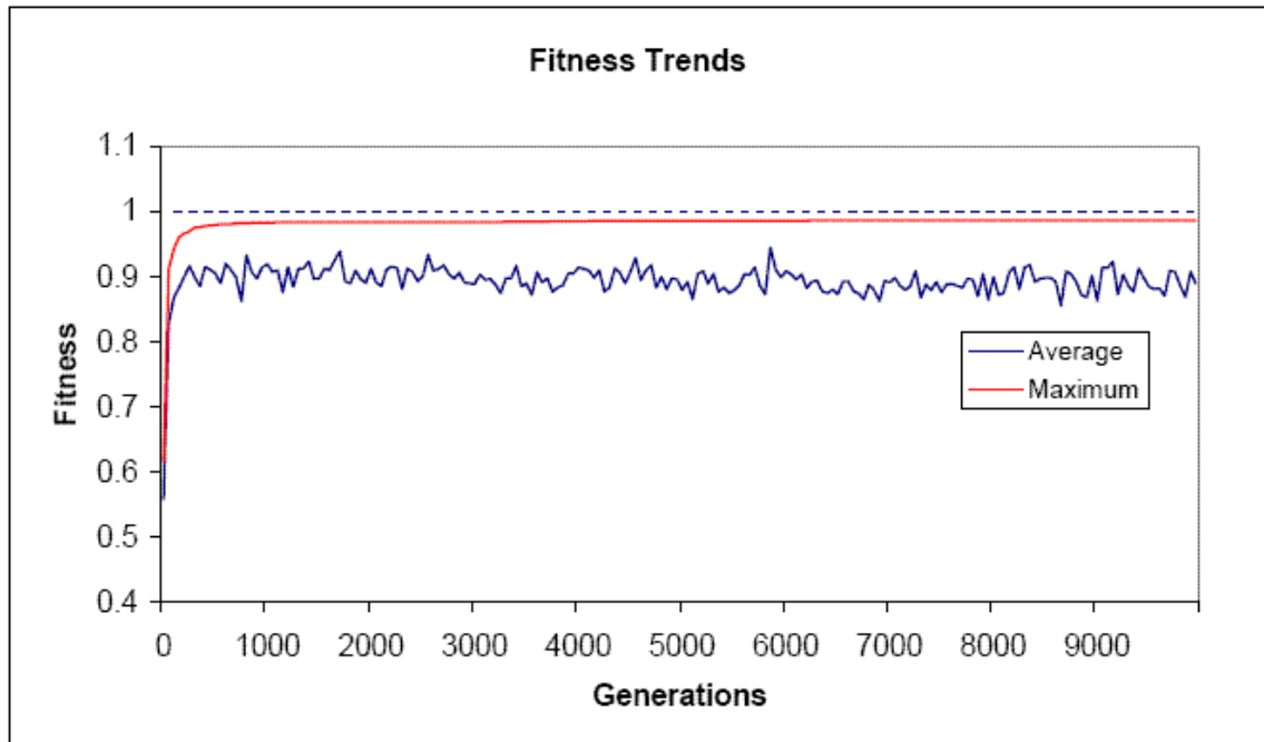
Figure 30 Fitness trends was Iris plant classification using BbNN
