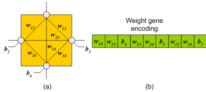
Figure 13 BbNN weight gene encoding (a) Neuron block (b) Weight encoding
