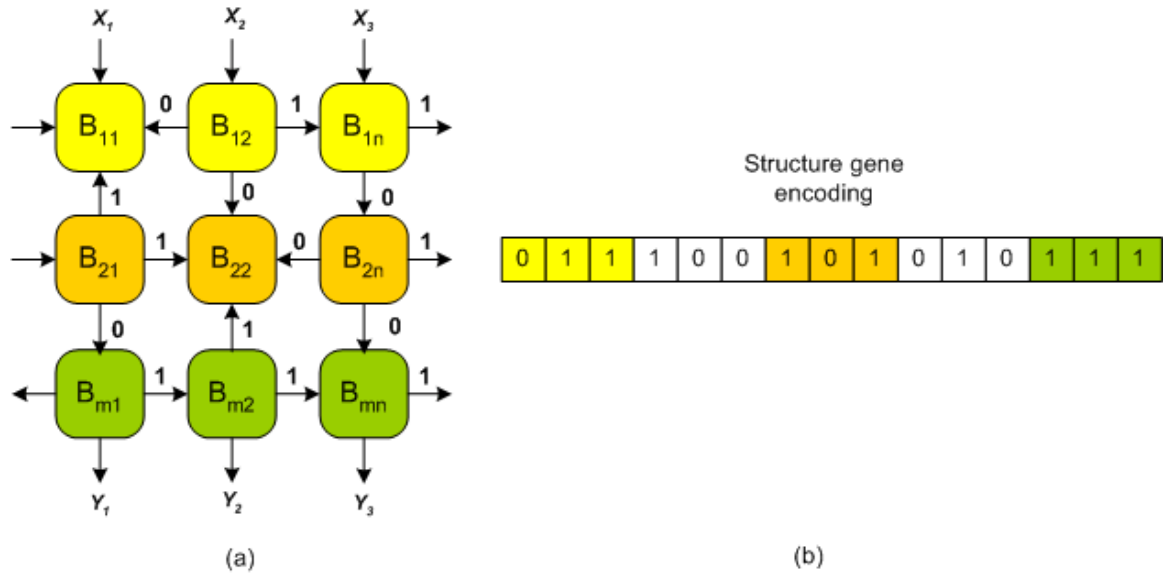
Figure 11 Recurrent BbNN network structure encoding (a) BbNN (b) Structure encoding
