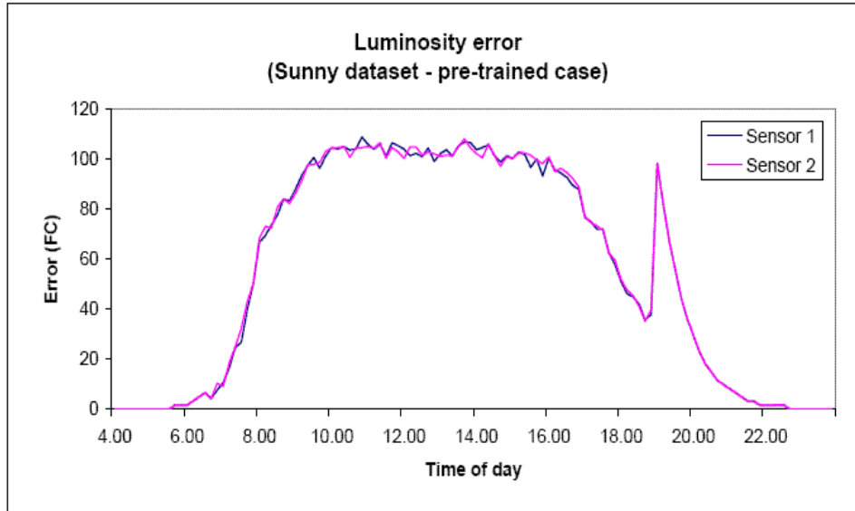
Figure 69 Luminosity error for the sunny dataset - pre-trained case
