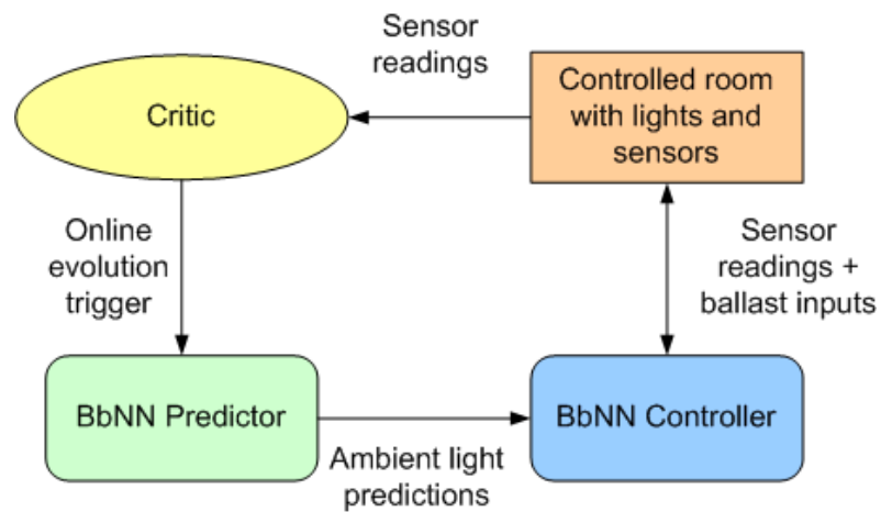
Figure 54 BbNN predictor - controller block diagram
