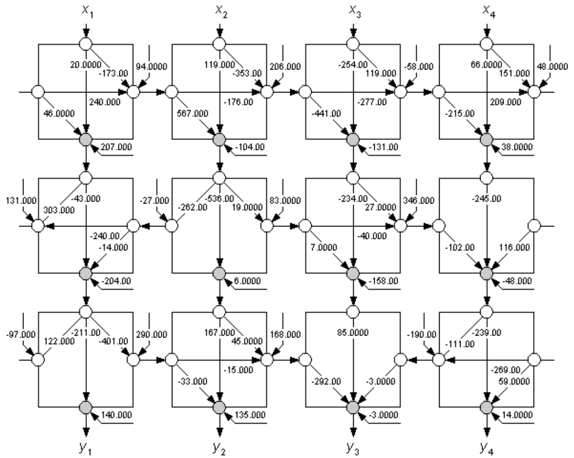
Figure 44 Evolved BbNN after 1557 generations
