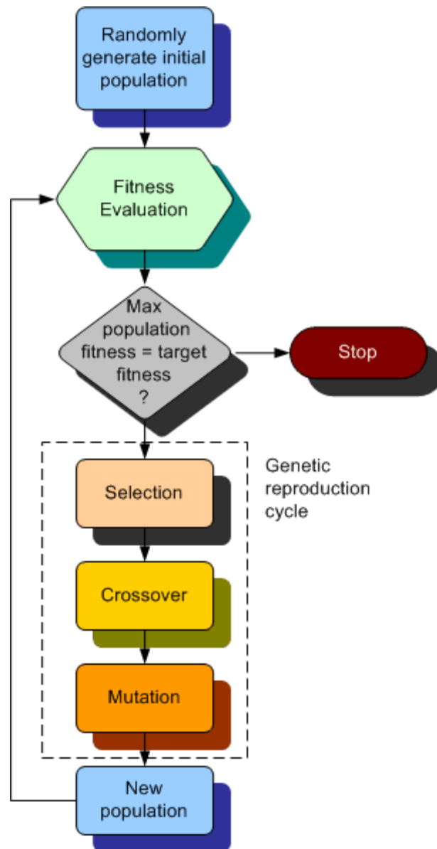
Figure 10 Flowchart depicting genetic evolution process
