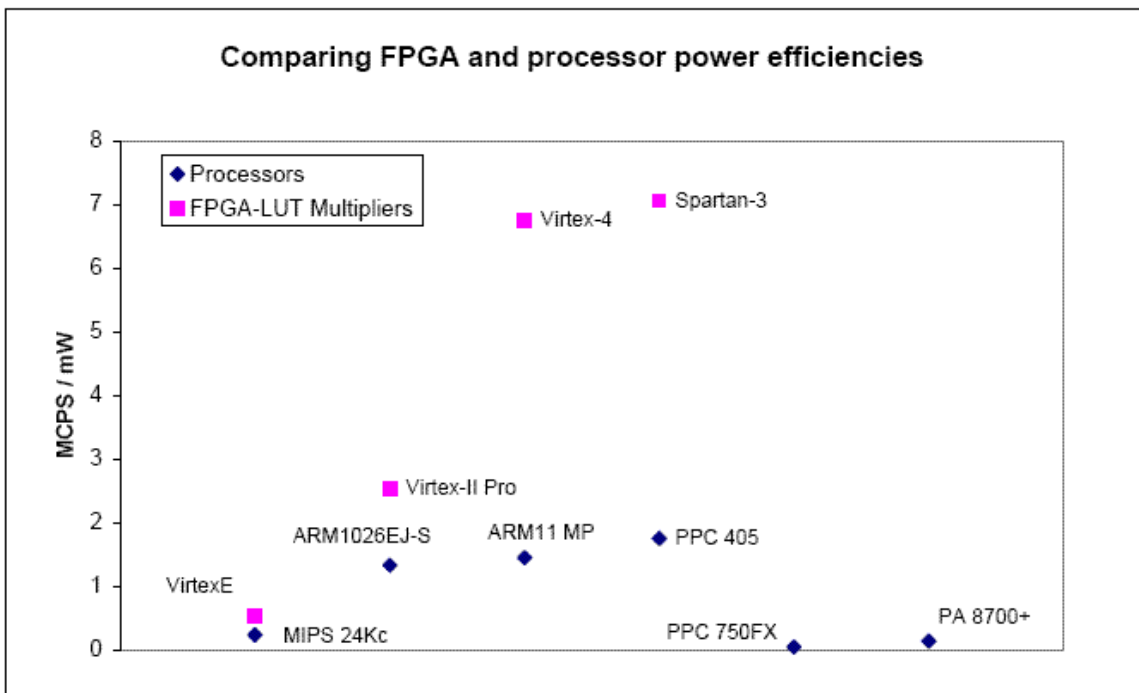
Figure 85 Comparing power efficiencies of processors and FPGAs (LUT Multiplier)
