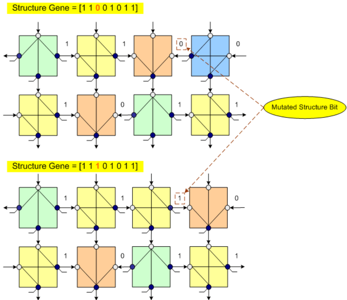
Figure 16 Structure mutaiton operation in BbNN
