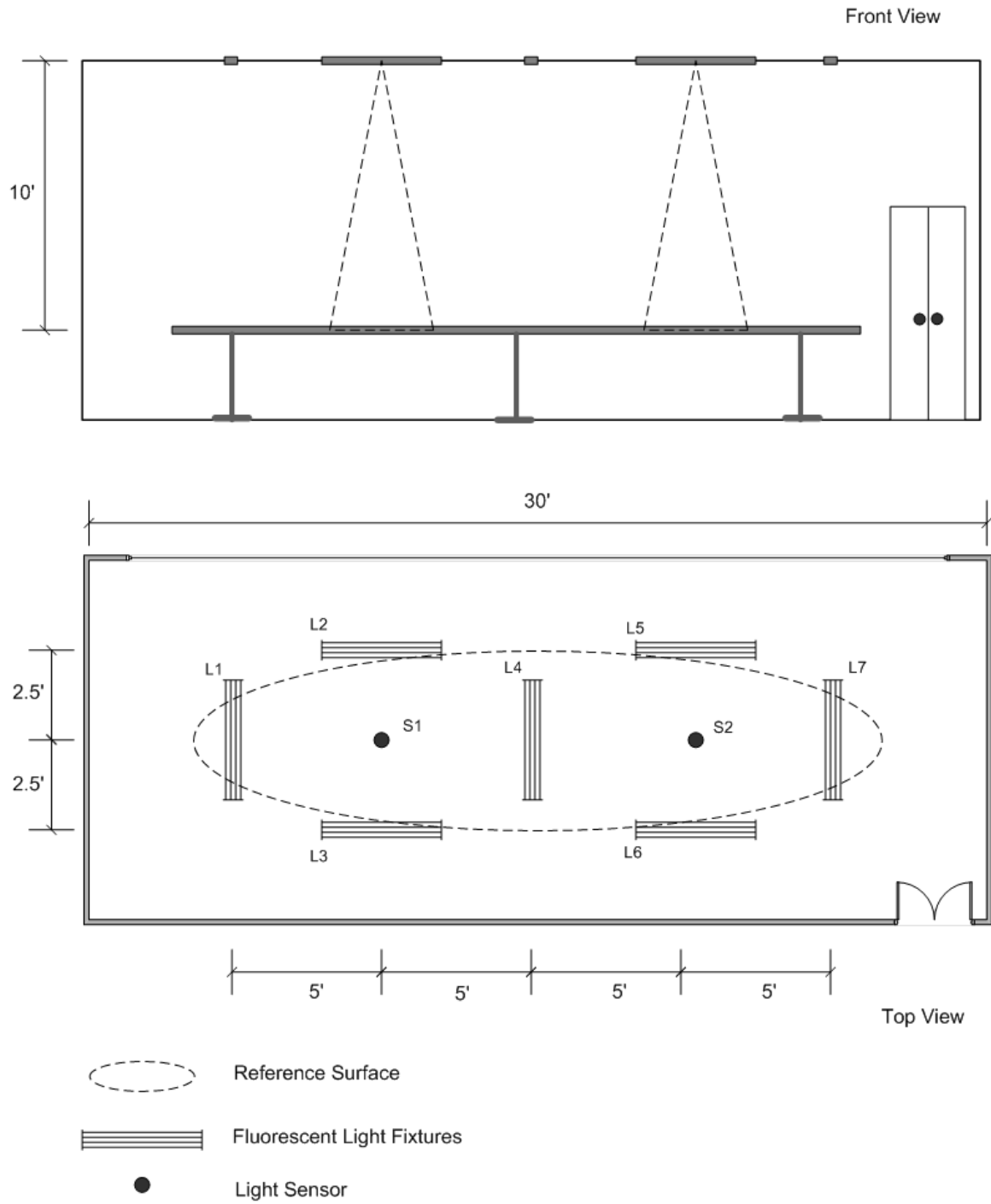
Figure 37 Layout of the reference room used for simulation
