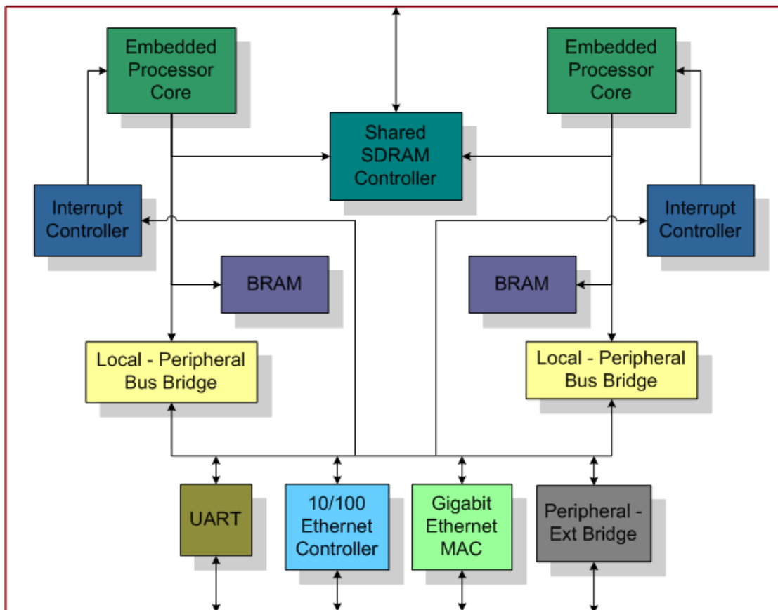
Figure 24 Programmable System on a Chip - logical diagram
