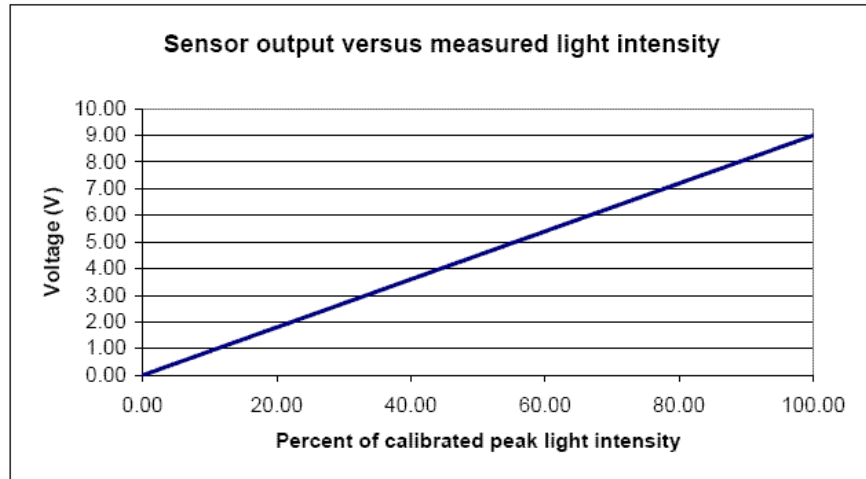
Figure 39 Plot of sensor signal output (V) versus measured light intensity (in percent of calibrated peak intensity)
