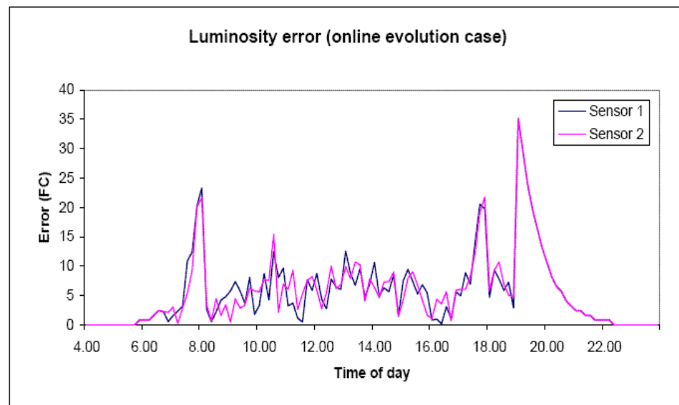
Figure 58 Error between target and measured luminosities (online evolution case)
