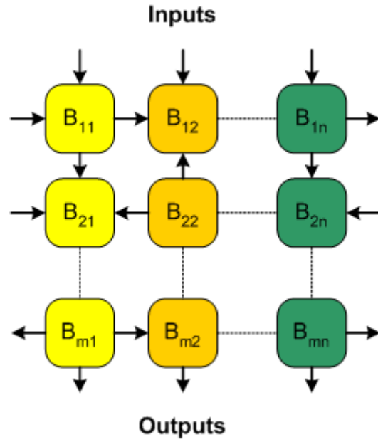
Figure 7 Block-based Neural Network topology
