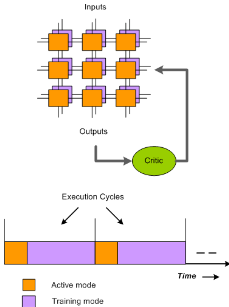
Figure 33 Single network scheduled to switch between training and active modes
