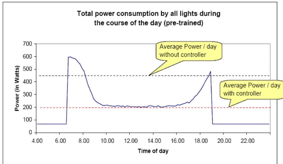
Figure 59 Power consumption (pre-trained case)
