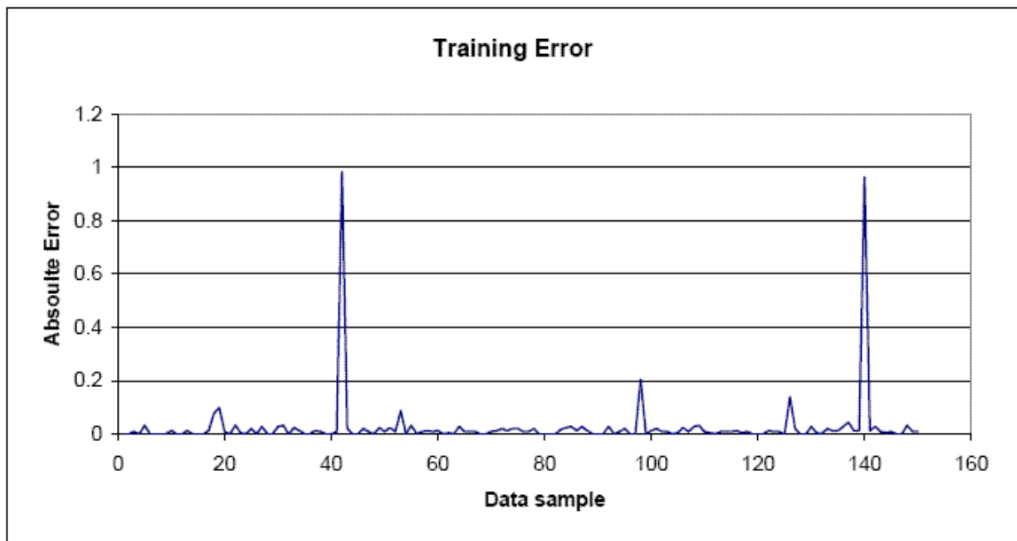
Figure 29 BbNN training error for Iris plant classification database. Results show less than 1.5% misclassification rate
