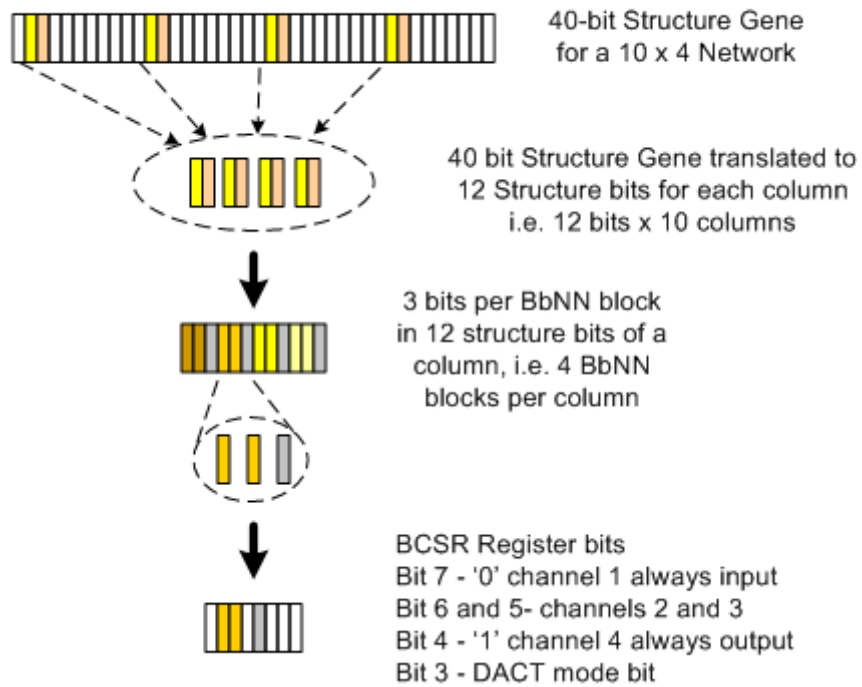
Figure 20 Dynamic gene translation logic for internal configuration emulation
