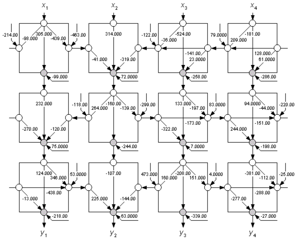
Figure 53 Evolved network after the second re-training cycle
