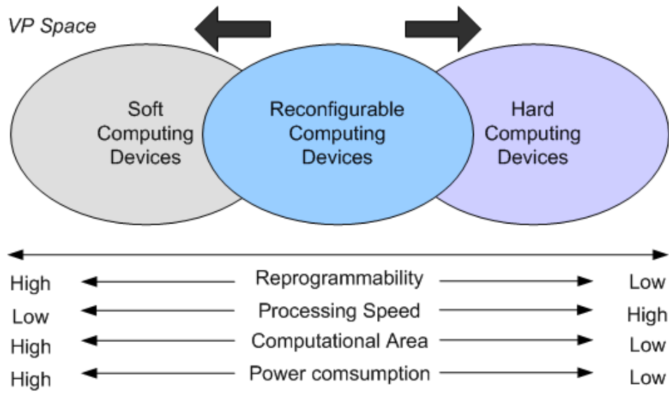
Figure 74 Reorganization of the VP space with advances in RP device technologies
