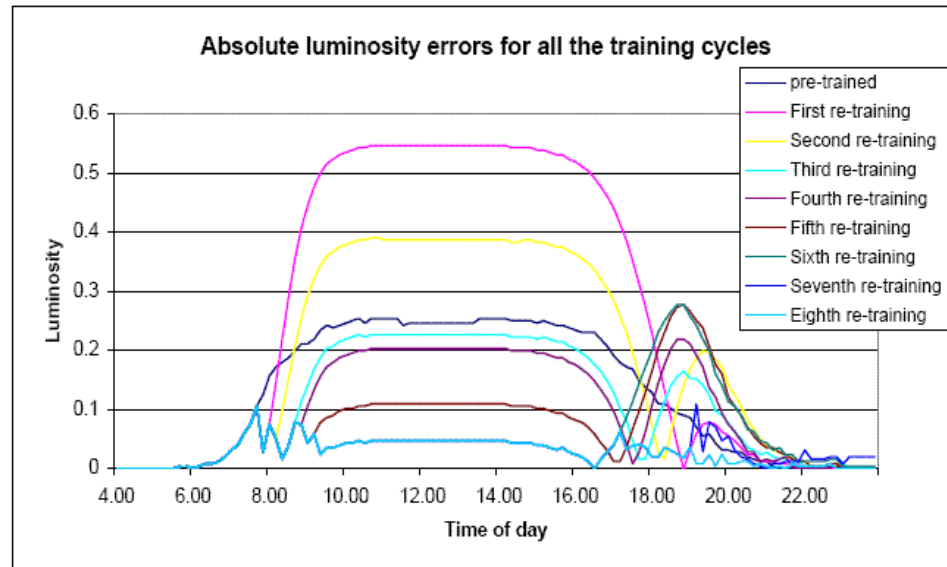
Figure 64 Prediction errors of all the re-training steps. The errors curves show the prediction errors assuming the subsequent re-training cycles are not triggered
