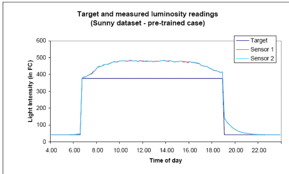
Figure 68 Target and measured luminosity reading for the sunnydataset - pre-trained case
