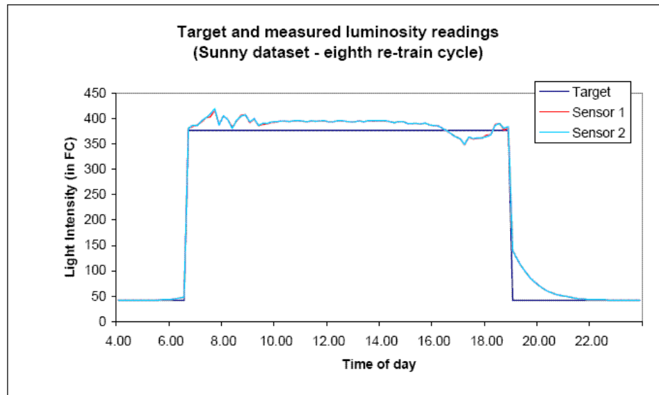
Figure 70 Target and measured luminosity readings for the sunny dataset with all eight re-train cycles
