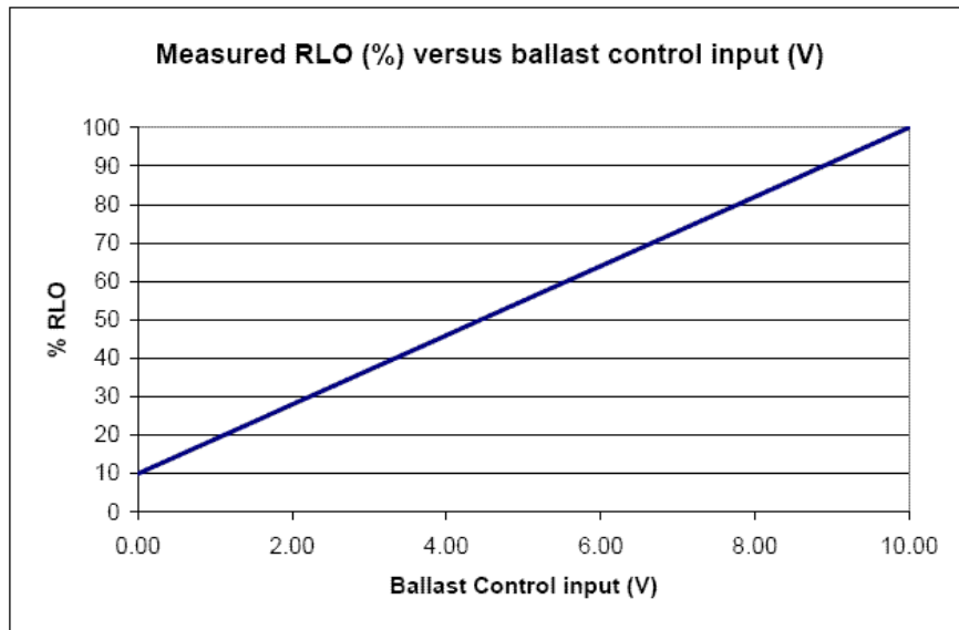
Figure 38 Plot of measured relative light output (%) versus ballast control input
