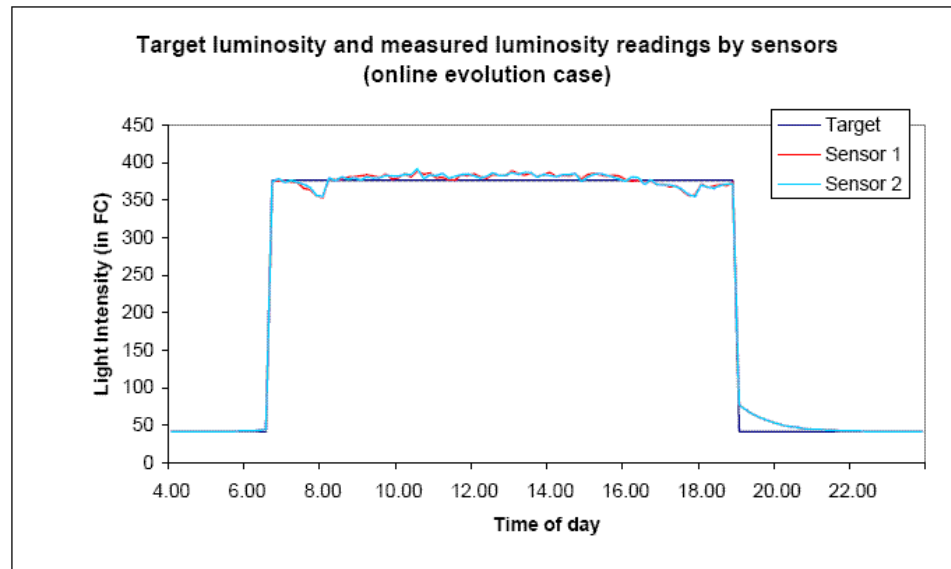
Figure 57 Target and measured luminosity levels as recorded by the light sensors (online evolution case)
