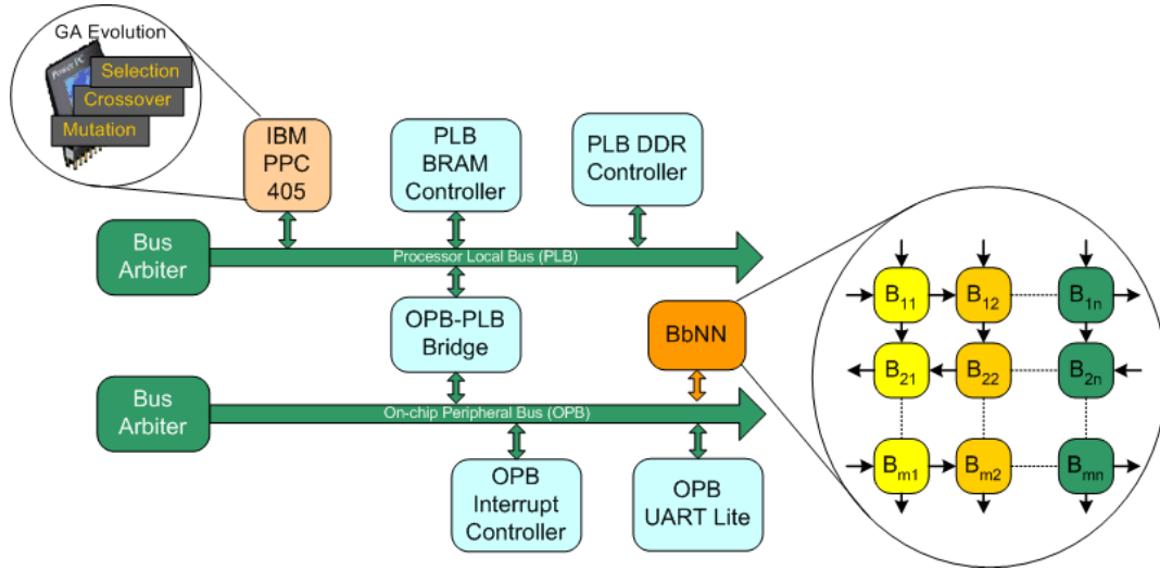
Figure 25 BbNN PSoC platform. GA operators execute on PPC405, Fitness evaluation done using hardware BbNN design
