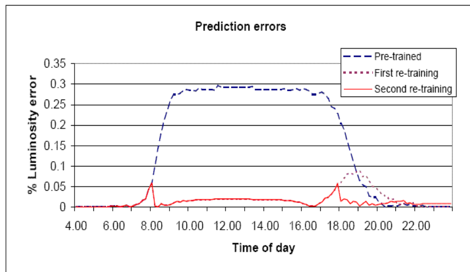
Figure 49 Prediction errors for pre-trained, first re-training, and second re-training cycles
