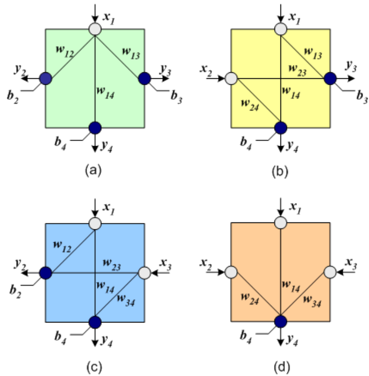
Figure 8 Four different internal configurations of a basic neuron block (a) 1/3 (b) 2/2 (left) (c) 2/2 (right) (d) 3/1 configurations
