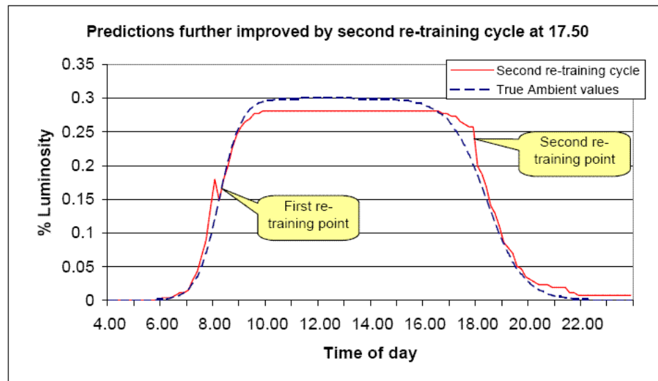
Figure 48 Predictions improve after the second re-training cycle at 17:50
