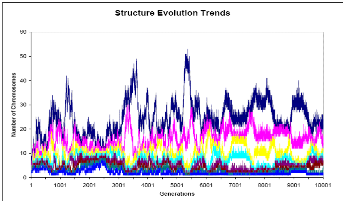
Figure 31 Structure evolution trends for Iris plant classification using BbNN
