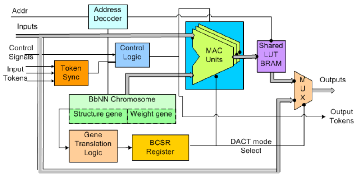
Figure 23 SBbN neuron logical block diagram
