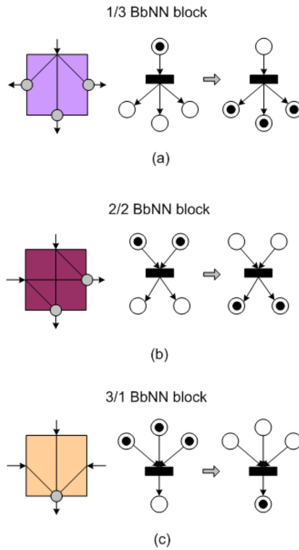
Figure 21 Equivalent Petri Net models for BbNN blocks (a) 1/3 (b) 2/2 (c) 3/1
