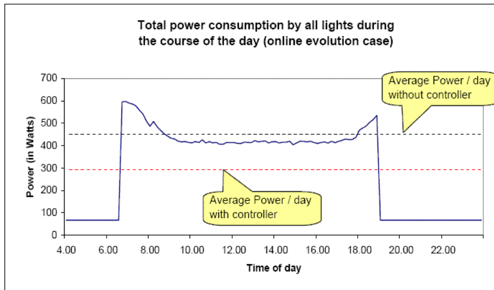
Figure 60 Power consumption (online evolution case)
