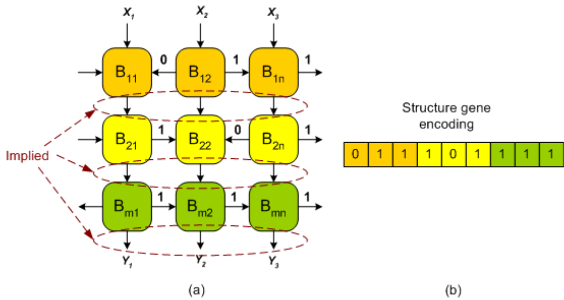
Figure 12 Feedforward BbNN network structure encoding (a) BbNN (b) Structure encoding
