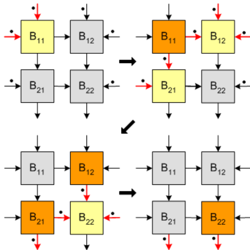
Figure 22 An example 2 x 2 BbNN firing sequence
