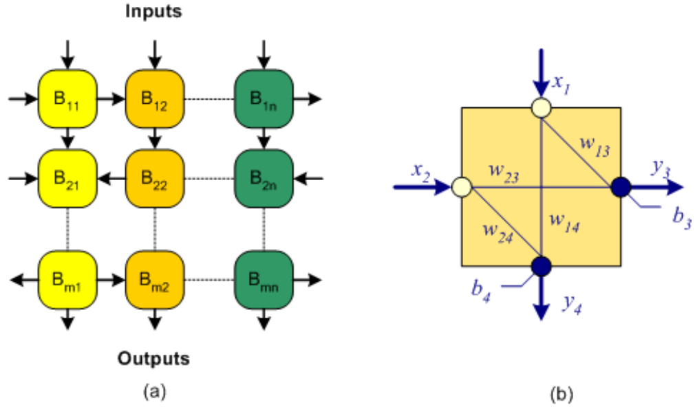
Figure 2 (a) Block-based neural network topology (b) 2 input / 2 output neuron block configuration
