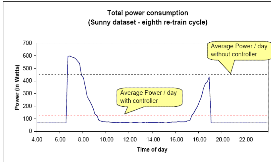
Figure 73 Total power consumption with sunny dataset - eight re-training cycles
