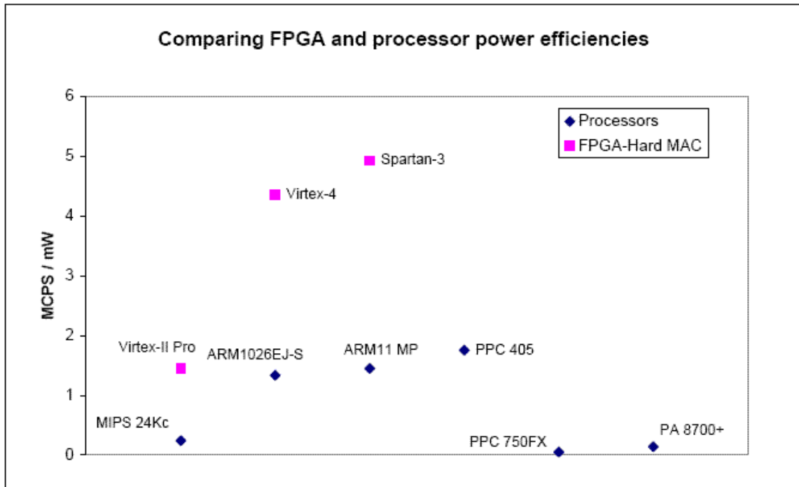
Figure 82 Comparing power efficiencies of processors and FPGAs (Hard MAC)
