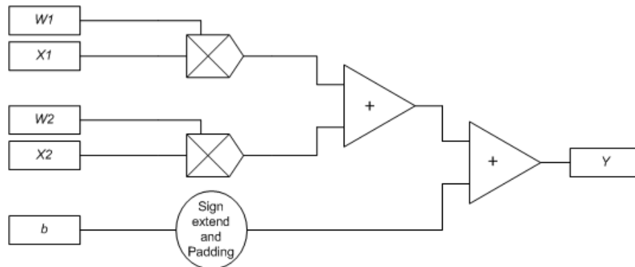
Figure 77 Pipelined parallel multiplier circuit for neural processing
