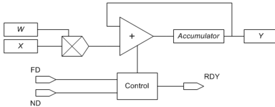
Figure 76 Pipelined multiplier accumulator circuit for neural processing
