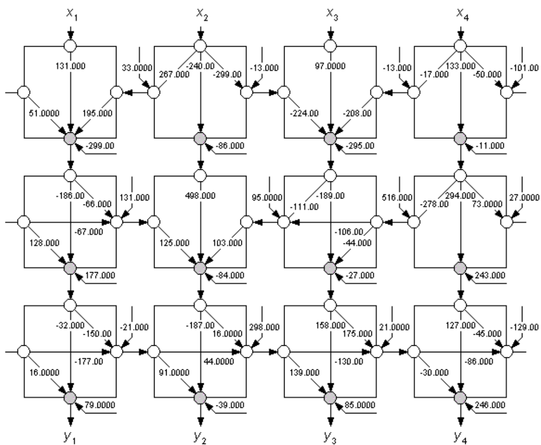
Figure 67 Evolved BbNN network after eighth re-training cycle
