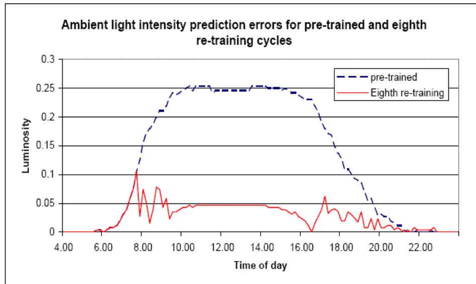
Figure 65 The plot shows the prediction errors for the eighth re-training cycle and the pre-trained case
