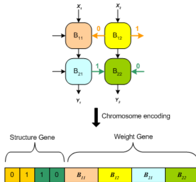
Figure 14 BbNN chromosome encoding for a 2 x 2 network
