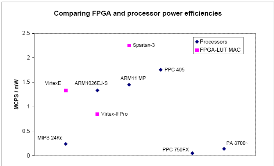
Figure 83 Comparing power efficiencies of processors and FPGAs (LUT MAC)
