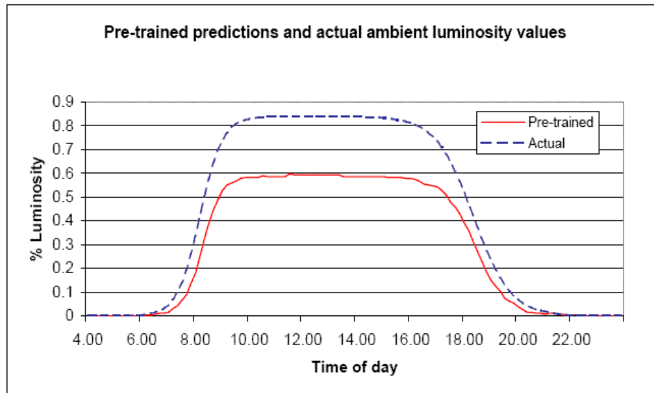
Figure 62 Actual and pre-trained predictions of ambient light intensity
