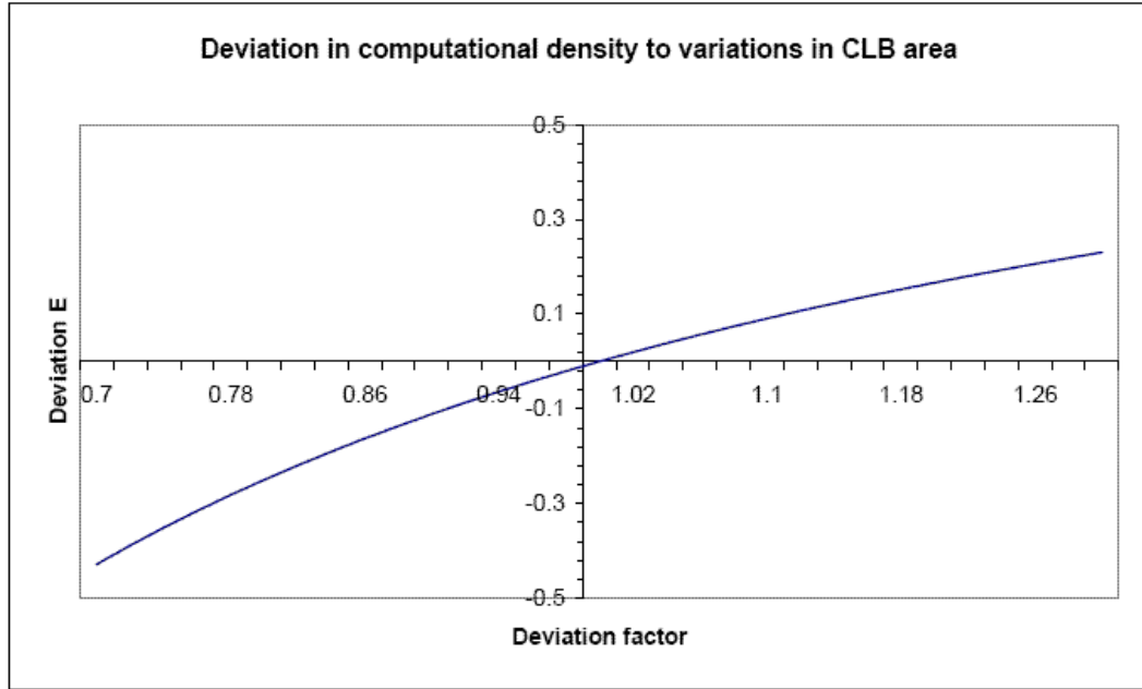
Figure 87 Deviation in computational density verses die area deviation factor
