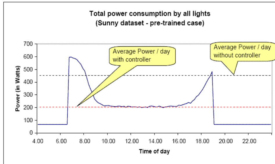
Figure 72 Total power consumption for sunny case - pre-trained case
