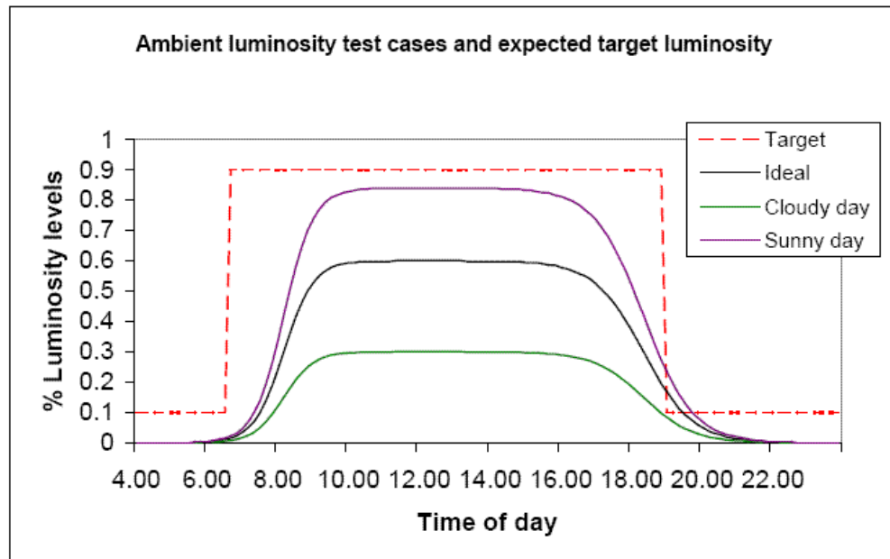
Figure 45 Ambient luminosity test cases and expected target luminosity
