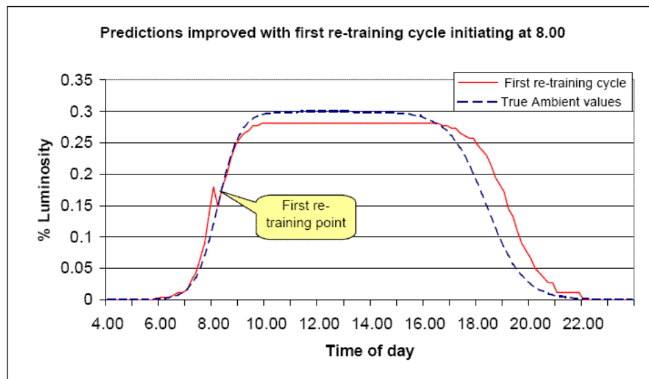
Figure 47 Predictions improve after first re-training cycle at 8:00
