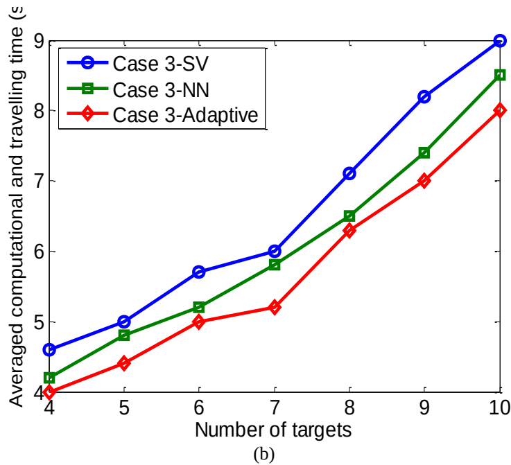
Figure 9.9 Averaged computational and traveling time for sequential visiting (SV), nearest neighbor (NN), and adaptive methods under different scenarios: (a) cases 1 and 2 and (b) case 3. In both case 1 and 2, our adaptive algorithm produces a performance closer to the one that requires less computational and traveling time. Case 3 resembles the practical surveillance application. Our adaptive algorithm requires the least computational and traveling time.
