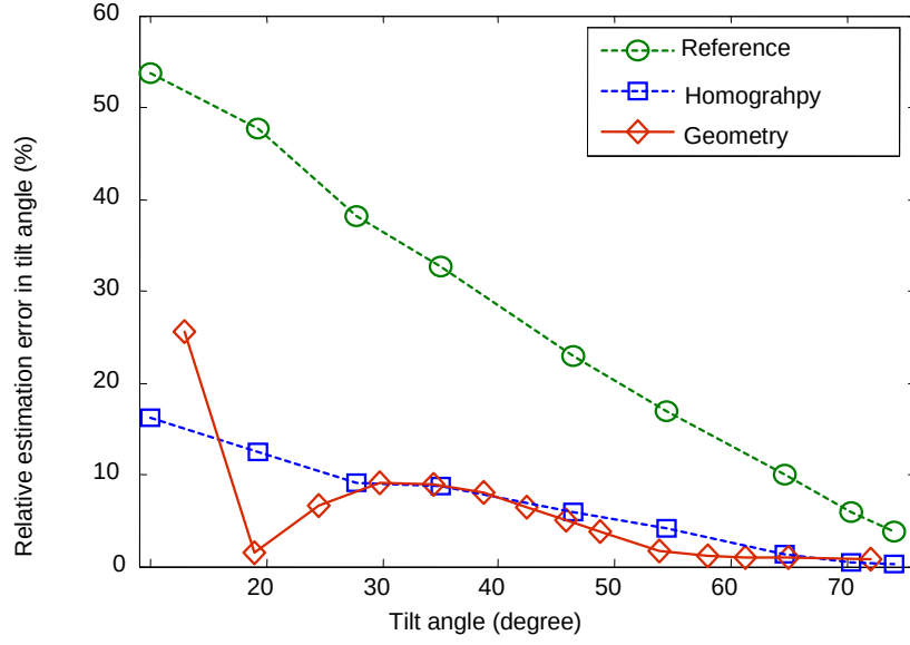
Figure 9.2 Performance comparison between our algorithm and the reference algorithm [Cui98] based on relative errors in the estimated \hat{\theta}_T . The reference algorithm uses a fixed model and suffers from over-fitting problem due to noisy data.
