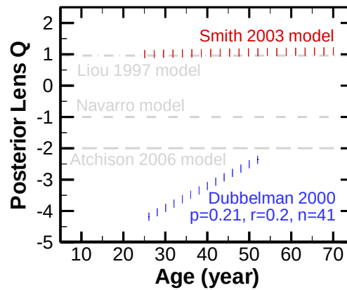
Figure 2.50 Comparison of age-dependence in Q_4 studies
