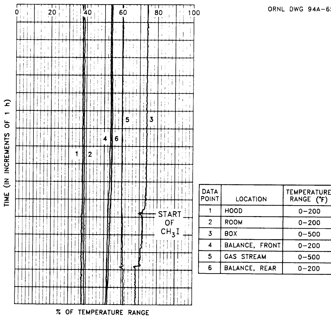
Figure 5.7. Temperature fluctuation observed for run T14 at time of \text{CH}_3\text{I} addition to gas stream.
