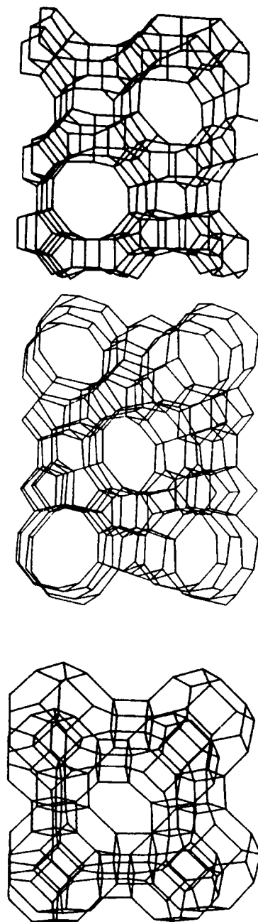
Figure 2.3. Pore structure of commercial zeolites. Redrawn with permission after Figure 4, p. 27, D. E. W. Vaughan, "The Synthesis and Manufacture of Zeolites," Chemical Engineering Progress , Vol. 84, No. 2, p. 25-31, February 1988, American Institute of Chemical Engineers.
