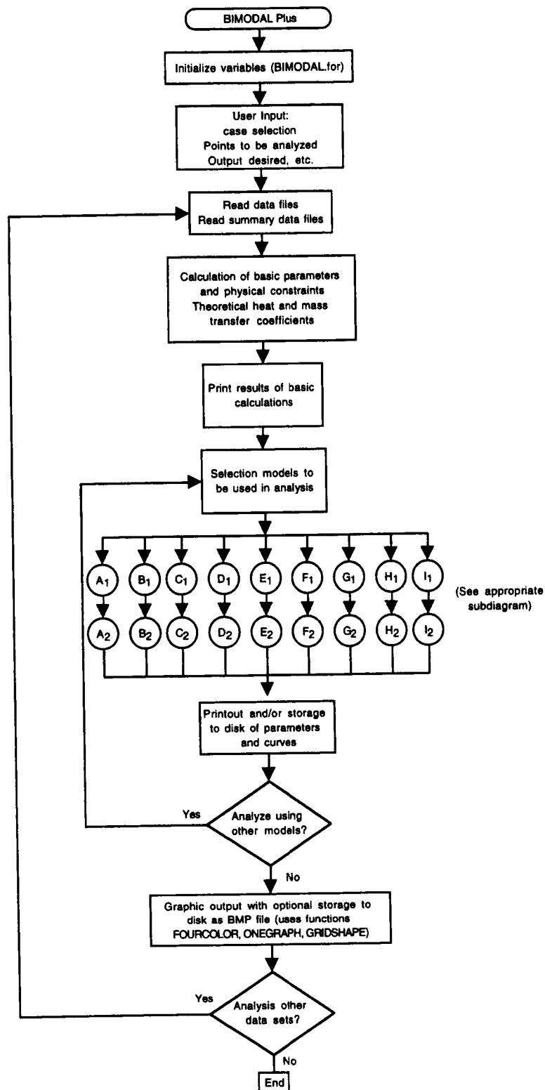
Figure 5.5. Flow chart to BIMODAL Plus FORTRAN code for fitting model parameters to experimentally obtained loading curves.
