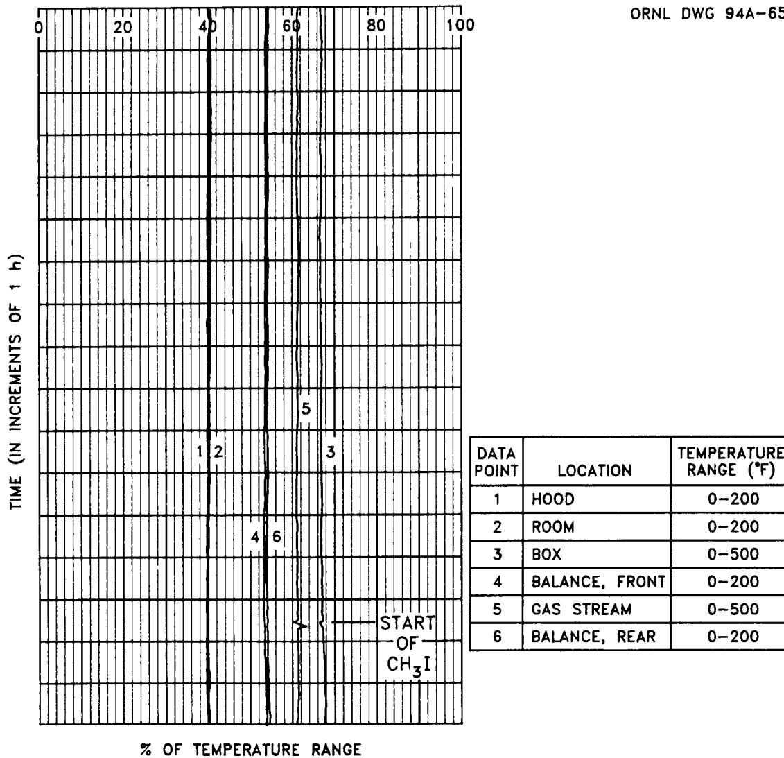
Figure 5.6. Typical temperature control performance as observed in Run T8.
