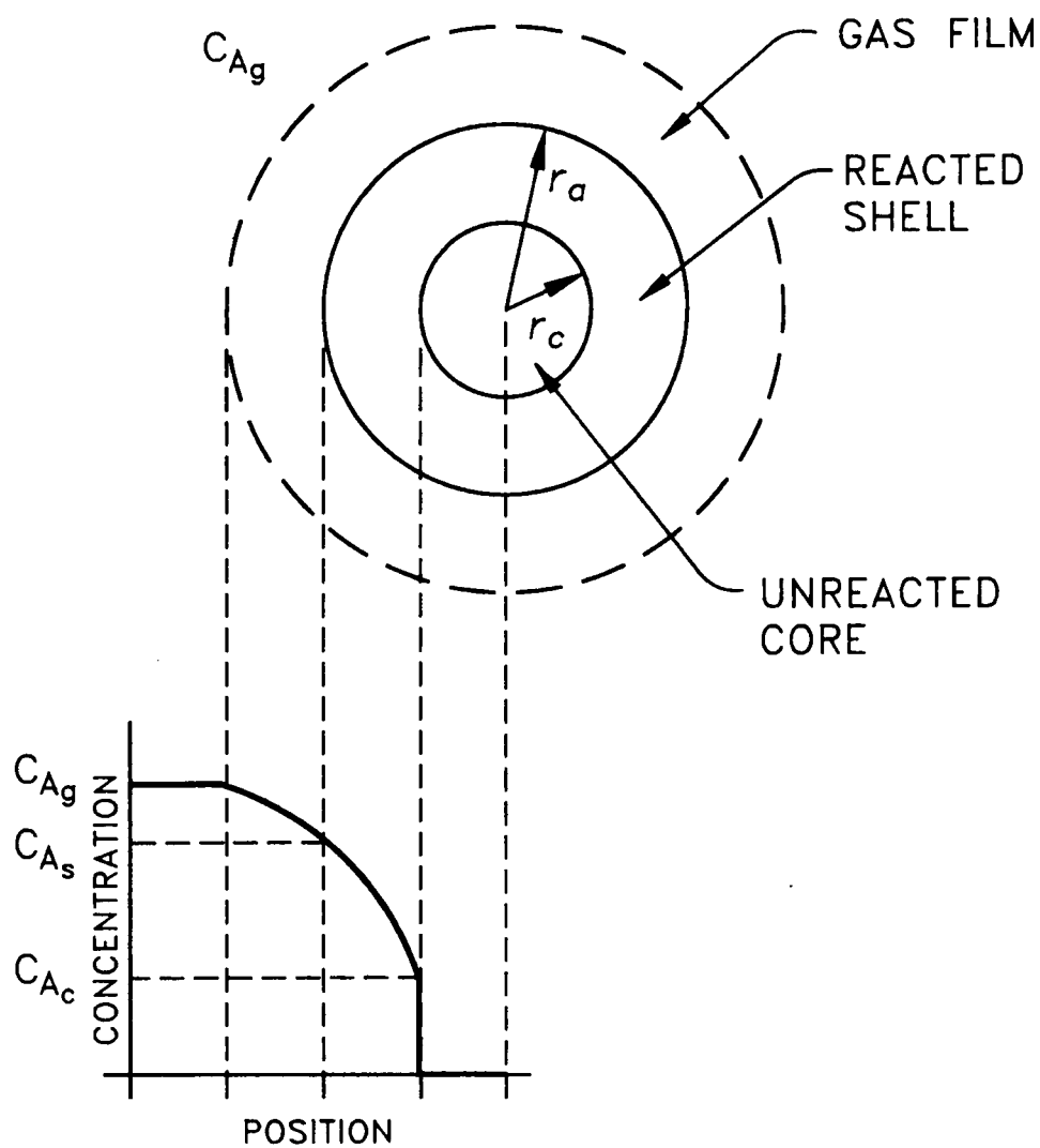
Figure 2.4. Schematic representation of the shrinking core model. Adapted with permission from Figure 4, p. 362, O. Levenspiel, Chemical Reaction Engineering , Second Ed., John Wiley & Sons, Inc., New York, (1972).
