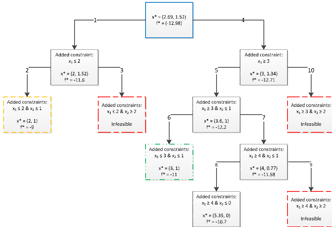
Figure 2.4: Example 2.5 - Branch and Bound Method Diagram
