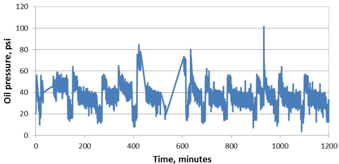
Figure 4.51: Stock engine (compression) oil pressure over time for base oil
