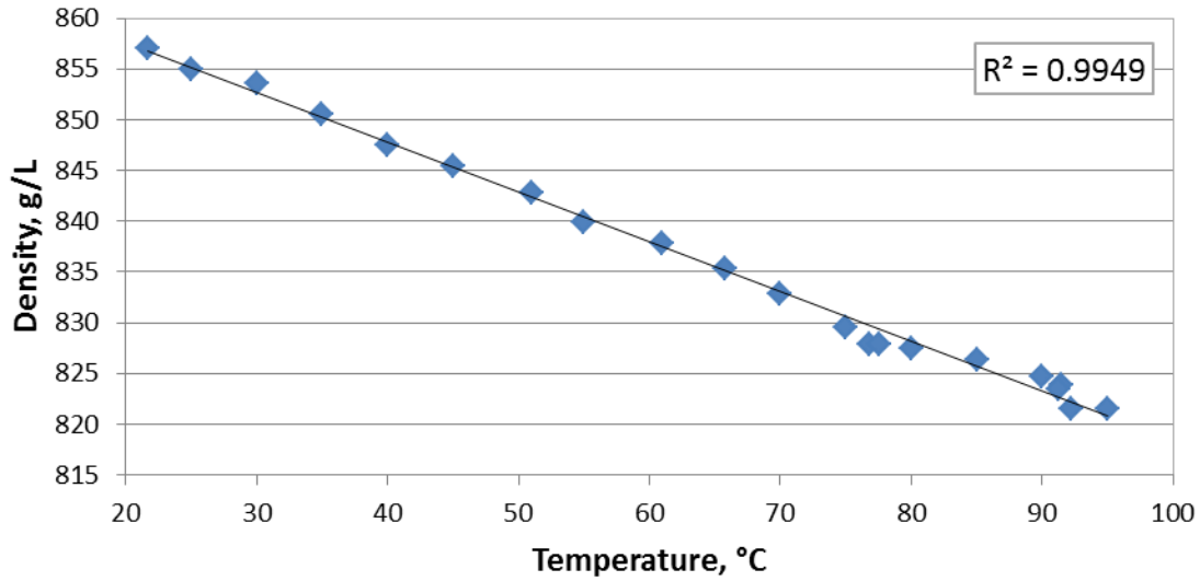
Figure 4.17: Effect of temperature on density for Mobil-1 15W50 lube oil
