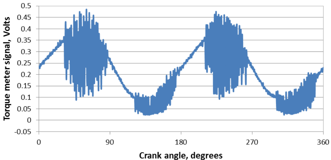
Figure 4.7: Instantaneous torque with torque meter excited by AC/DC converter
