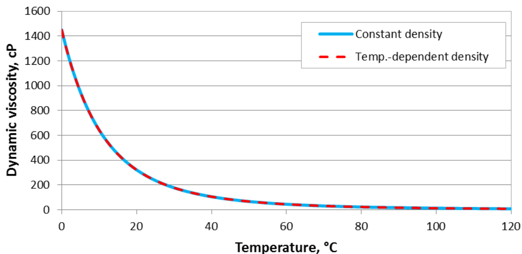
Figure 4.18: Comparison of viscosity temperature relationship calculated with Vogel's equation for constant and temperature-dependent density
