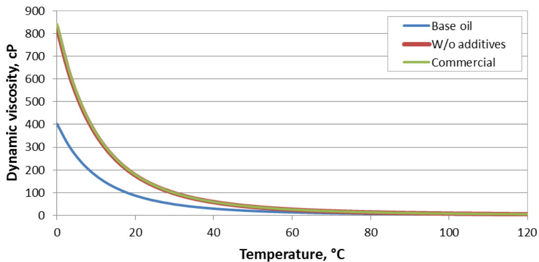
Figure 4.23: Vogel predicted viscosities for Chevron 10W30 in three different stages of production
