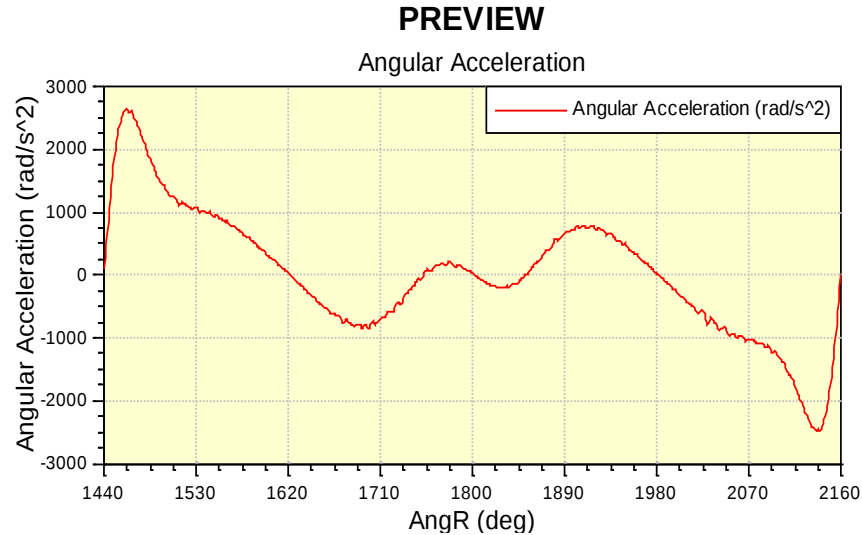
Figure 3.22: Excite crankshaft output based on compression pressure trace
