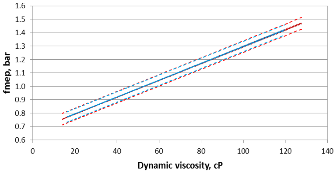
Figure 4.47: Comparison of linear fits for 5W30 tests with oil changes (red) and without oil changes (blue) with confidence and prediction intervals
