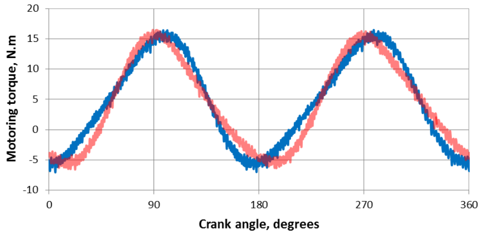
Figure 4.26: Instantaneous torque curves measured approximately 3 seconds apart for modified engine with internal oil pump (no compression) with the Cooper instruments torque meter and a 15W40 weight oil
