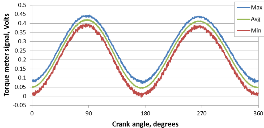
Figure 4.8: Instantaneous torque with torque meter excited by 12 VDC battery and averaged over 300 crankshaft revolutions
