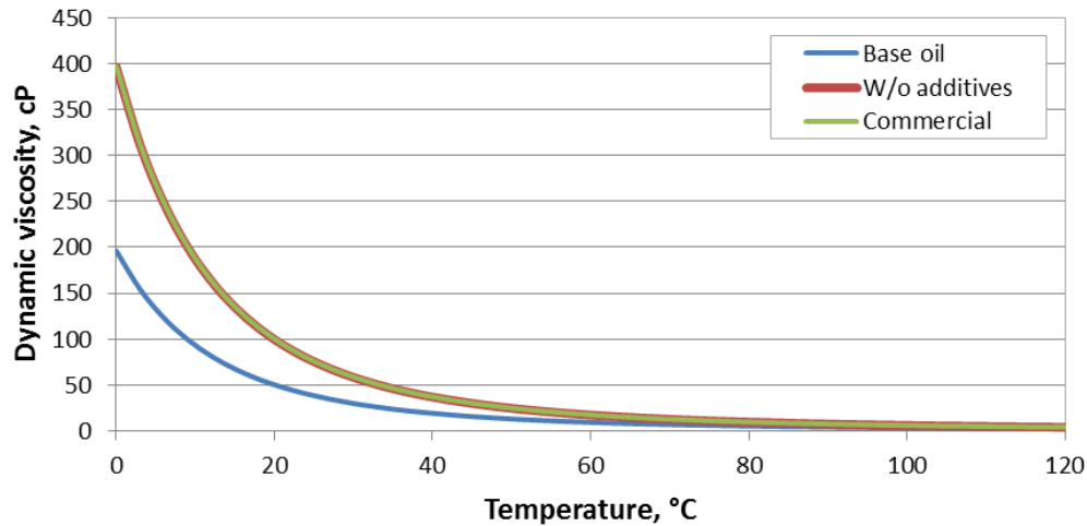
Figure 4.22: Vogel predicted viscosities for Chevron 5W20 in three different stages of production
