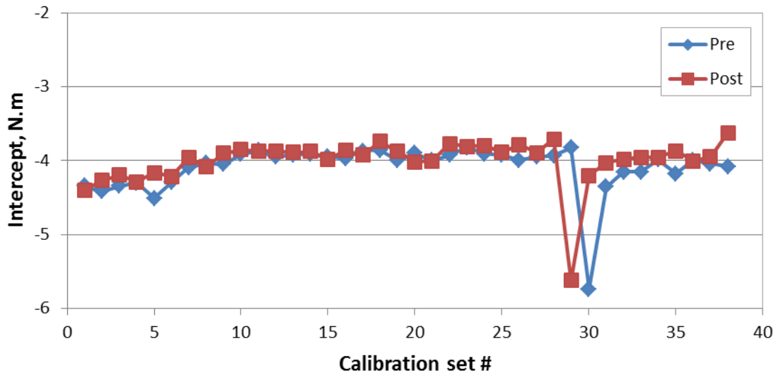
Figure 4.11: Cooper instruments calibration equation y-intercept over time
