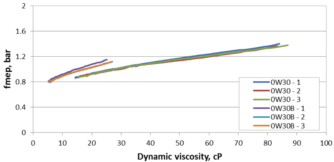
Figure 4.49: Friction mean effective pressure for 0W30 oil and its base oil measured on modified engine with external oil pump using Omega torque meter
