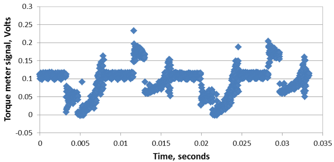
Figure 4.4: Signal from torque meter when powered by A/D converter sampling at 60 kHz
