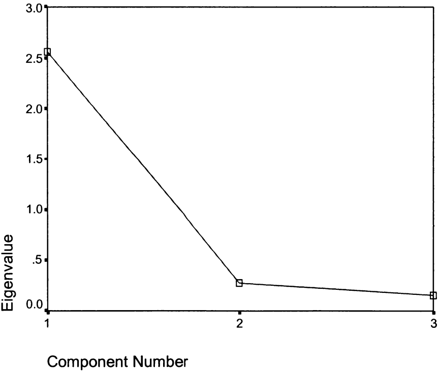
Scree Plot
