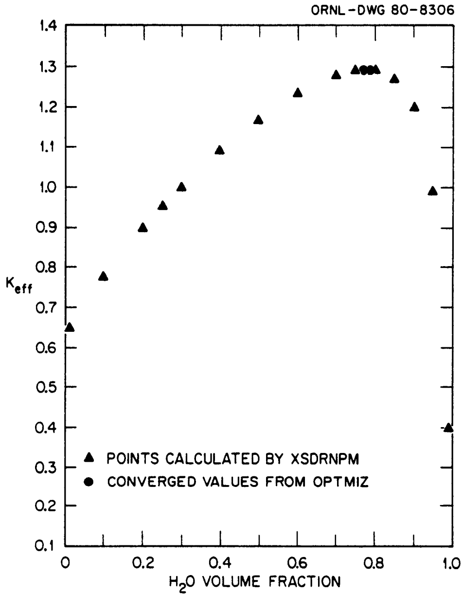
Figure 12. Curve of K-effective Versus Pitch for a Cylindrical Tank of 4% Enriched UO_2 Powder Mixed with Water.
