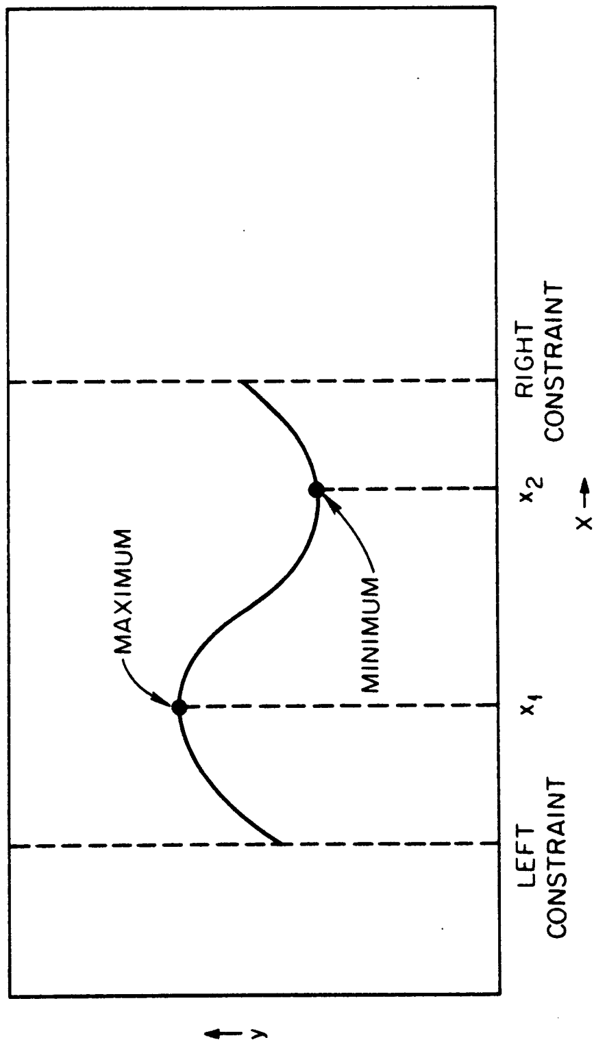
Figure 5. The Maximum and Minimum Points of a Cubic with Two Local Extrema.
