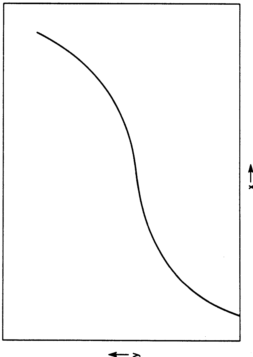
Figure 2. A Cubic with No Local Extrema.
