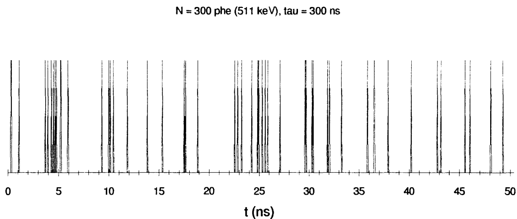
Figure 3-8. Monte Carlo Simulated Photoelectron Emissions for BGO/Photomultiplier Scintillation Detector.
