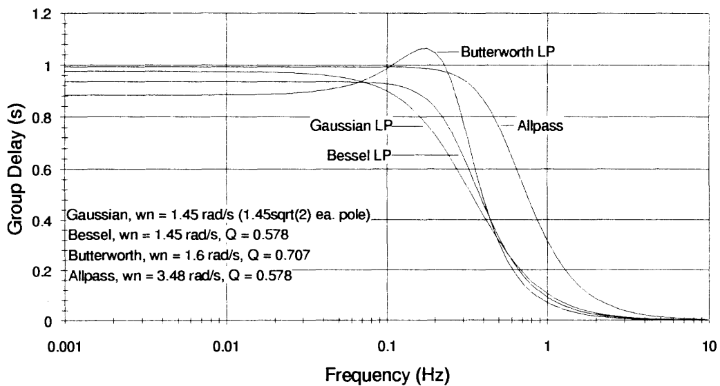
Figure 4-9. Group Delay of Second-Order Lowpass, Allpass Delay-Line Approximation Filters.
