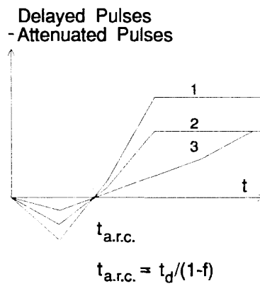
Figure 1-5. Illustration of CFD Operation for Linear-Edge, Flat-Top Pulses.
