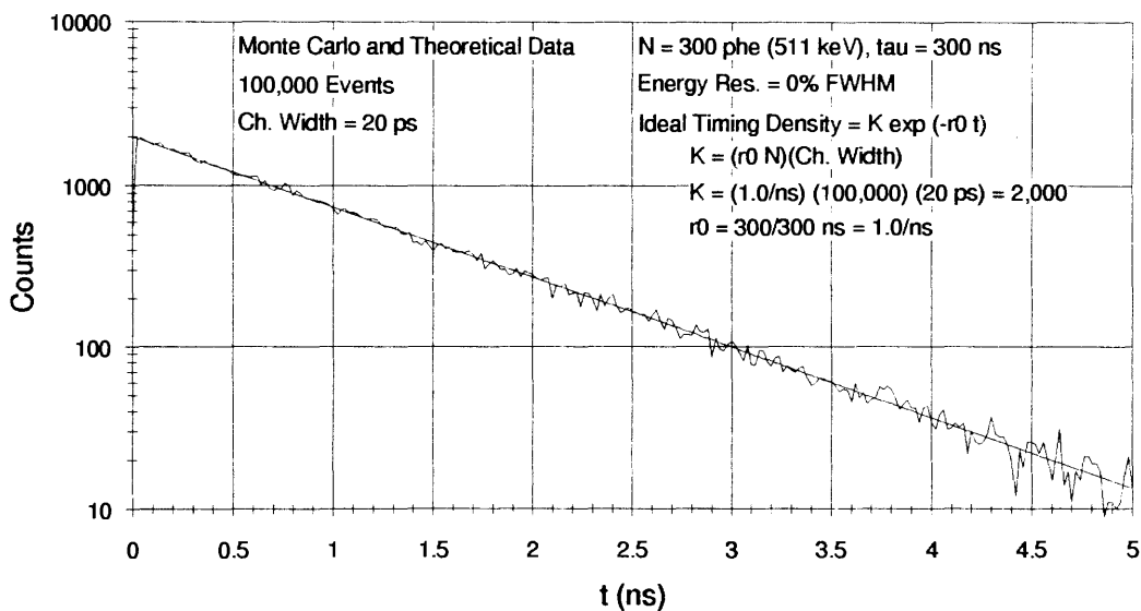
Figure 3-11. Comparison of Monte Carlo Simulated First-Photoelectron Timing Spectrum with Theoretical Poisson Timing Spectrum.
