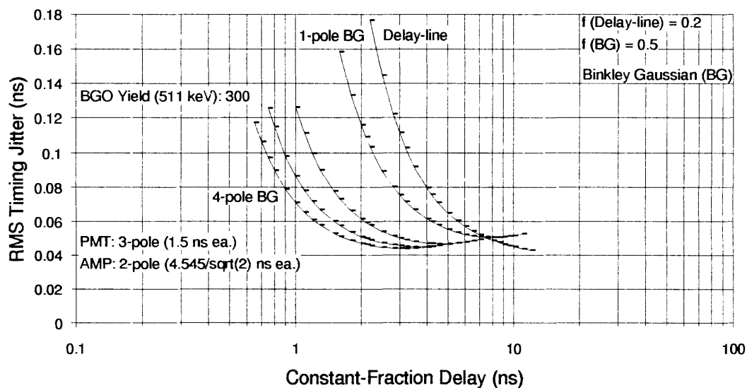
Figure 4-29. Timing Jitter for Delay-Line and Non-Delay-Line CFDs.
