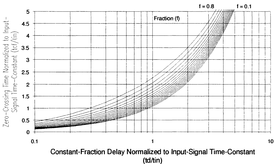
Figure A-2. Delay-Line CFD Zero-Crossing Time for Single-Pole Step Input.
