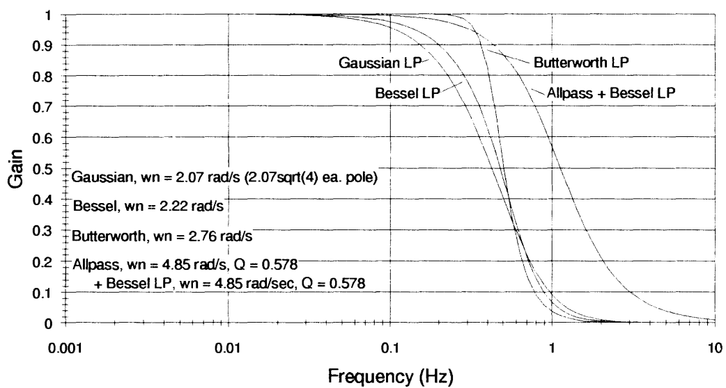
Figure 4-13. Frequency Response of Fourth-Order Lowpass, Allpass Delay-Line Approximation Filters.
