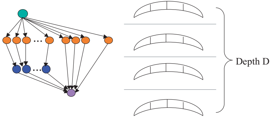
Figure 4.5: An example of greedy multi-level thread scheduling. The DAG is divided into four levels. The level index of each node is equal to the length of the longest path from the root to that node.
