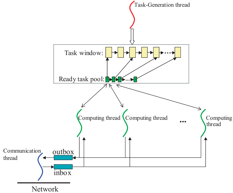
Figure 6.8: Architecture of the runtime system.
