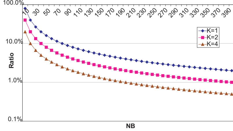
Figure 6.16: \frac{t_{comm}}{kt_{comp}} ratio on Cray XT4.
