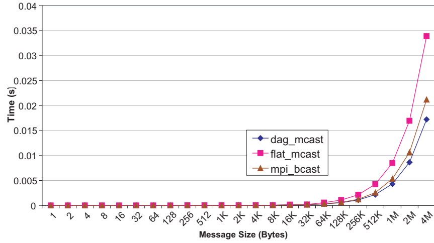
(a) 4 Processes
