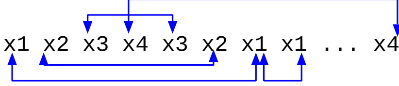
Figure 3.1: An example of a cache block trace containing five circular sequences.
