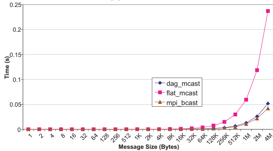
(c) 16 Processes
