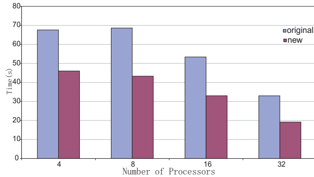
Figure 5.14: CFD kernel on SGI Altix.
