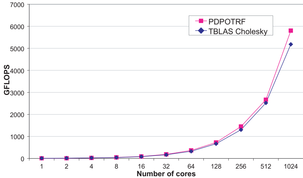
Figure 6.21: Overall performance of Cholesky factorization on Cray XT4.
