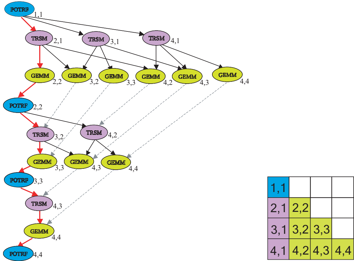
Figure 7.2: Cholesky factorization DAG for a matrix with 4 \times 4 blocks.
