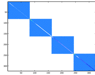
Figure 3.6: Sparse matrix of qc324 ( nnz = 26, 730 ).
