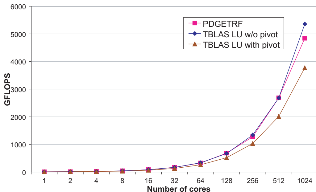
Figure 6.23: Overall performance of LU factorization on Cray XT4.
