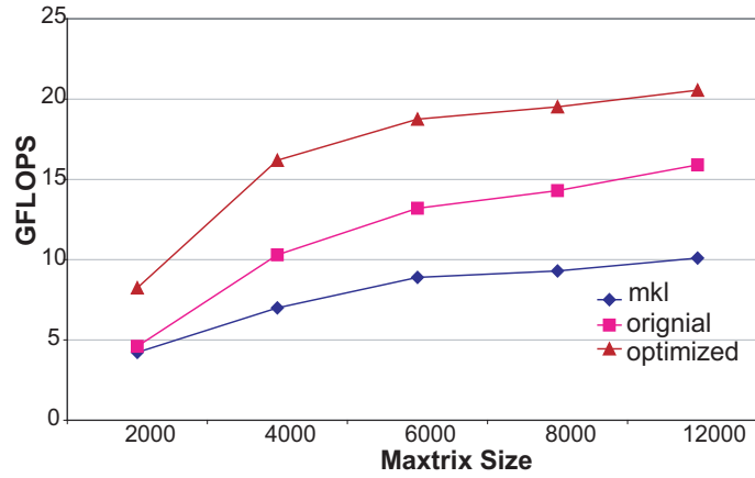
Figure 5.16: Cholesky factorization on SGI Altix with 4 processors.
