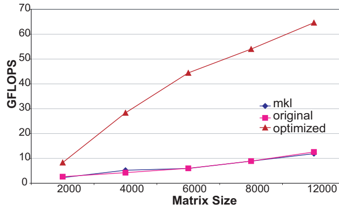
Figure 5.18: Cholesky factorization on SGI Altix with 16 processors.
