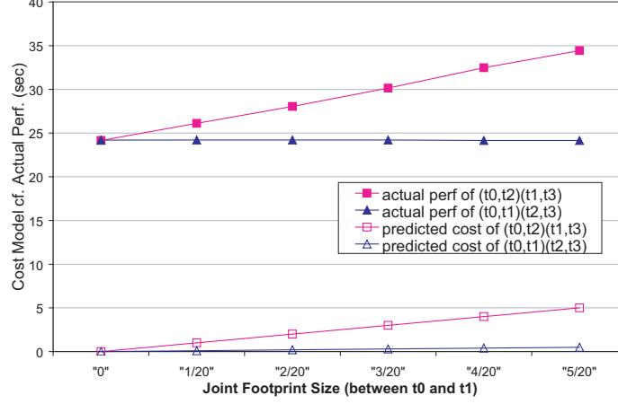
Figure 4.7: Compare the predicted cost to the actual execution time for two schedules: (t_0, t_1)(t_2, t_3) and (t_0, t_2)(t_1, t_3) .
