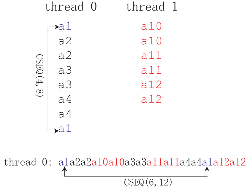
Figure 3.4: A cache hit of thread 0 becomes a miss because of references from thread 1.
