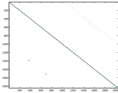
Figure 3.5: Sparse matrix of dw2048 ( nnz = 10, 114 ).
