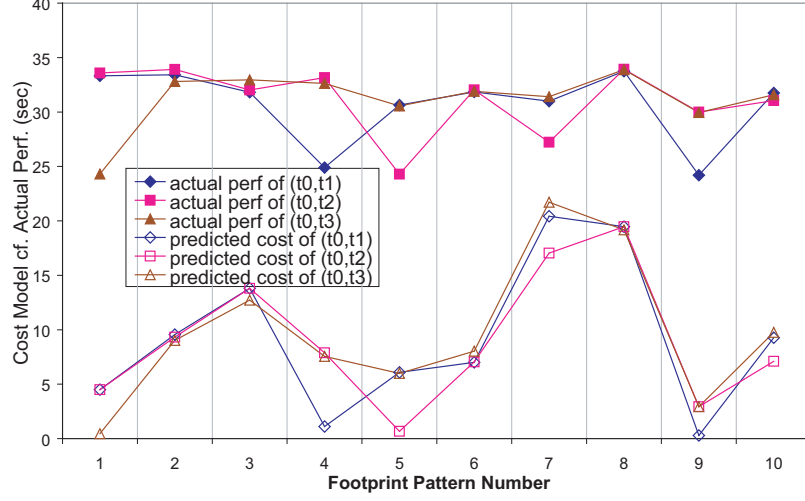
Figure 4.8: Compare the predicted cost to the actual execution time for three thread schedules on 10 randomly generated memory footprint patterns.
