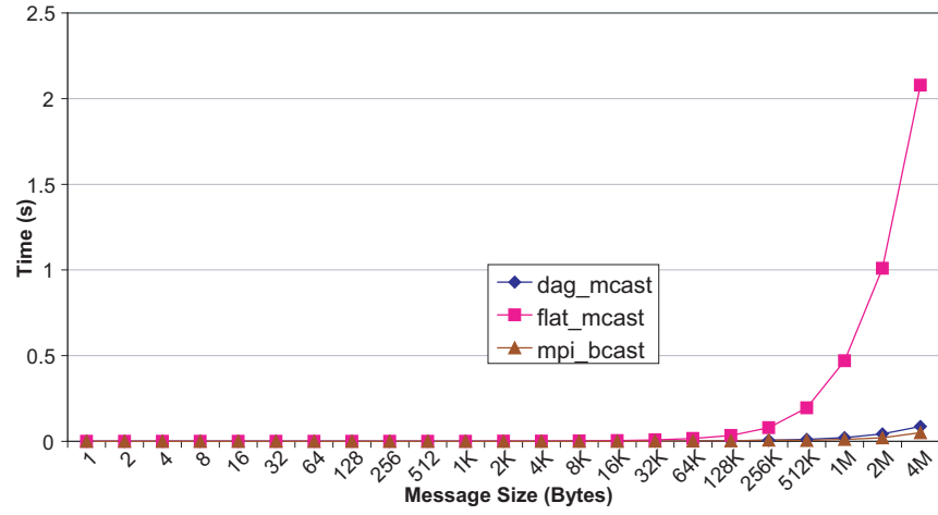
(e) 64 Processes
