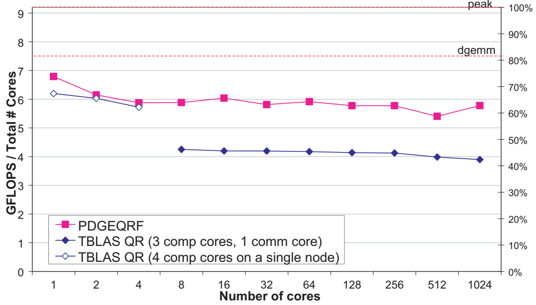
Figure 6.26: Scalability of QR factorization on Cray XT4.
