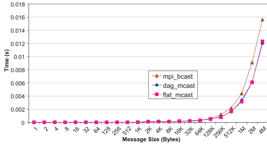
(a) 4 Processes
