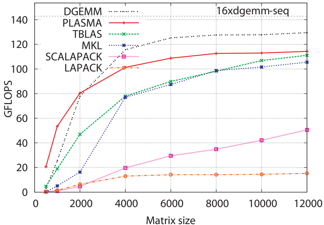
Figure 6.17: Cholesky factorization on a 16-core Intel Tigerton machine.
