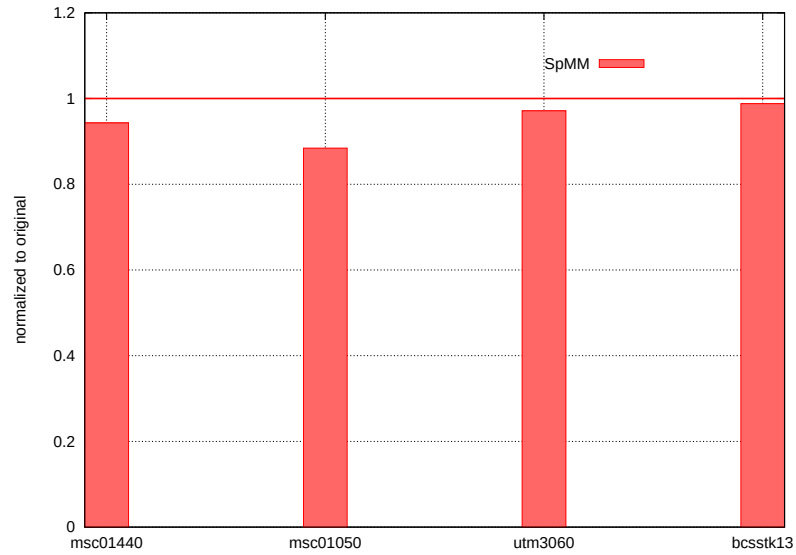
Figure 5.12: SpMM on Intel Clovertown with 8 cores.
