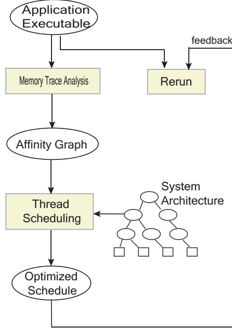
Figure 5.1: Overall structure of the thread scheduling method with memory considerations.
