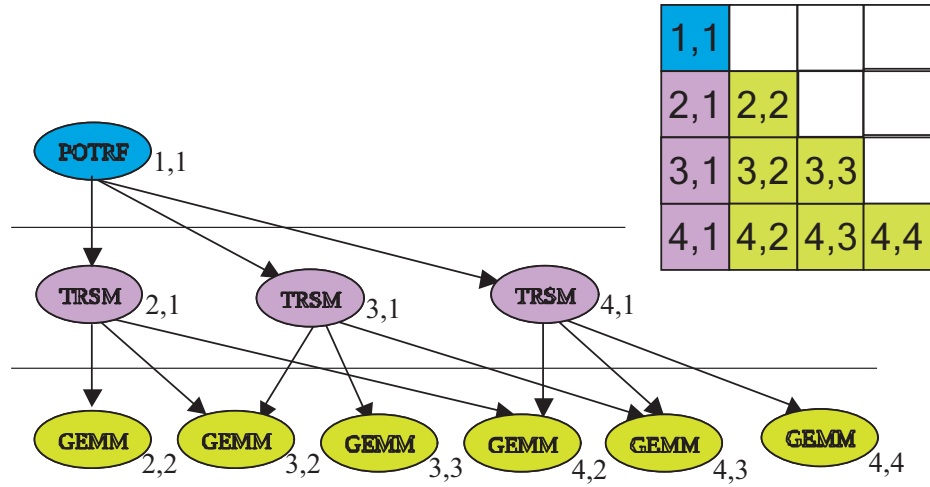
Figure 5.8: Cholesky factorization DAG (one iteration).
