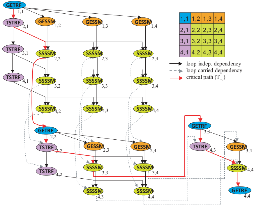
Figure 6.11: DAG for the tiled LU factorization.
