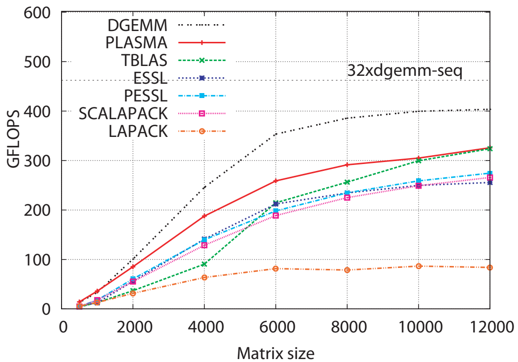
Figure 6.20: QR factorization on a 32-core IBM Power6 machine.
