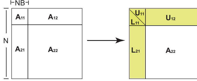
Figure 6.1: Block LU factorization.
