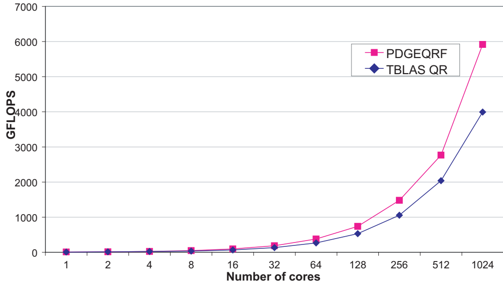
Figure 6.25: Overall performance of QR factorization on Cray XT4.
