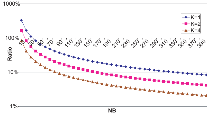
Figure 6.15: \frac{t_{comm}}{kt_{comp}} ratio on a Myrinet cluster.
