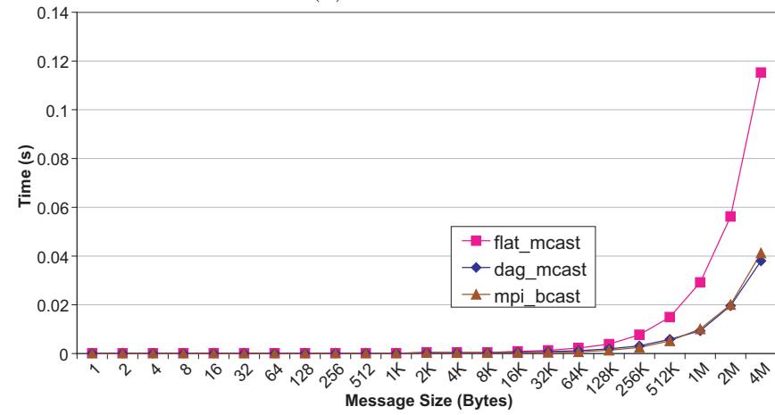
(c) 16 Processes
