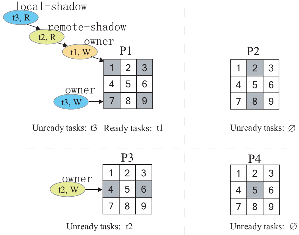
Figure 6.6: Snapshot of the distributed algorithm after four processes have generated tasks t_1 , t_2 , and t_3 in sequence. Assume t_1 reads/writes block 1, t_2 reads block 1 and writes block 4, and t_3 reads block 1 and writes block 7.
