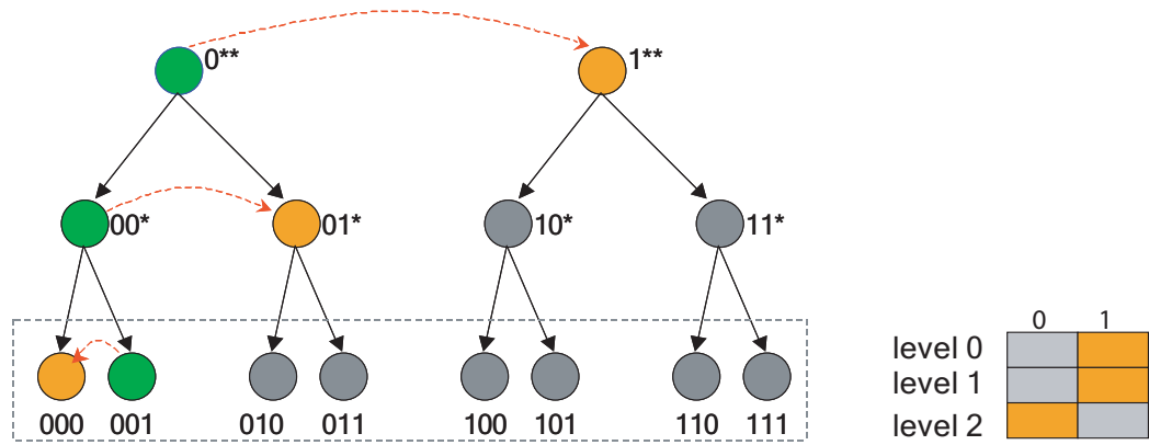
Figure 7.9: Similar to the prefix-based routing method.
