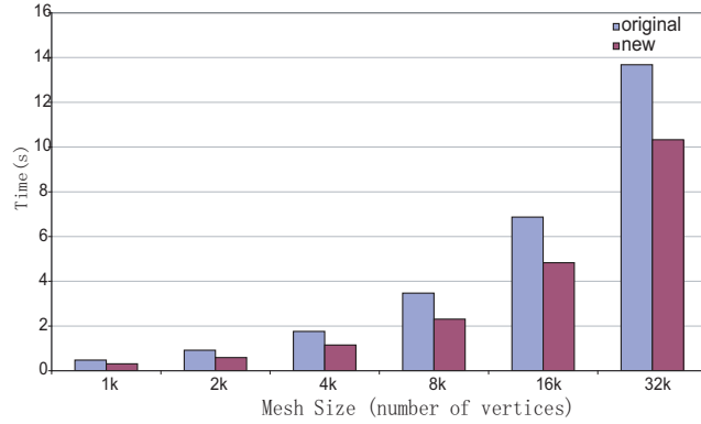
Figure 5.13: CFD kernel on Intel Clovertown with 8 cores.
