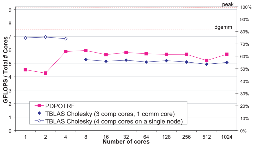
Figure 6.22: Scalability of Cholesky factorization on Cray XT4.
