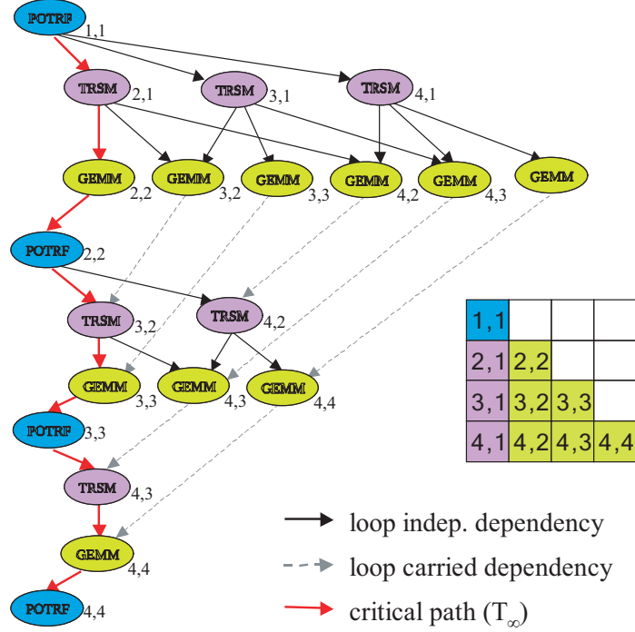
Figure 6.10: DAG for the tiled Cholesky factorization.
