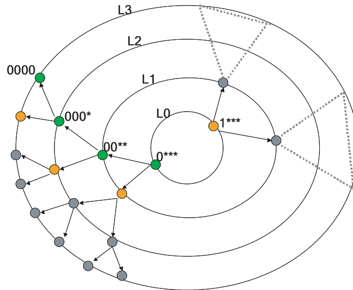
Figure 7.10: Implicit multiple spanning trees.
