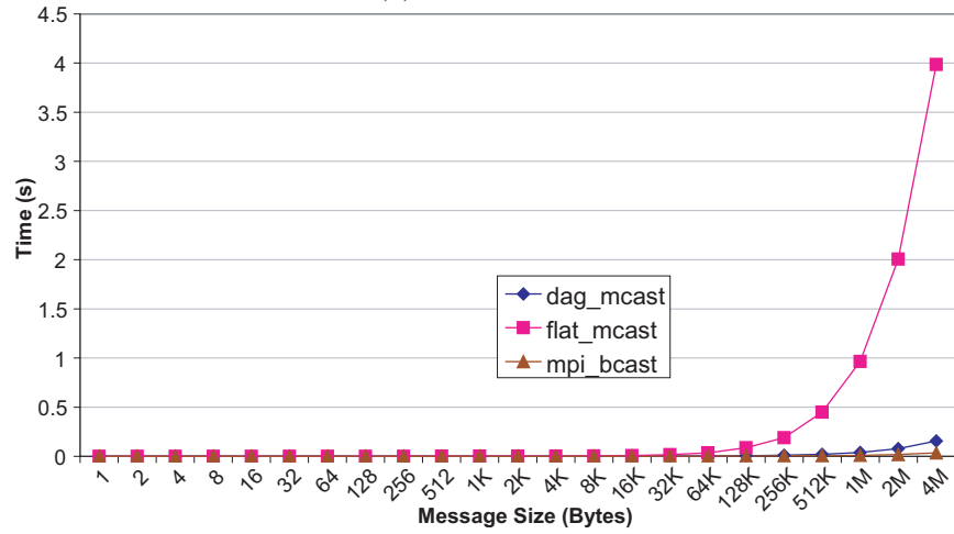
(f) 128 Processes
