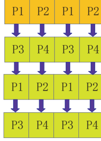
Figure 6.13: Trailing submatrix update in the tiled LU and QR algorithms.
