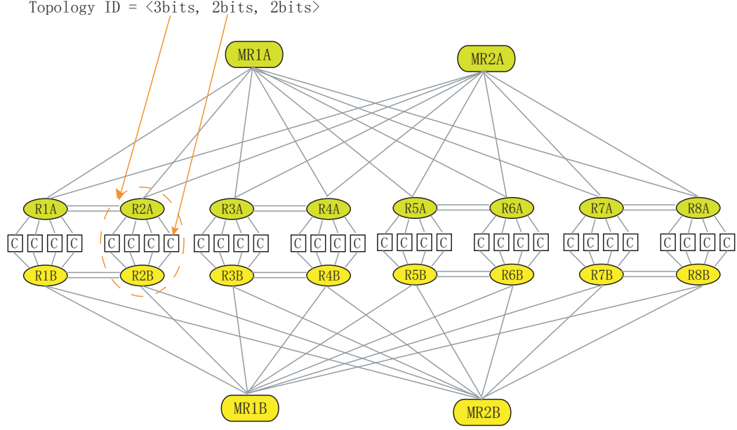
Figure 7.5: An example to assign topology IDs to an SGI Altix 3700 System with 128 processors. C denotes a 4-processor C-brick.
