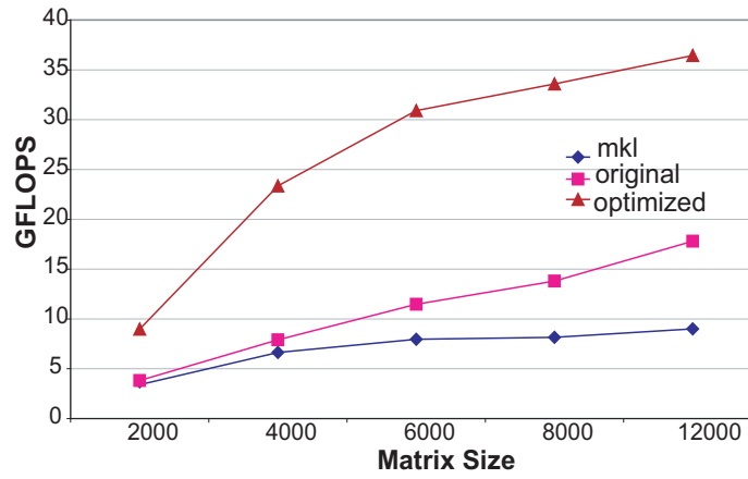
Figure 5.17: Cholesky factorization on SGI Altix with 8 processors.
