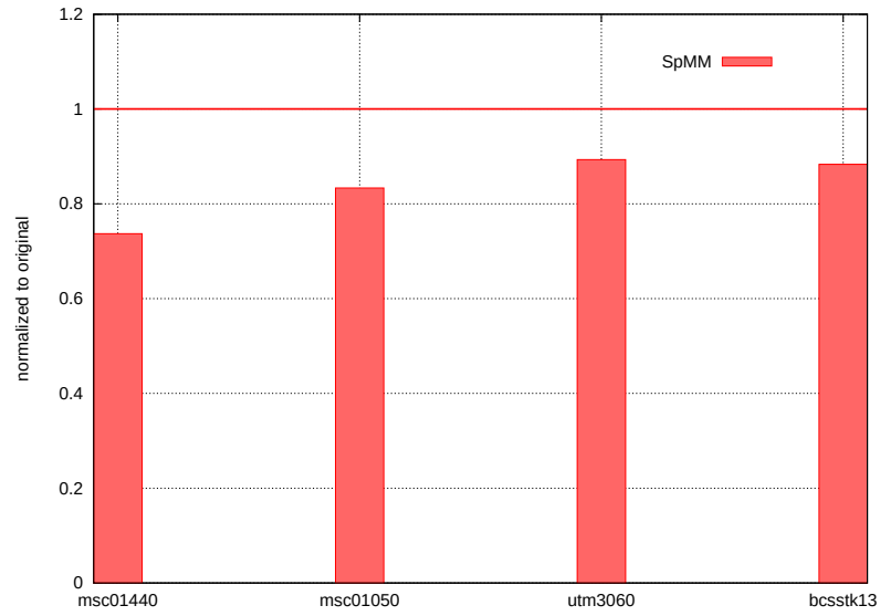
Figure 5.11: SpMM on SGI Altix with 4 processors.
