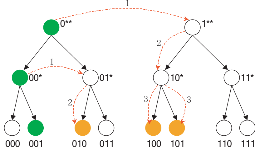
Figure 7.4: Multicast on a system with 8 compute nodes.
