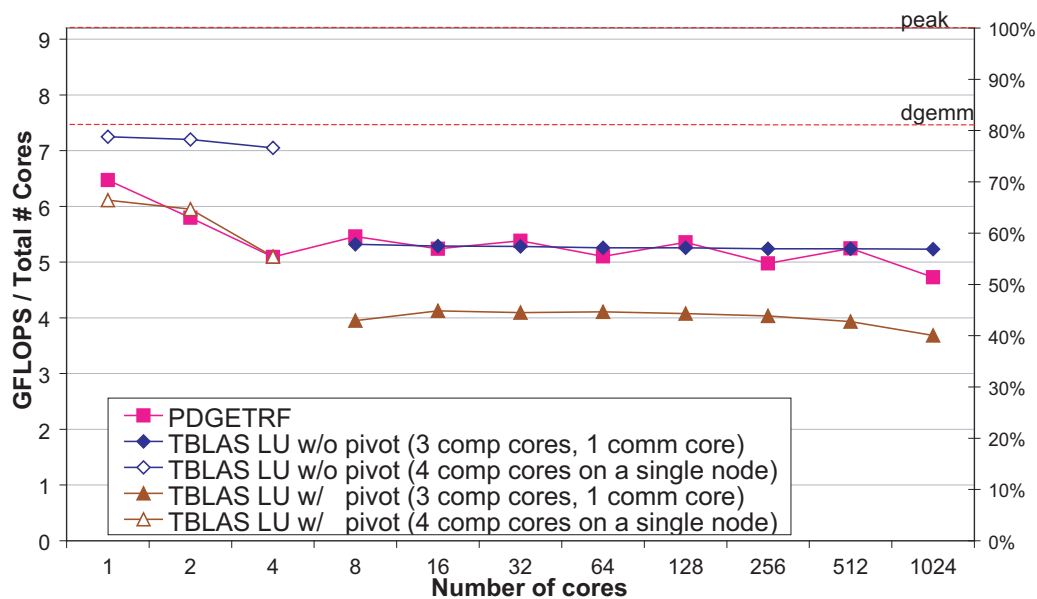
Figure 6.24: Scalability of LU factorization on Cray XT4.
