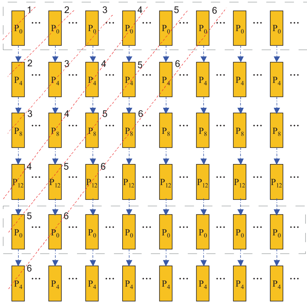
Figure 6.14: Asynchronous pipeline execution by a 4 \times 4 process grid.
