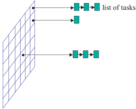
Figure 6.5: Block access list to store tasks in the runtime system.
