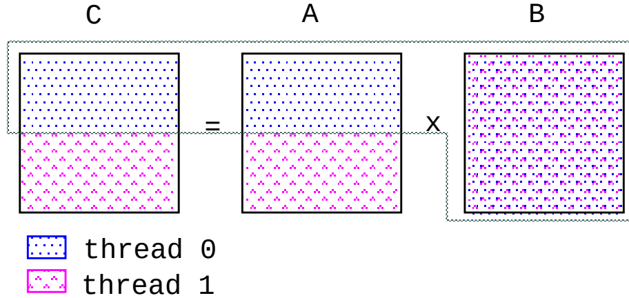
Figure 3.3: Two threads compute matrix multiplication of C = A \times B using the block data distribution. For thread 0, half of its compulsory misses on matrix B could be saved by data loading of thread 1 (i.e., F_{m2h}^{(co)} = \frac{1}{(.5+.5+1) \times 2} = \frac{1}{4} ).
