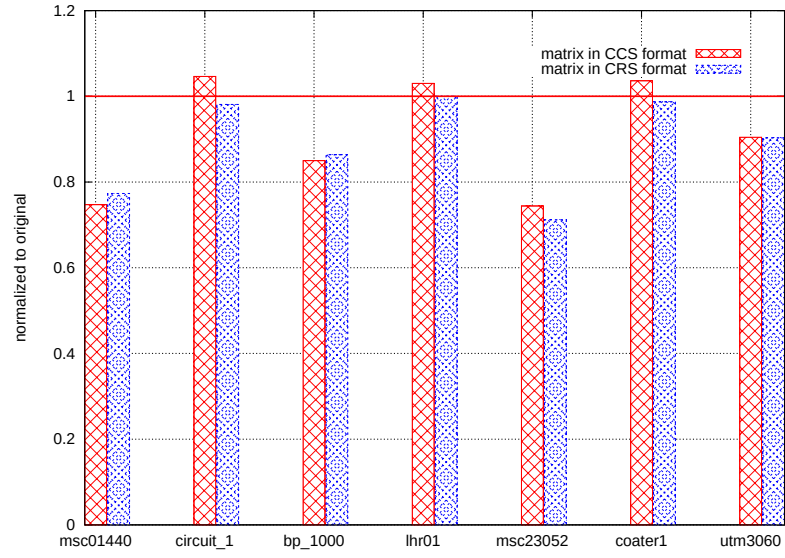
Figure 5.9: SpMV on SGI Altix with 4 processors. Both formats of CCS and CRS are used for each sparse matrix.
