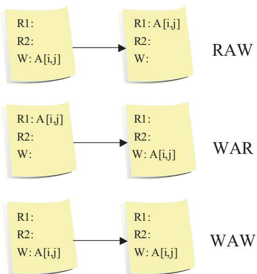
Figure 6.3: Detecting data dependences based on a task list.
