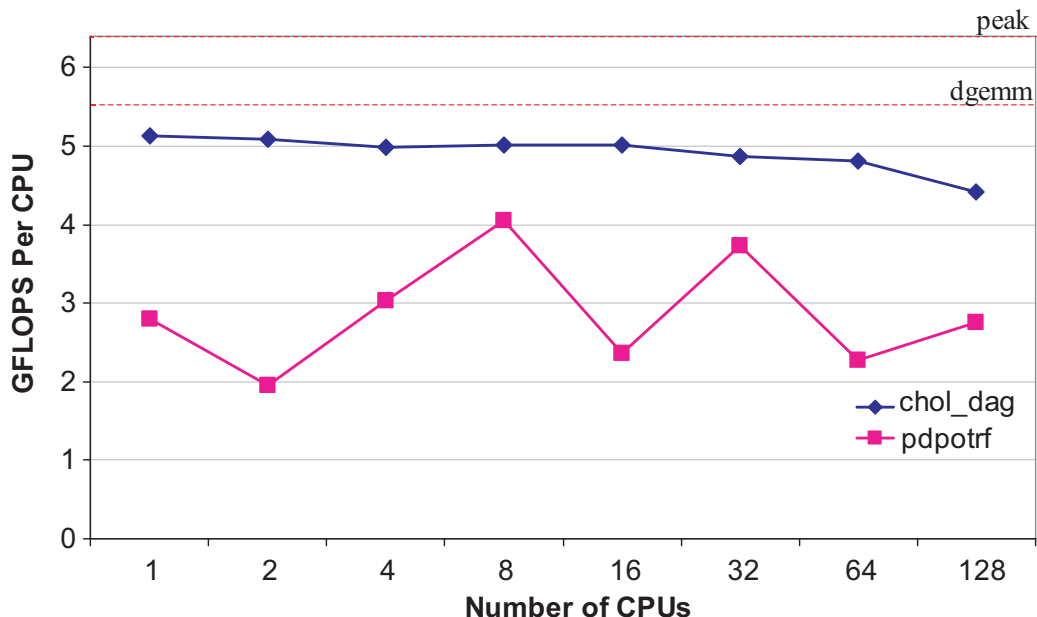
Figure 7.3: Cholesky factorization on a cluster machine.
