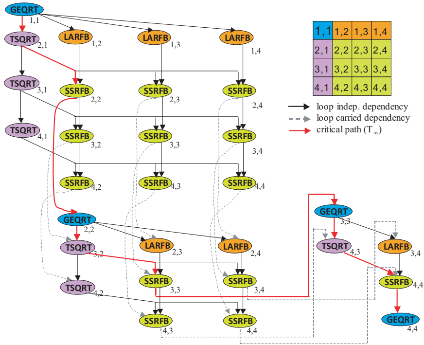
Figure 6.12: DAG for the tiled QR factorization.
