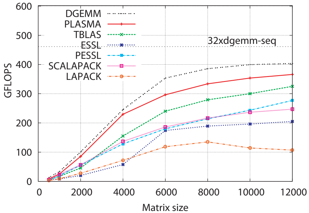
Figure 6.19: Cholesky factorization on a 32-core IBM Power6 machine.
