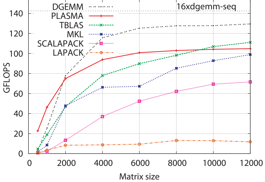
Figure 6.18: QR factorization on a 16-core Intel Tigerton machine.
