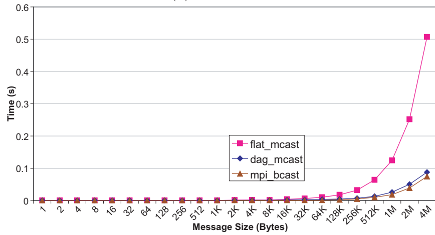
(e) 64 Processes
