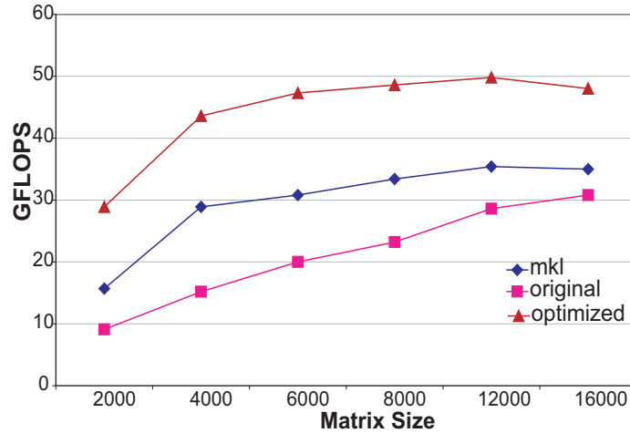
Figure 5.15: Cholesky factorization on Intel Clovertown.
