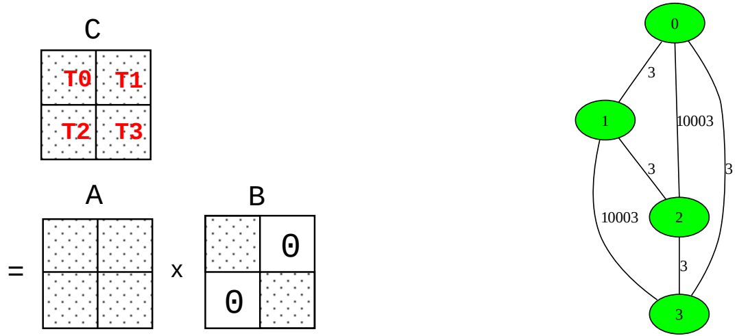
Figure 4.2: An example of affinity graph for matrix multiplication using four threads.
