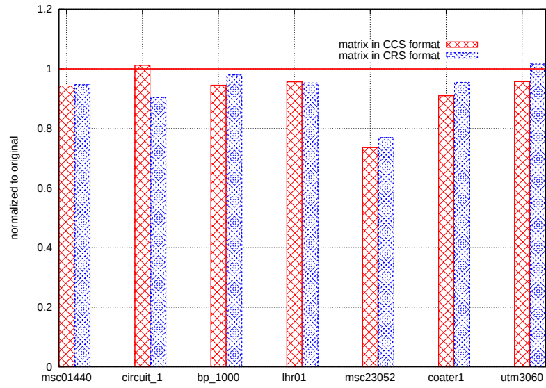
Figure 5.10: SpMV on Intel Clovertown with 8 cores. Both formats of CCS and CRS are used for each sparse matrix.
