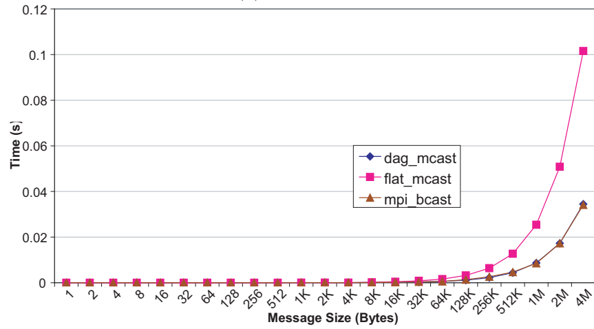
(b) 8 Processes
