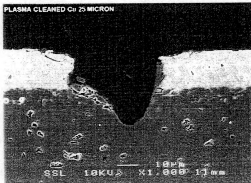
Fig. 24- Secondary electron image of a nominal 25 μm gap attempt in copper.
