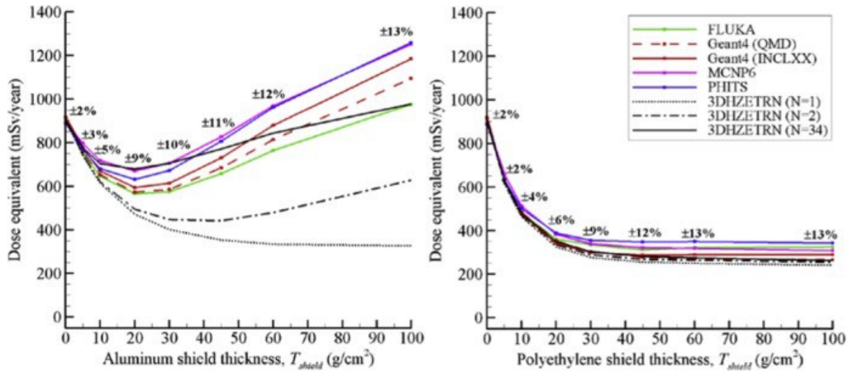
Figure 1. Dose equivalent from neutrons and ions as a function of aluminum (left) and polyethylene (right) shield thickness for the full GCR boundary condition.
