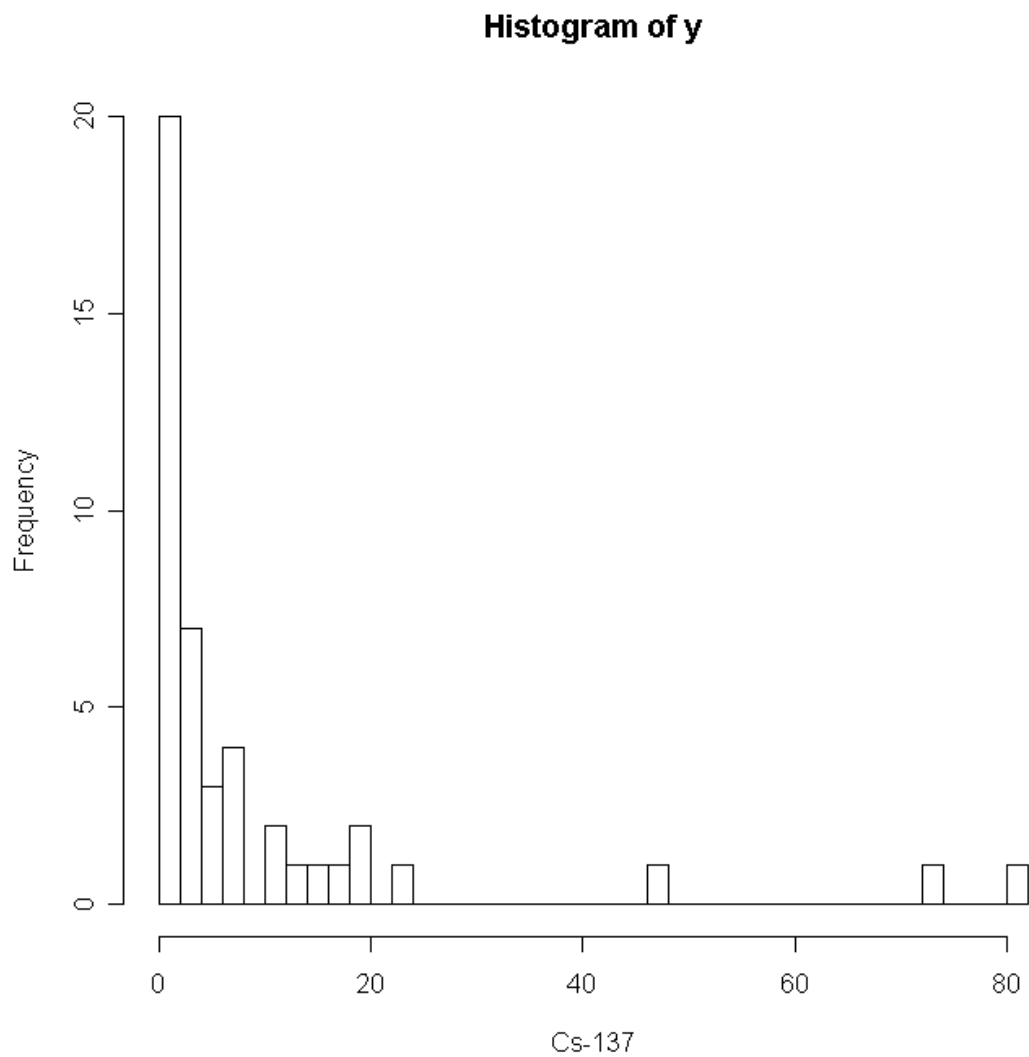
Figure 21 Histogram of FSS data showing Cs-137 concentrations.
