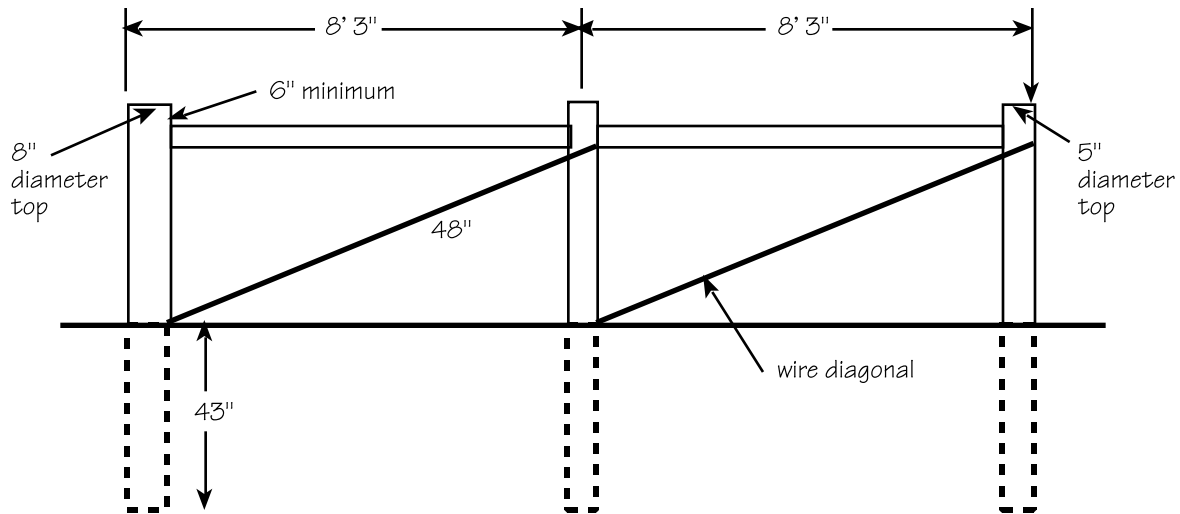
Figure 7. Double Brace assembly
