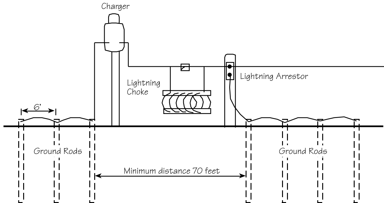
Figure 5. Protecting Electric Fence
