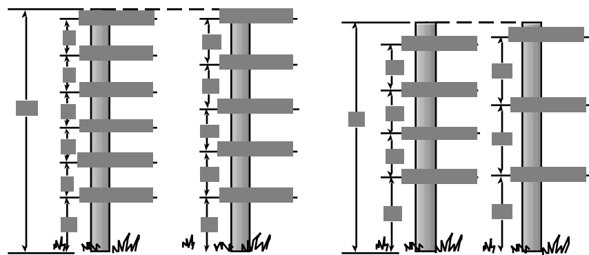
Figure 1. Common Spacings in Barbed Wire Fences
