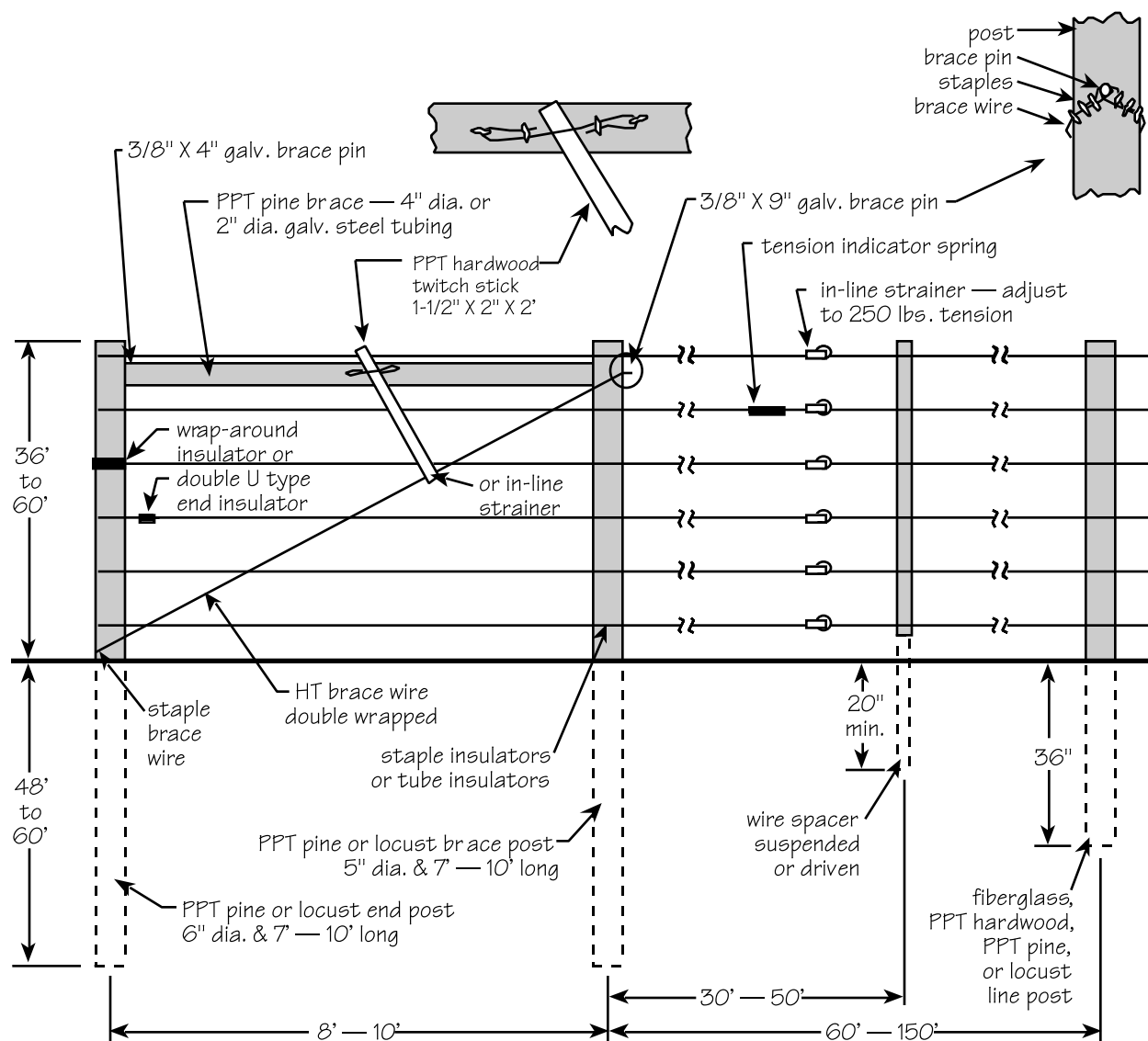
Figure 6. Corner Brace Assembly
