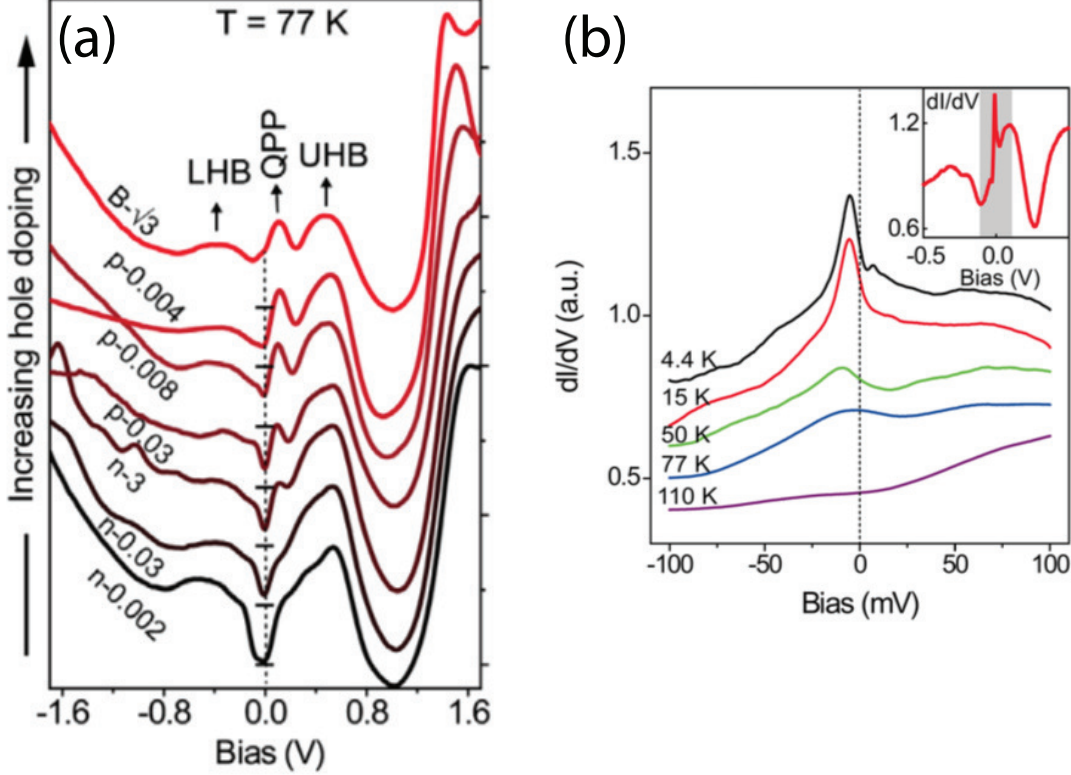
Figure 3.5: (a) \frac{dI}{dV} spectra measured at 77 K for the Si(111)-( \sqrt{3} \times \sqrt{3} ) R30°-Sn system grown on different substrates with different doping levels. (b) High resolution \frac{dI}{dV} spectra taken at various temperatures on the most heavily hole-doped surface, revealing a Van Hove Singularity at -6 meV.
