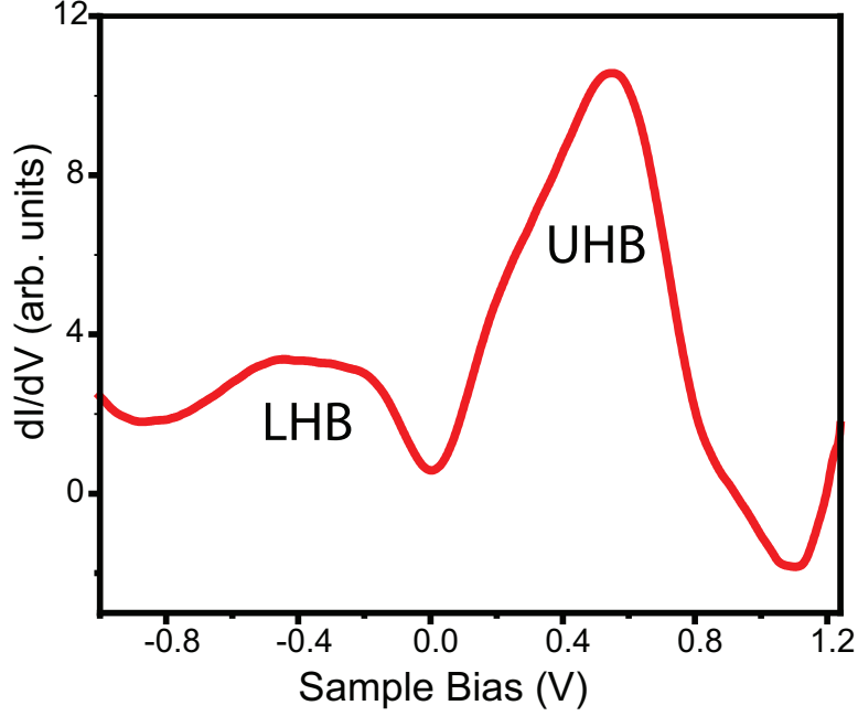
Figure 3.2: STS spectra taken on the undoped \text{Si}(111)-(\sqrt{3} \times \sqrt{3}) \text{R}30^\circ\text{-Sn} surface at 77 K.
