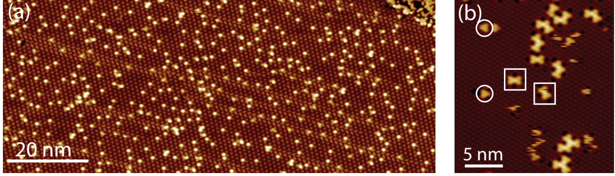
Figure 3.10: (a) STM topography image on the 2\sqrt{3} -HC domain on a heavily doped p-type surface with \Theta_K=.008 ML of potassium measured at 4 K. The adsorbed K atoms appear as bright single-point defects. (b) STM image on the same surface as (a) in a neighboring (\sqrt{3} \times \sqrt{3}) domain. K atoms appear as bright trimers in their simplest form (circled). Adjacent trimers appear as bowties (boxes). The areal density of the single points in (a) equal the trimer density in (b).
