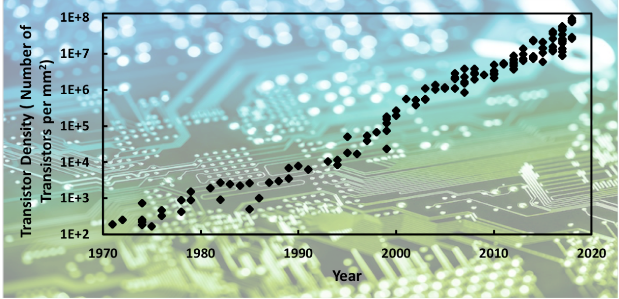
Figure 1.1: Log plot of transistor density for integrated circuits over time, exemplifying Moore’s law in action, defined by a doubling every two years. Data taken from Wikipedia (2020) .
