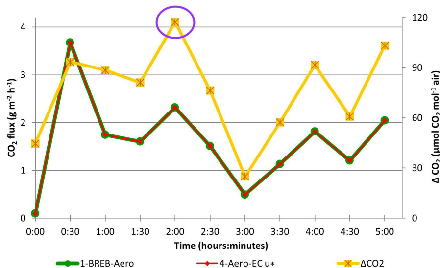
Fig. 4. Half-hour \text{CO}_2 flux for the BREB-Aero (Method 1) and Aero-EC u^* (Method 4) from 0000 to 0500 h on 17 June 2017 with 30-min average \text{CO}_2 concentration differences between lower and upper sensor at the SMB BREB station. The purple circle indicates the maximum \text{CO}_2 concentration difference of 117 \mu\text{mol CO}_2 \text{ mol}^{-1} \text{ air} during this period.
