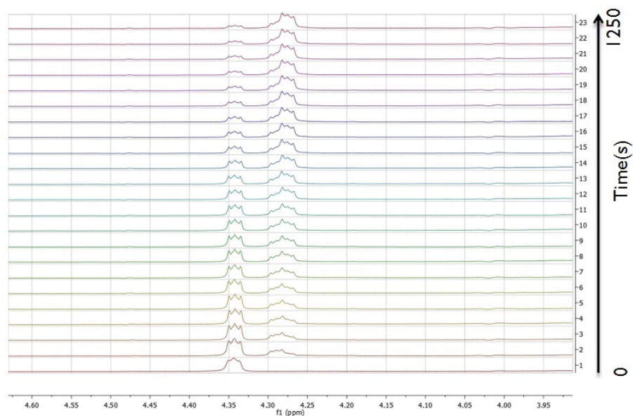
Figure 24: Stacked 1 H-NMR spectra for PEG-TECC reaction at 21 0 C showing thiol intensity drop and appearance of amine peak.
