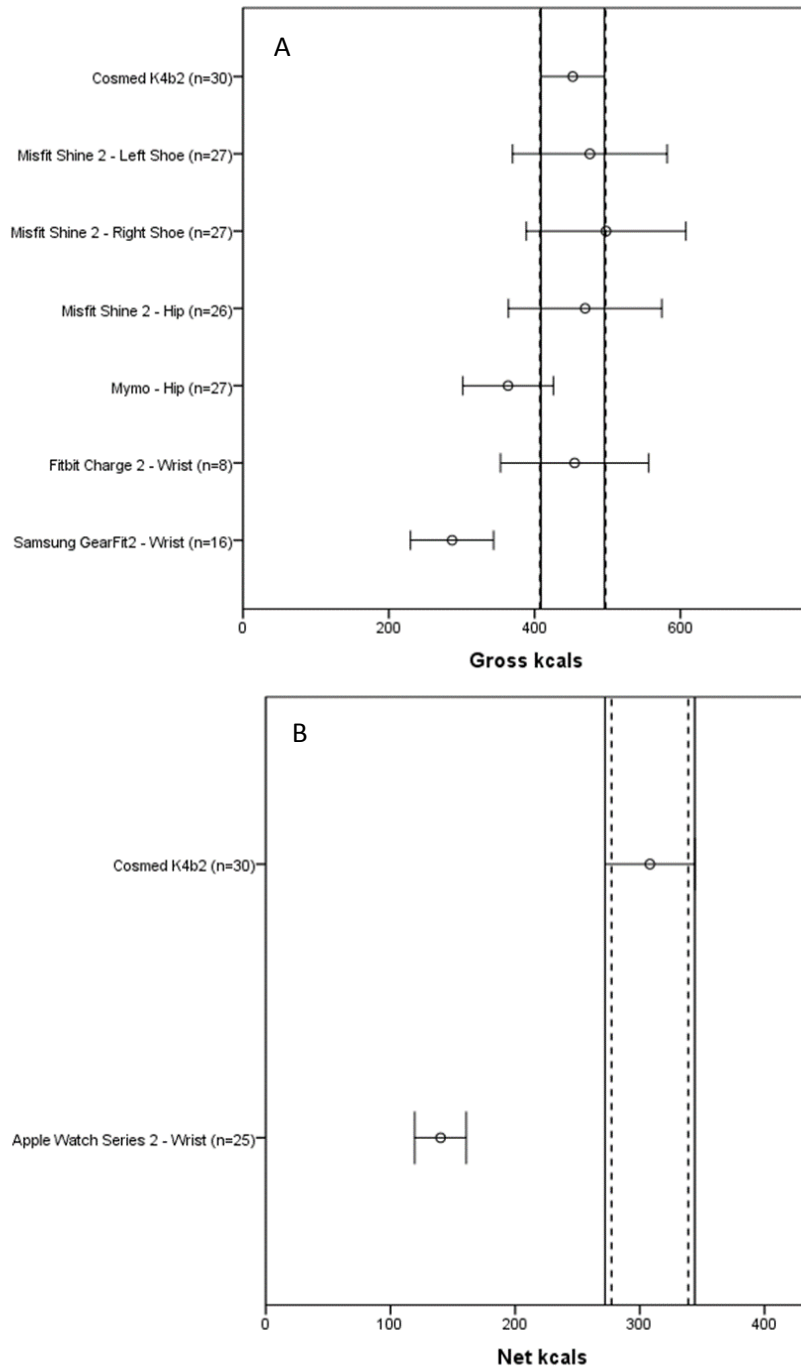
Figure 2. Agreement between the Cosmed K4b 2 and A) consumer monitors that provide estimates of gross EE and B) consumer monitors that provide estimates of net EE for participants aged 13-18 years. Dark vertical lines indicate the equivalence zone from the Cosmed K4b 2 . Dotted vertical lines indicate \pm 10\% of the mean measured EE of the Cosmed K4b 2 .
