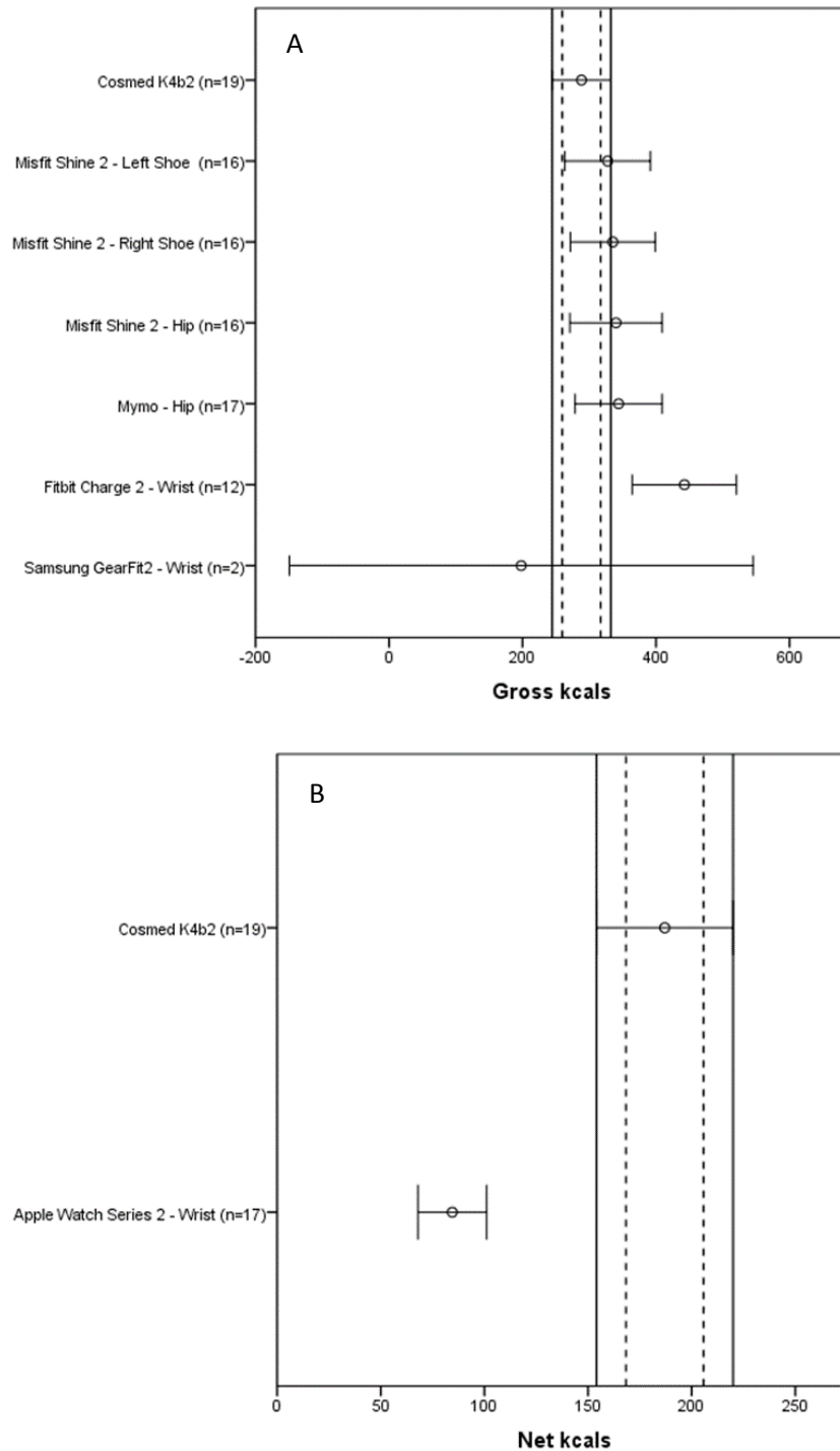
Figure 1. Agreement between the Cosmed K4b 2 and A) consumer monitors that provide estimates of gross EE and B) consumer monitors that provide estimates of net EE for participants aged 6-12 years. Dark vertical lines indicate the equivalence zone from the Cosmed K4b 2 . Dotted vertical lines indicate \pm 10\% of the mean measured EE of the Cosmed K4b 2 .
