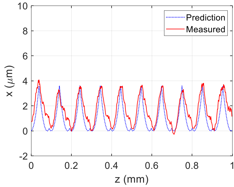
Figure A.10: Surface profile comparison for test point O31432, where the measured MTP parameters were RAF = 0.7 , OPR = 0.5 .
