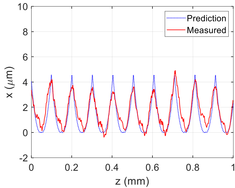
Figure 6.26: Surface profile comparison for test point O31422, repeat testing location at jaw 3. The measured MTP parameters were RAF = 0.6 , OPR = 0.5 .
