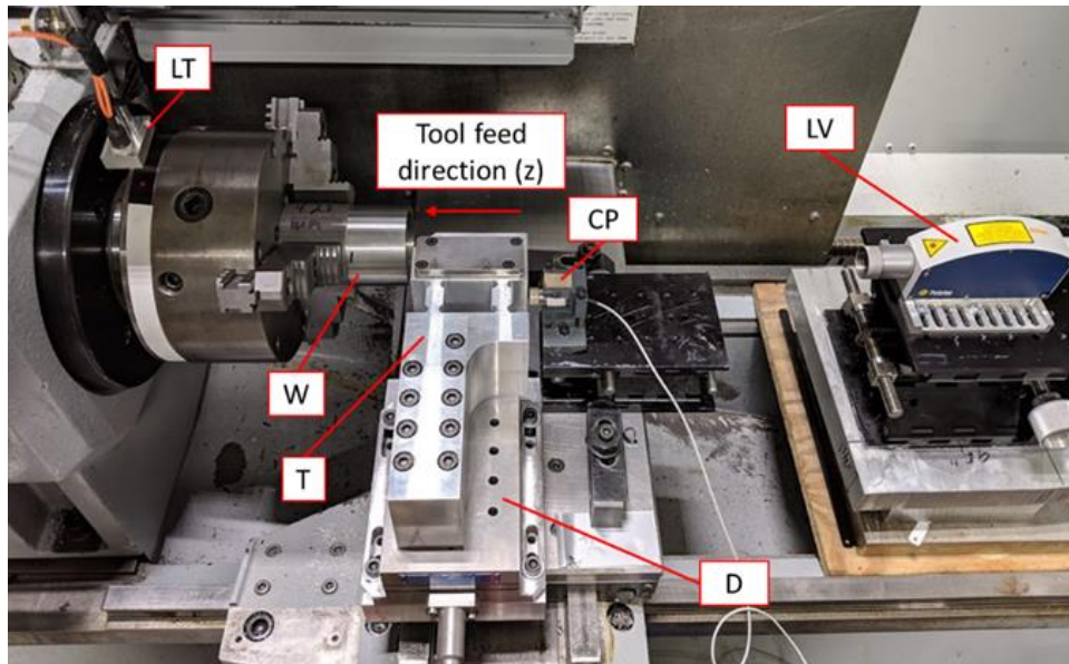
Figure 5.1: Photograph of tube turning setup including workpiece (W), dynamometer (D), flexure-based cutting tool (T), laser tachometer (LT), laser vibrometer (LV), and capacitance probe (CP).
