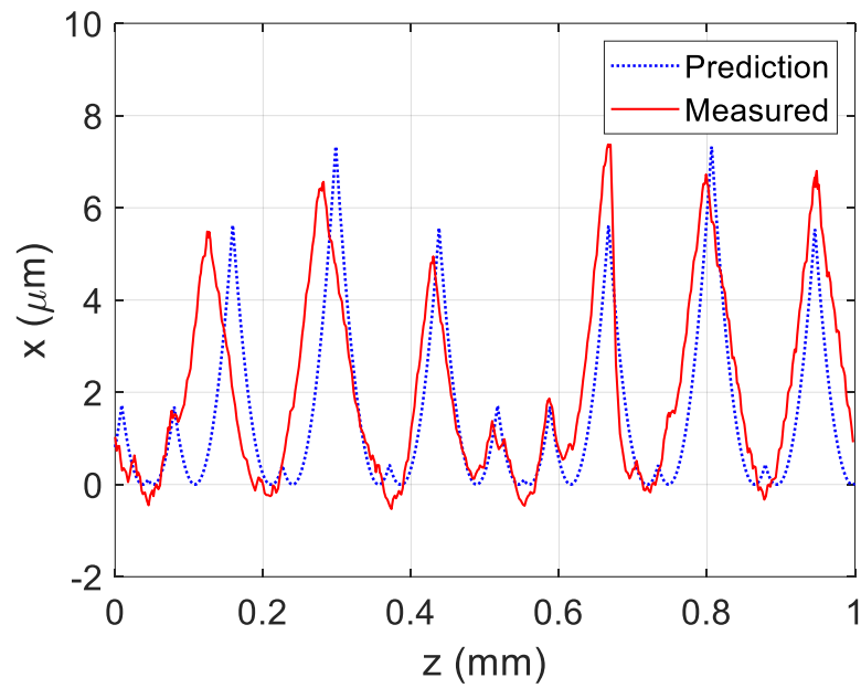
Figure A.2: Surface profile comparison for test point O31242, where the measured MTP parameters were RAF = 0.8 , OPR = 0.3 .
