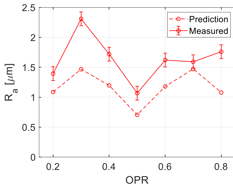
Figure 6.25: Arithmetic mean surface roughness ( R_a ) value as OPR is varied. Plotted error bars represent one standard deviation.
