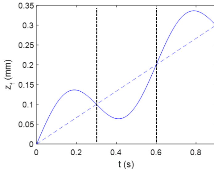
Figure 3.2: MTP feed motion for three spindle revolutions. The spindle speed is 200 rpm, the feed per revolution is 0.1 mm/rev, and the OPR and RAF values are 0.5 and 0.8. The dashed positive slope line identifies the constant feed contribution to the motion, while the solid line shows its sum with the sinusoidal MTP contribution. The vertical dotted lines denote each revolution.
