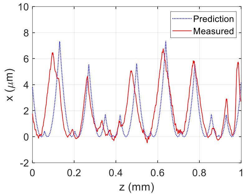
Figure 6.23: Surface profile comparison for test point O31242, repeat testing location at jaw 2. The measured MTP parameters were RAF = 0.8 , OPR = 0.3 .
