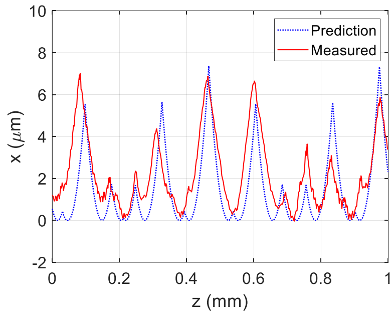
Figure 6.24: Surface profile comparison for test point O31242, repeat testing location at jaw 3. The measured MTP parameters were RAF = 0.8 , OPR = 0.3 .
