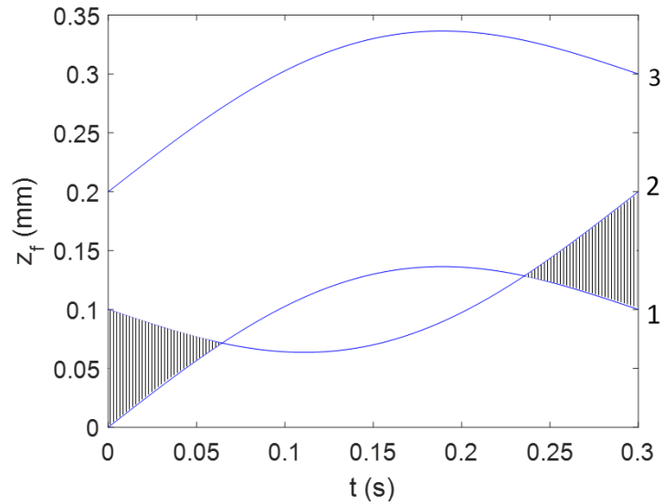
Figure 3.3: Chip thickness calculation for revolution 2. The nonzero chip thickness zones are denoted by the hatched areas.
