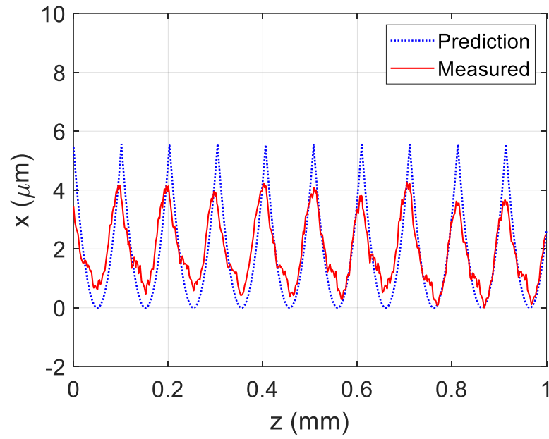
Figure A.8: Surface profile comparison for test point O31412, where the measured MTP parameters were RAF = 0.5 , OPR = 0.5 .
