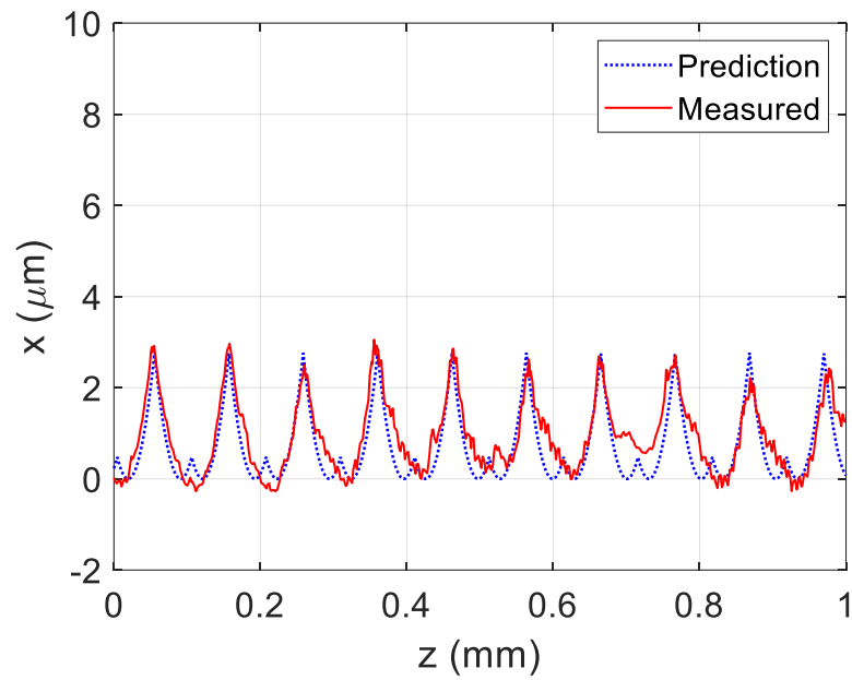
Figure A.4: Surface profile comparison for test point O31442, where the measured MTP parameters were RAF = 0.8 , OPR = 0.5 .
