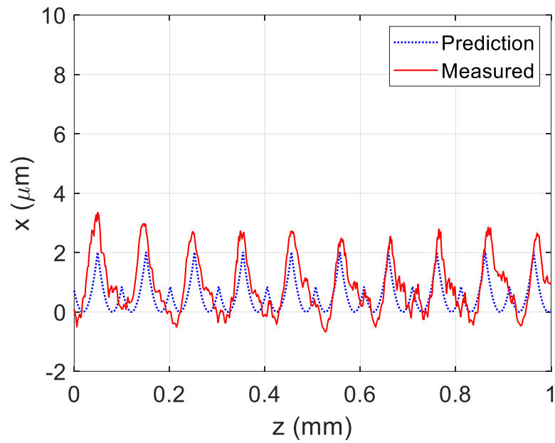
Figure A.12: Surface profile comparison for test point O31452, where the measured MTP parameters were RAF = 0.9 , OPR = 0.5 .
