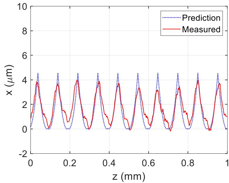
Figure 6.28: Surface profile comparison for test point O31422, repeat testing location at jaw 3. The measured MTP parameters were RAF = 0.6 , OPR = 0.5 .
