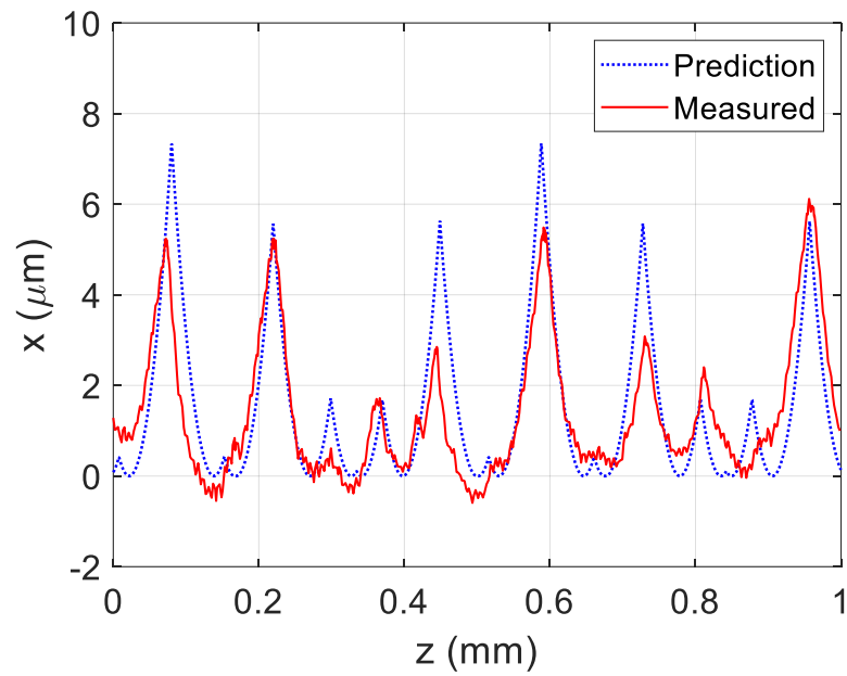
Figure A.6: Surface profile comparison for test point O31642, where the measured MTP parameters were RAF = 0.8 , OPR = 0.7 .
