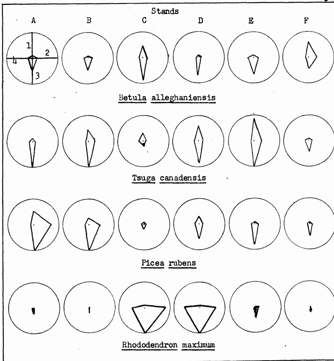
Figure 8. Phytographs showing growth patterns of major woody species in six stands in study area. Radius 1, percentage of total basal area; Radius 2, percentage of total stems; Radius 3, percentage frequency; Radius 4, percentage of total woody stem reproduction.
