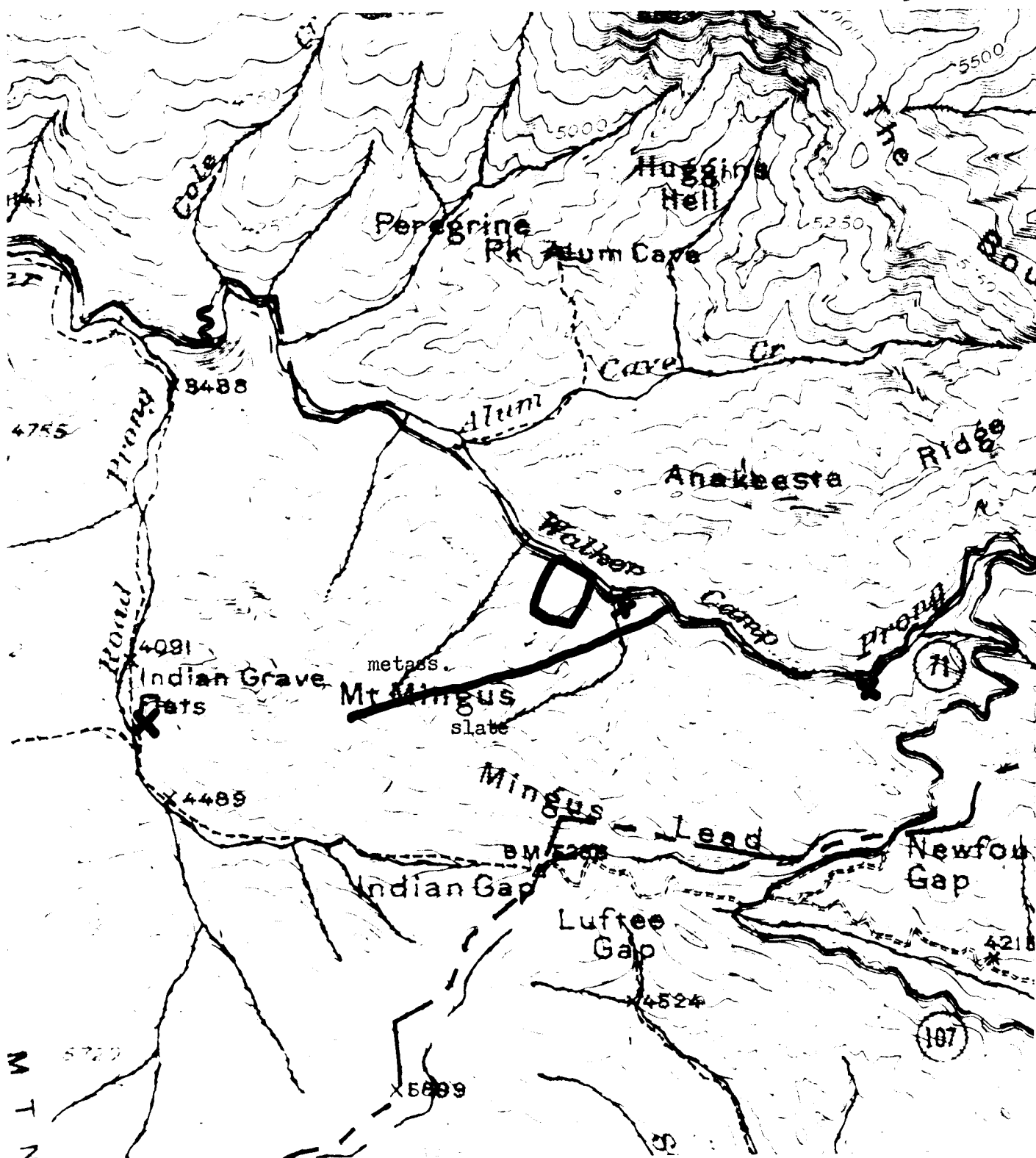
Figure 1. Contour map of north portion of Clingmans Dome 7 \frac{1}{2} " Quadrangle outlining location of study area; location of isolated low altitude Abies fraseri , X; and geologic position of metasandstone and slate formations.
