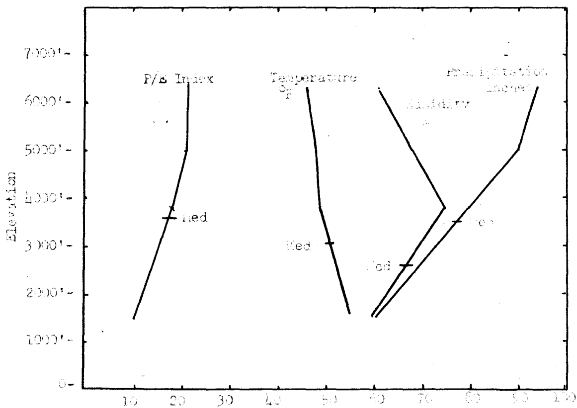
Figure 4. Graph showing average monthly P/E index, temperature, per cent of days humidity was over 90 per cent, and precipitation from January 1948 to June 30, 1950.
