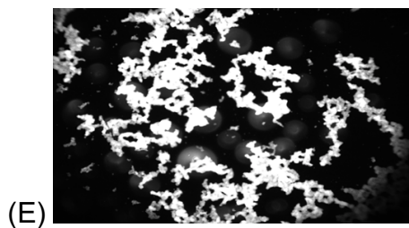
Figure 3 Image A and represents a negative agglutination score. Image B represents a 1+ agglutination score. Images C represents a 2+ agglutination score. Image D represents a 3+ agglutination score. Image E represents a 4+ agglutination score.
