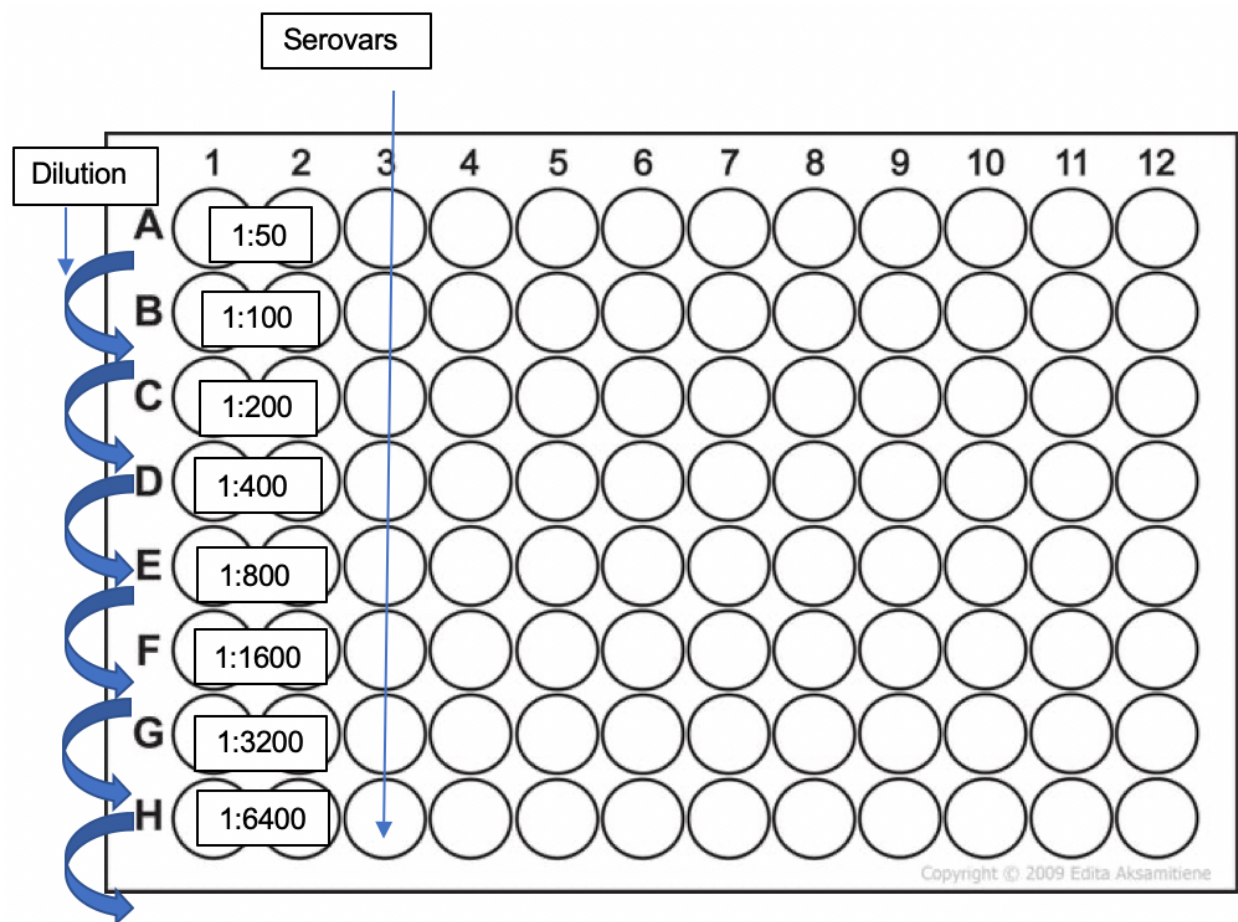
Figure 4 Microscopic Agglutination Test (MAT) titration plate layout. Serial dilution of patient serum performed vertically, then 50 \mu L of the respective standardized culture is added to each well.
