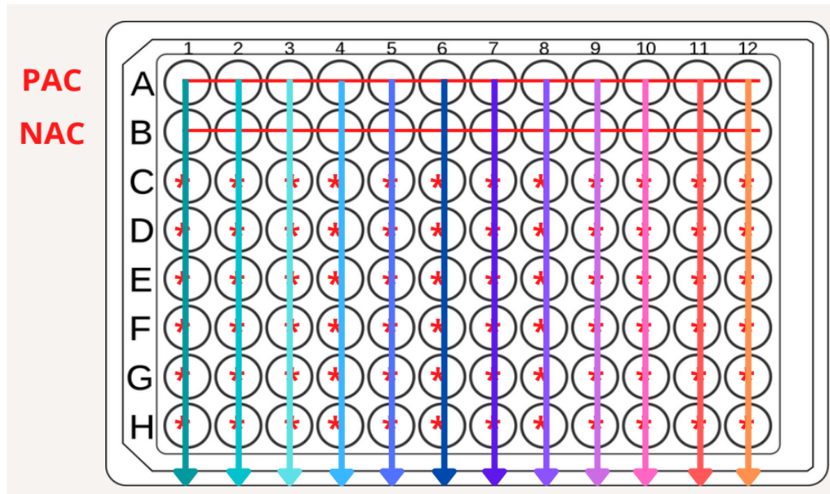
Figure 2 Microscopic Agglutination Test (MAT) plate layout for screening. PAC is the positive control (homologous rabbit antisera), NAC is the negative control (phosphate buffered saline). Diluted patient serum goes horizontally down rows C, D, E, F, G, and H, and the standardized culture goes down each column (1-Autumnalis, 2-Ballum, etc.).
